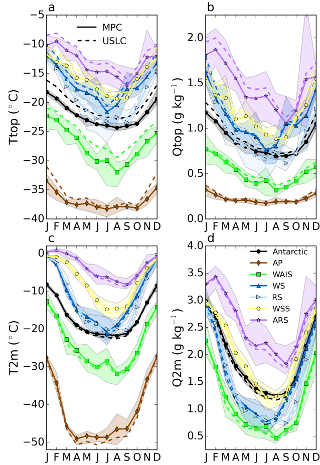
Figure 11. Top row: monthly time series of (a) the in-cloud Temperature ( T_{top} ), and of (b) the in-cloud water vapour mixing ratio ( Q_{top} ), at the top of the low-level MPC and USLC layers, for the different regions of interest. Bottom row: near-surface (two-meters) temperature (c) and water vapour mass mixing ratio (d) below these layers. The shaded areas indicate the interannual variability for the MPC layers. For readability, the ones for the USLC layers are not shown, but they are of similar amplitude.
