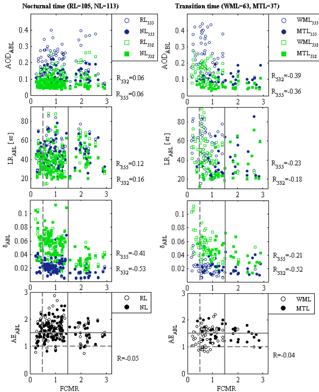
Figure 7. Hourly averaged aerosol optical depth (AOD), lidar ratio (LR), linear particle depolarization ratio ( \delta ) and Ångström exponent ( \text{\AA E} ) derived within atmospheric boundary layer at 355 and 532 nm of PollyXT lidar at the EARLINET/ACTRIS site of RS-Lab in Warsaw for July-September of 2013, 2015, 2016 versus surface fine to coarse mass ratio (FCMR) derived from particulate matter ( \text{PM}_{2.5} and \text{PM}_{10} ) measured at the WIOS site in Warsaw-Ursynow. Thresholds of \text{\AA E} and FCMR are marked as horizontal and vertical lines, respectively.
