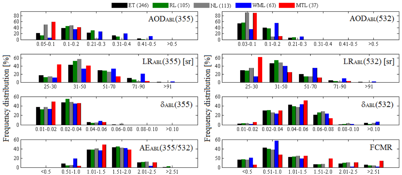
5 Figure 2. Frequency distribution of aerosol optical depth (AOD), lidar ratio (LR), linear particle depolarization ratio ( \delta ) and Ångström exponent ( \text{ÅE} ) at 355 and 532 nm derived within atmospheric boundary layer at the EARLINET/ACTRIS lidar site in Warsaw for period of July-September 2013, 2015, 2016. Corresponding fine to coarse mass ratio (FCMR) derived from measurements of surface particulate matter with an aerodynamic diameter below 10\mu\text{m} ( \text{PM}_{10} ) and below 2.5\mu\text{m} ( \text{PM}_{2.5} ) at the WIOS site in Warsaw-Ursynow. The period of measurement is divided to the entire time (ET; 24 h), the nocturnal time (NT; 22:00-2:00 UTC, including the residual boundary layer RL and the nocturnal boundary layer NL), and the transition time (TT; after sunrise at 03:00-8:00 for the morning transition layer MTL and before sunset at 16:00-20:00 UTC for the well-mixed boundary layer WML). 10
