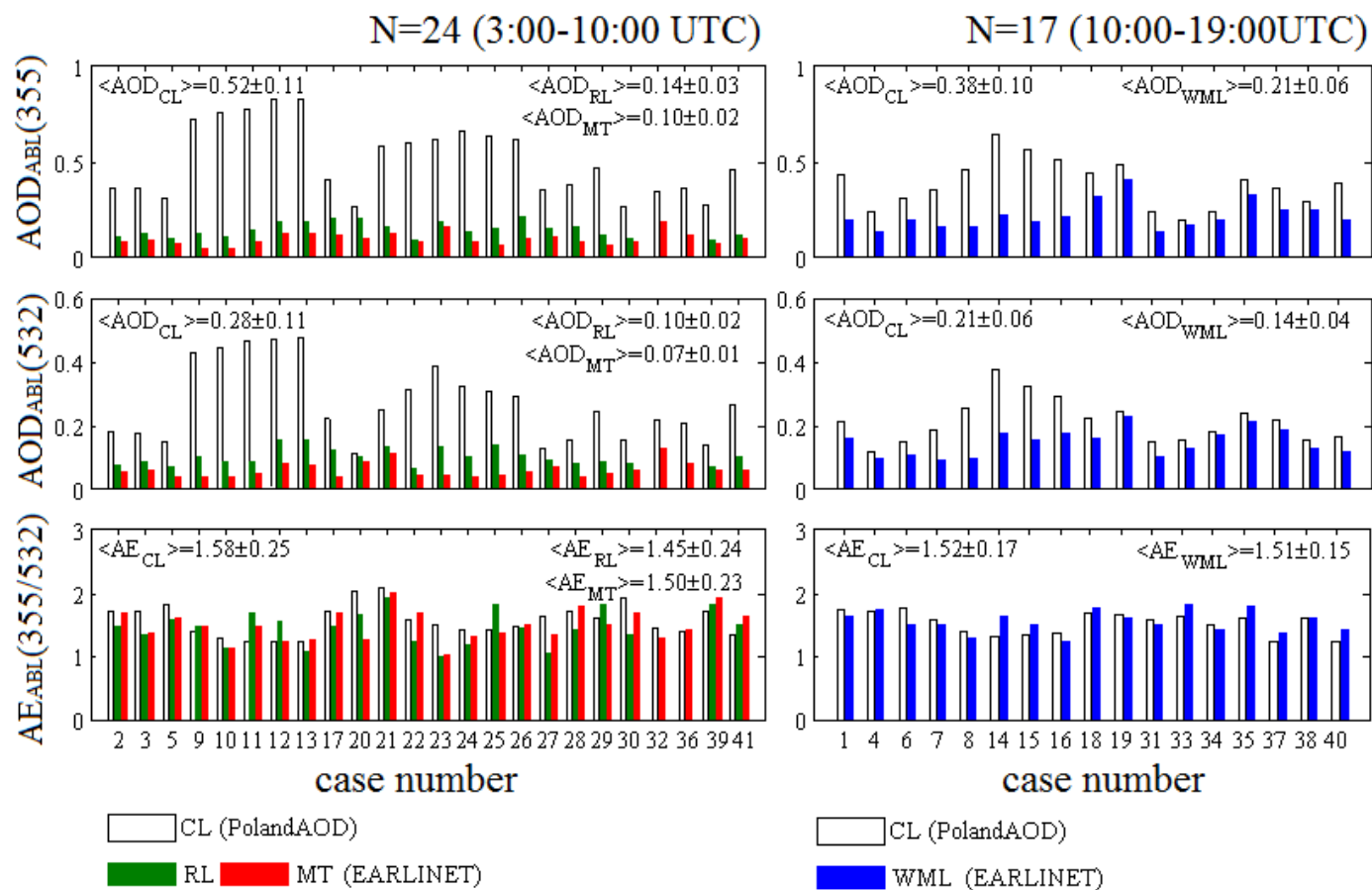
Figure 4. Hourly averages of aerosol optical depth (AOD) and Ångström exponent (ÅE) derived within the atmospheric boundary layer at 355 and 532 nm from PollyXT lidar at the EARLINET/ACTRIS site in Warsaw plotted along with the corresponding MFR-7 shadowband radiometer at the PolandAOD-NET site in Warsaw for July-September 2013, 2015, 2016 (leap year). Those were collocated measurements at the RS-Lab in Warsaw. AOD CL of MFR-7 measurements at 415 and 500 nm were scaled to 355 and 532 nm using Ångström law.
