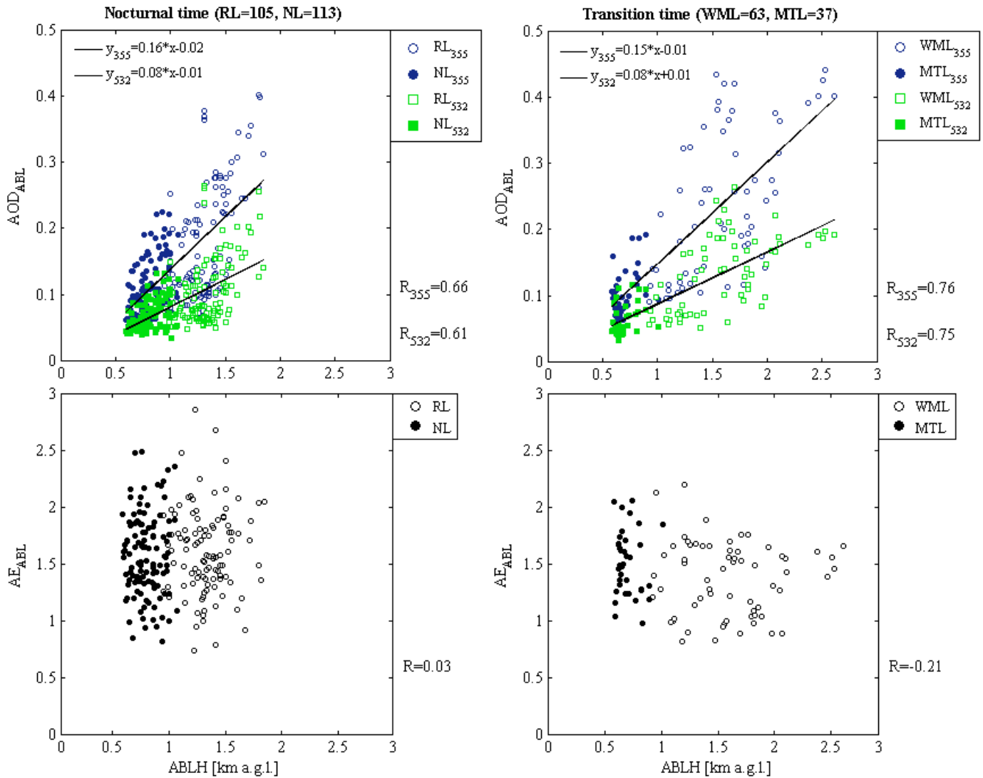
5 Figure 5. Hourly averaged aerosol optical depth (AOD) and Ångström exponent (ÅE) derived within boundary layer at 355 and 532 nm versus atmospheric boundary layer height (ABLH), all derived from PollyXT lidar at the EARLINET/ACTRIS site of RS-Lab in Warsaw for July-September of 2013, 2015, 2016. Linear fit to data points is shown for correlation coefficients R > 0.6 .
