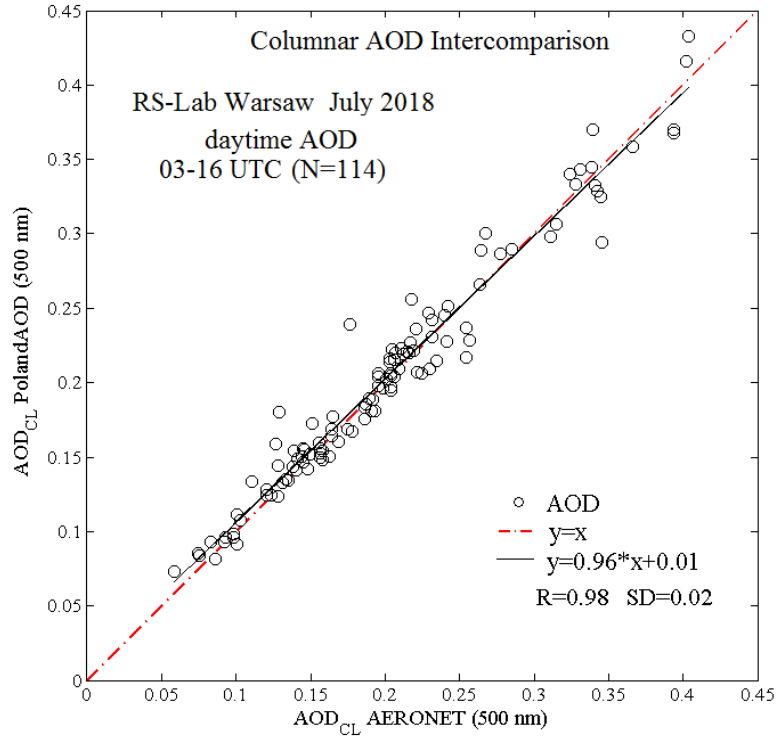
Figure 3. Intercomparison of hourly averaged clear-sky daytime aerosol optical depth measured within the atmospheric column( AOD_{CL} ) with CE318 at the AERONET site (Level 2.0 data) and the MFR-7 shadowband radiometer at the PolandAOD-NET site (Level 1.5 data) show high agreement for a month of collocated measurements at the RS-Lab in Warsaw.
