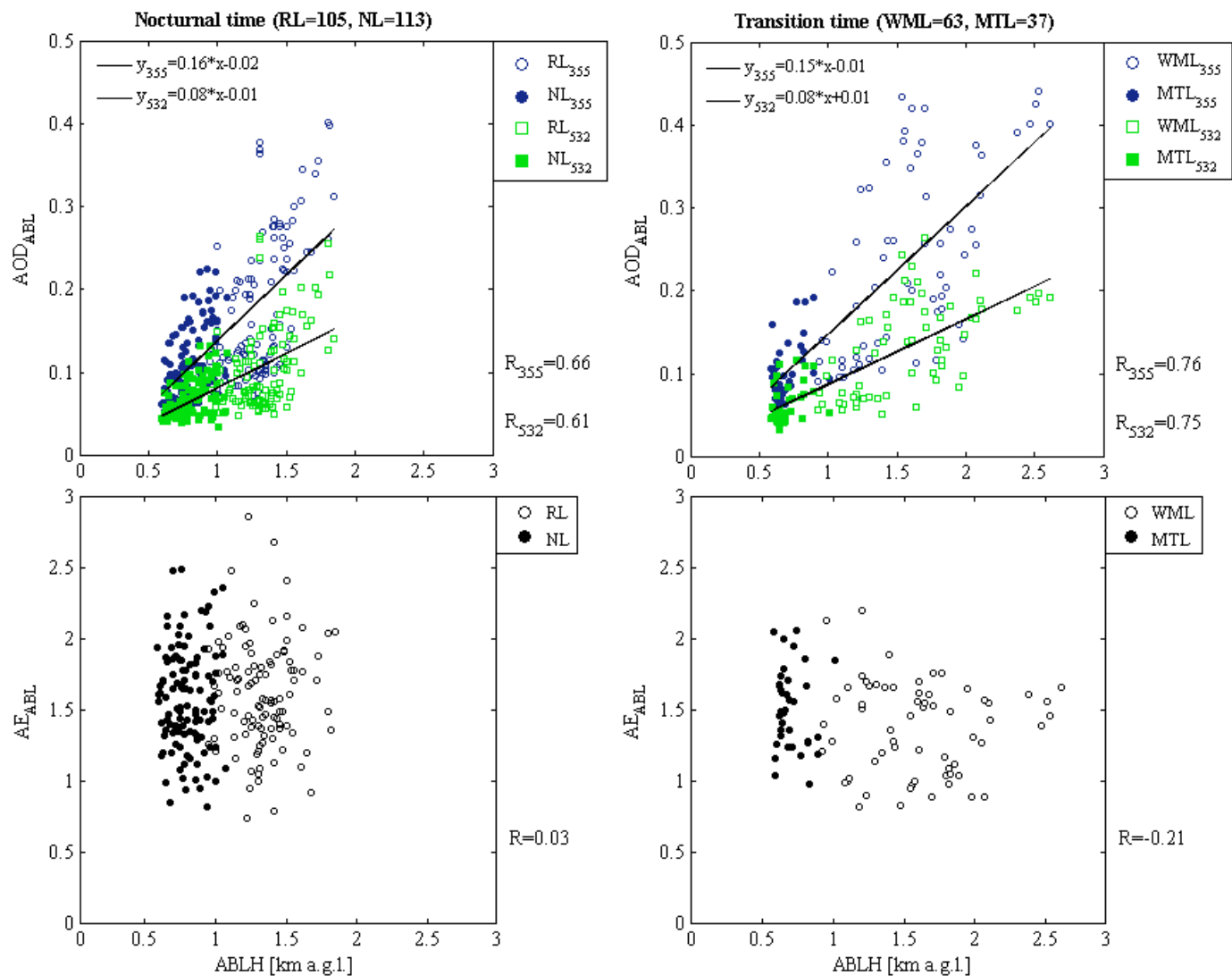
Figure 6. Comparison of hourly averaged aerosol optical depth (AOD) and Ångström exponent (ÅE) derived within boundary layer at 355 and 532 nm against aerosol boundary layer height (ABLH) derived from PollyXT lidar at the EARLINET site in Warsaw in period of July-September of 2013, 2015, 2016. Linear fit to data points is shown for correlation coefficients R > 0.6 .
