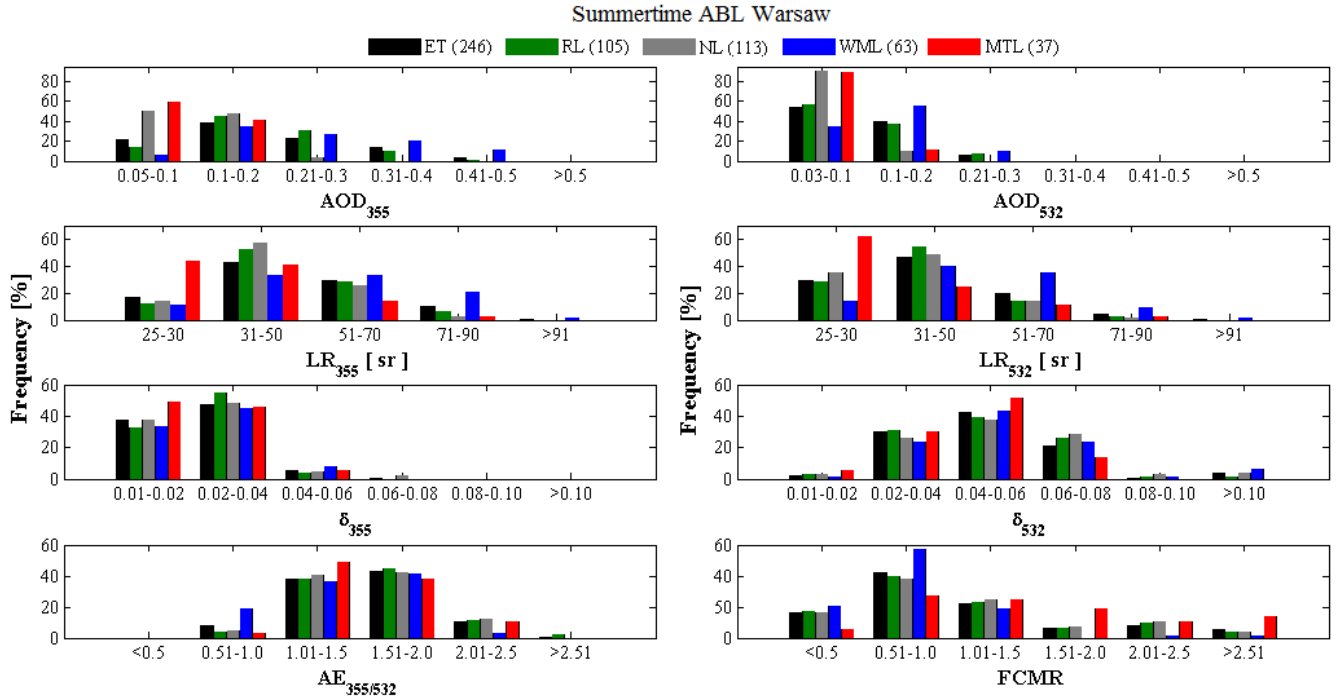
Figure 2. Frequency distribution of aerosol optical depth (AOD), lidar ratio (LR), particle linear depolarization ratio ( \delta ) and Ångstrom exponent ( \text{\AA E} ) at 355 and 532 nm, derived within aerosol boundary layer at the EARLINET lidar site in Warsaw for period of July-September 2013, 2015, 2016 with corresponding fine to coarse mass ratio (FCMR) derived from surface particulate matter with an aerodynamic diameter below 10\mu\text{m} ( \text{PM}_{10} ) and below 2.5\mu\text{m} ( \text{PM}_{2.5} ) measurements at the WIOS site in Warsaw-Ursynow. The period of measurement is divided to the entire time (ET; 24 h), the nocturnal time (NT; 22:00-2:00 UTC, including the residual boundary layer RL and nocturnal boundary layer NL) and the transition time (TT; after sunrise at 03:00-8:00 for morning transition layer MTL and before sunset at 16:00-20:00 UTC for well-mixed boundary layer WML).
