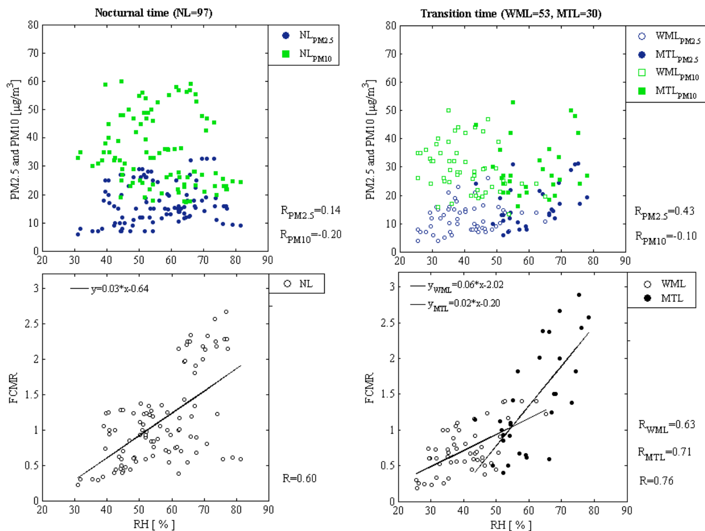
Figure 9. Hourly averaged near-surface relative humidity (RH) measured by the weather transmitter WXT510 (Vaisala) at RS-Lab in Warsaw for period of July-September of 2013, 2015, 2016 versus surface particulate matter PM 2.5 and PM 10 measured at the WIOS site in Warsaw-Ursynow. Linear fit to data points is shown for correlation coefficients R > 0.6 .
