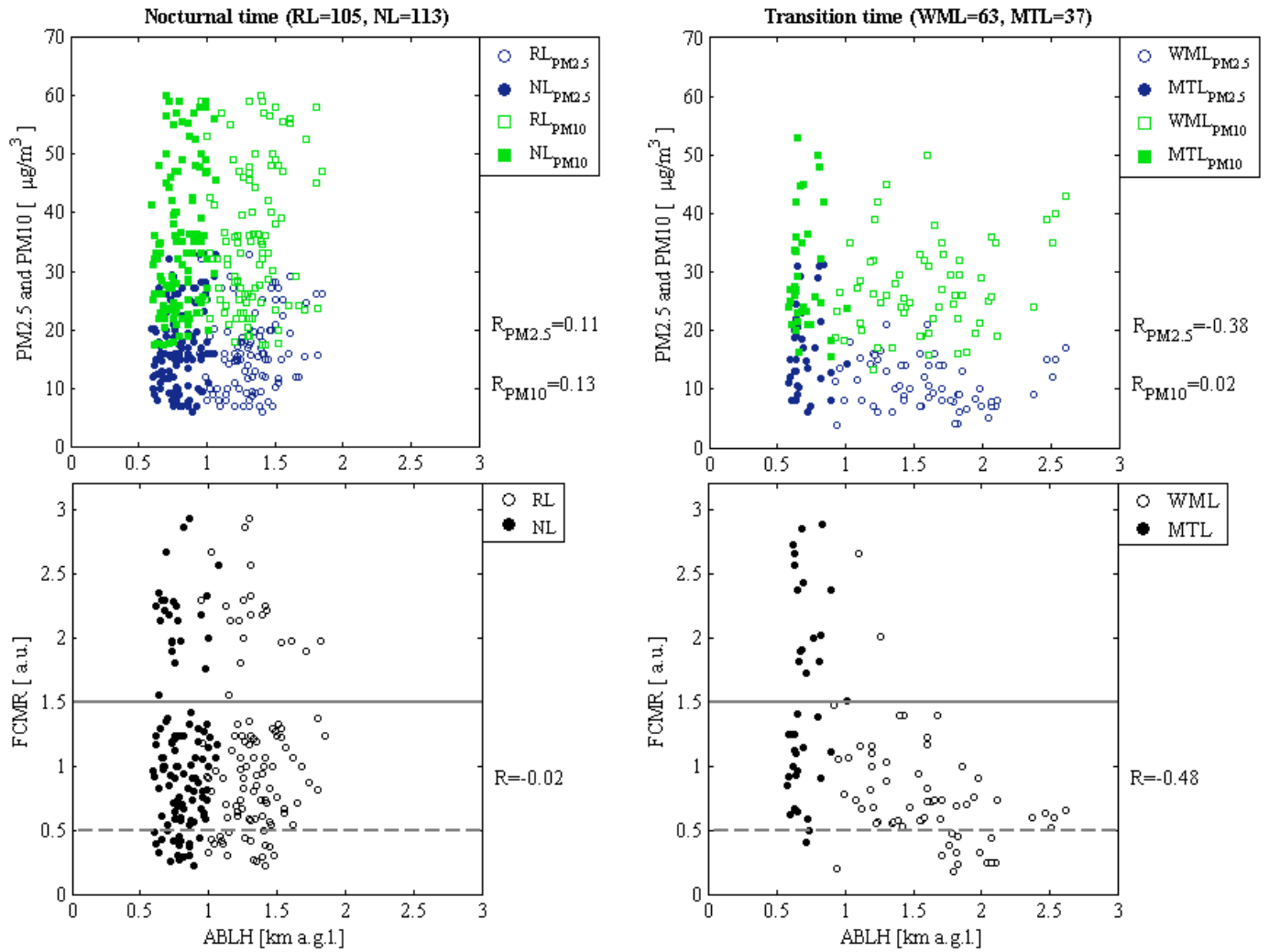
Figure 6. Hourly averages of surface fine to coarse mass ratio (FCMR), and particulate matter ( PM_{2.5} and PM_{10} ) measured at the WIOS site in Warsaw-Ursynow versus atmospheric boundary layer height (ABLH) derived from PollyXT lidar at the EARLINET/ACTRIS site of RS-Lab in Warsaw for period of July-September of 2013, 2015, 2016. Thresholds of FCMR are marked as horizontal lines.
