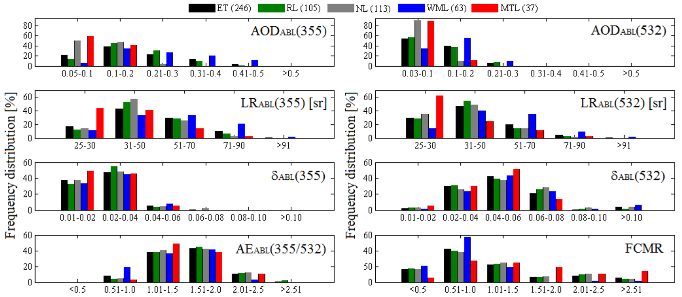
5 Figure 2. Frequency distribution of aerosol optical depth (AOD), lidar ratio (LR), linear particle depolarization ratio ( \delta ) and Ångström exponent ( \text{\AA E} ) at 355 and 532 nm derived within atmospheric boundary layer at the EARLINET/ACTRIS lidar site in Warsaw for period of July-September 2013, 2015, 2016. Corresponding fine to coarse mass ratio (FCMR) derived from measurements of surface particulate matter with an aerodynamic diameter below 10 \mu\text{m} ( \text{PM}_{10} ) and below 2.5 \mu\text{m} ( \text{PM}_{2.5} ) at the WIOS site in Warsaw-Ursynow. The period of measurement is divided to the entire time (ET; 24 h), the nocturnal time (NT; 22:00-2:00 UTC, including the residual 10 boundary layer RL and the nocturnal boundary layer NL), and the transition time (TT; after sunrise at 03:00-8:00 for the morning transition layer MTL and before sunset at 16:00-20:00 UTC for the well-mixed boundary layer WML).
