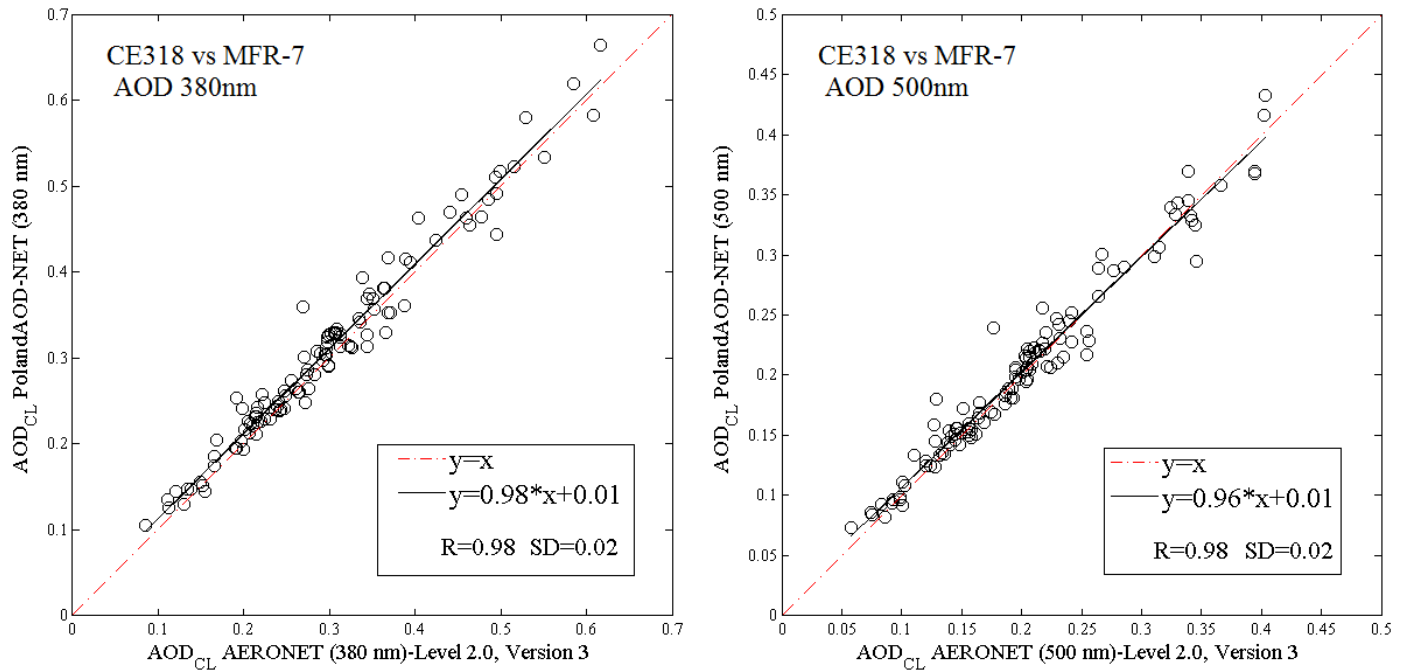
Figure 3. Intercomparison of hourly averaged clear-sky daytime aerosol optical depth measured within the atmospheric column ( AOD_{CL} ) with CE318 at the AERONET site in Warsaw (Version 3 Level 2.0 data) and the MFR-7 shadowband radiometer at the PolandAOD-NET site in Warsaw (Level 1.5 data). Note a high agreement obtained for both wavelengths for a month (July 2018) of collocated measurements (instruments in a distance of 3 m at the same altitude) at the RS-Lab in Warsaw. The AOD_{CL} at 415 nm from MFR-7 was scaled to 380 nm using Ångström law.
