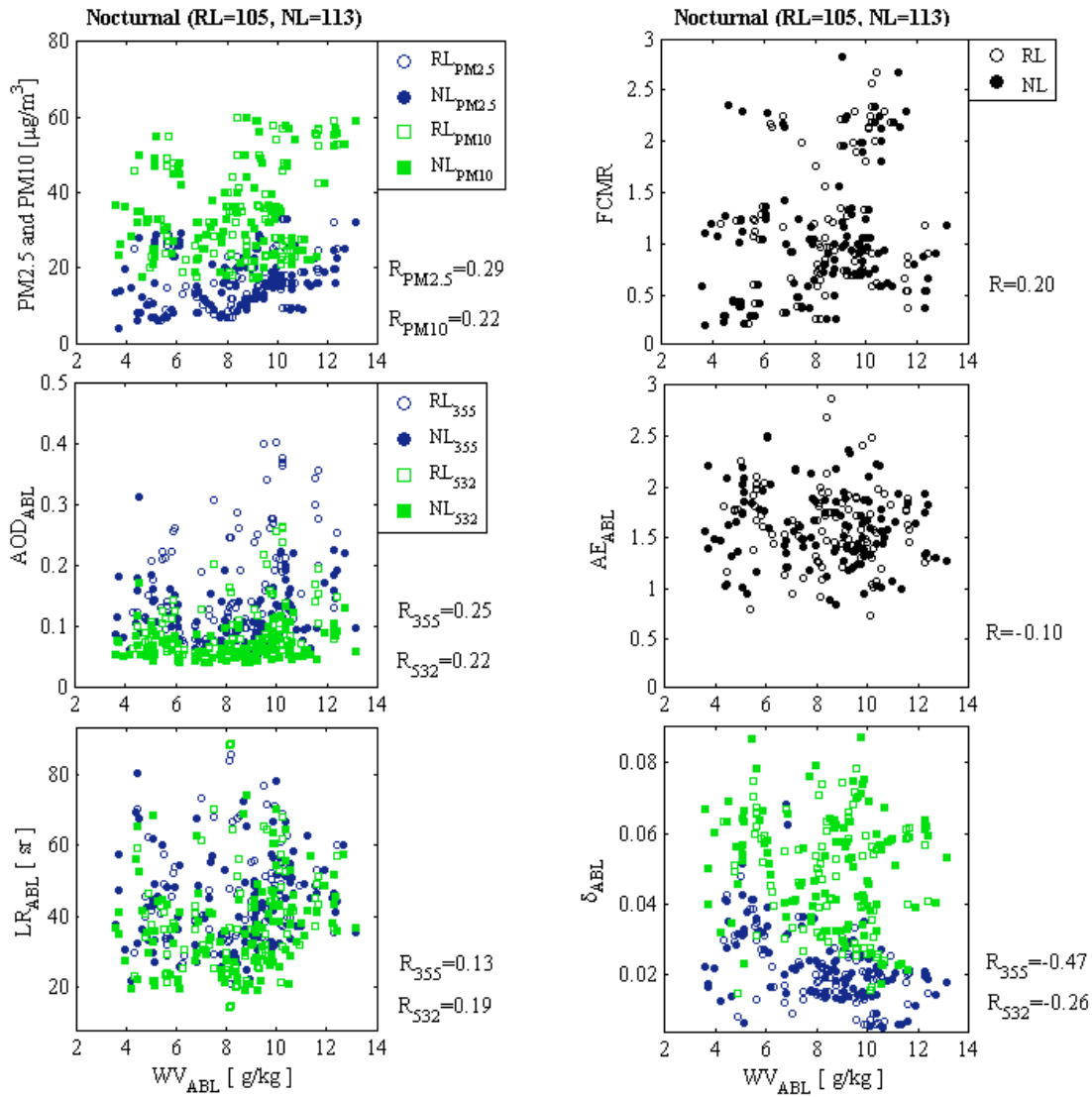
Figure 10. Nighttime hourly averaged water vapour mixing ratio (WV) versus aerosol optical depth (AOD), lidar ratio (LR), Ångström exponent (ÅE) and linear particle depolarization ratio ( \delta ), all derived within atmospheric boundary layer from PollyXT lidar at the EARLINET/ACTRIS site of RS-Lab in Warsaw, and versus fine to coarse mass ratio (FCMR) and surface particulate matter PM 2.5 and PM 10 measured at the WIOS site in Warsaw-Ursynow, during period of July-September of 2013, 2015, 2016. Note that lidar-derived WV is available only at nighttime.
