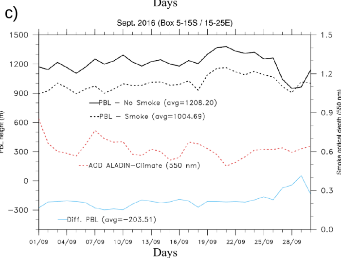
Figure 15. Daily-mean Surface Temperature, Sensible Heat Fluxes and PBL height obtained from the CTL (black lines) and SMK (dashed black) ALADIN-Climote simulations for september 2016. The AOD (red dashed lines) and the difference between the two simulations (CTL and SMK) for each variables are also reported (blue lines).
