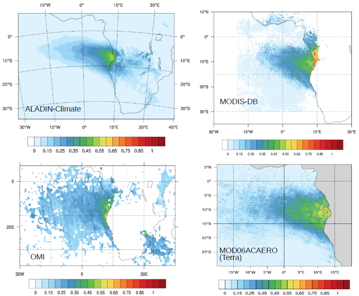
1530 Figure 6 Total monthly-averaged ACAOD (at 550 nm) for September 2016 simulated by the 1535 ALADIN-Climate (10:30 and 13:30 UTC outputs only are used) model and derived from MODIS (Deep-Blue and Meyer retrievals) and OMI instruments.
