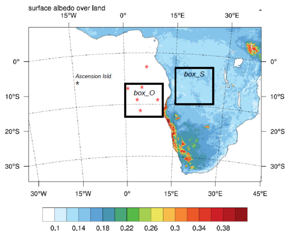
Figure 1. Domain defined for the ALADIN-Climate model simulations (here, the surface albedo is represented). The two different boxes (box_O and box_S) and the Ascension Island are indicated. Red stars represent the localisation of different profiles studied in the Part 4.2.3.2.
