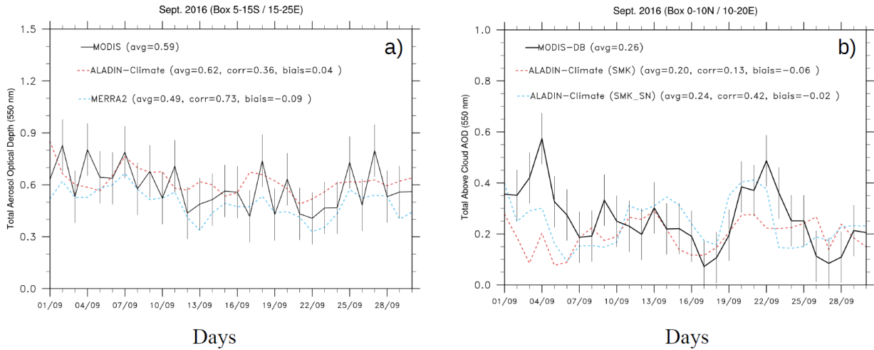
Figure 4. Total daily-mean AOD (at 550 nm) averaged over the box_S (5-15S / 15-25E) from the 1495 ALADIN-Climate model (10:30 and 13:30 UTC outputs are used), MERRA2 and derived from MODIS-Aqua DT data (left). Daily-mean ACAOD (at 550 nm) estimated from the MODIS-DB satellite and two different configurations of the ALADIN-Climate model (SMK and SMK_SN) averaged over the box_O (0-10N / 10-20E) (right). Uncertainties related to DT AOD and DB ACAOD are also indicated.
