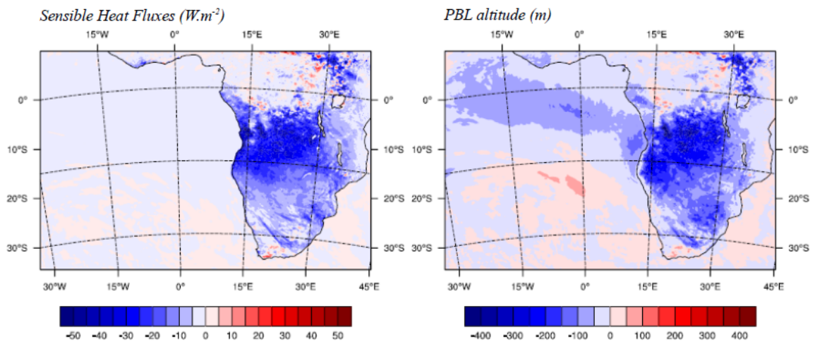
Figure 14. Differences between the CTL and SMK ALADIN-Climate runs in the monthly-mean (September 2016) SW surface radiations (top left), 2 meter continental temperature (top right), sensible heat fluxes (bottom left) and PBL height (bottom right).
