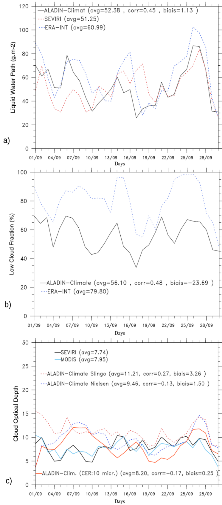
Figure 2. Daily-mean Sc properties (LWP, LCF and COD) simulated by ALADIN-Climate and from ERA-INT and SEVERI data. Values have been averaged over the box_O.
