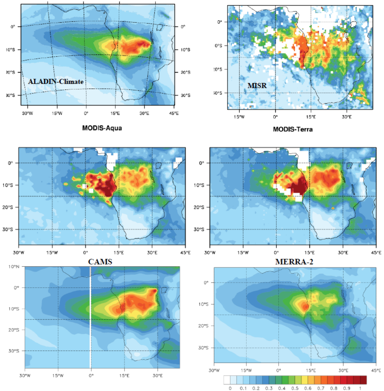
Figure 3. Total monthly-averaged Total AOD (at 550 nm) for september 2016 simulated by 1485 ALADIN-Climate (all times used), CAMS, MERRA2 and derived from the MODIS Terra, Aqua (combined DB/DT products) and MISR sensors.
