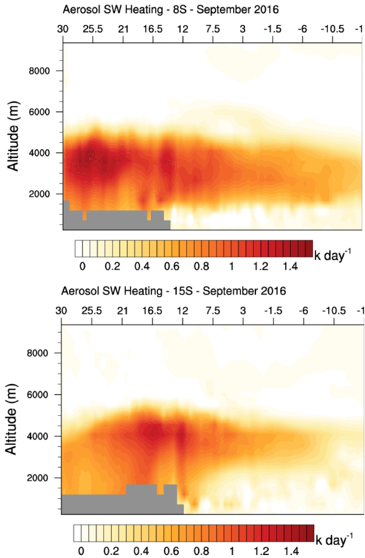
1645 Figure 10. Monthly-mean (September 2016) aerosol SW heating rate vertical profiles simulated by the ALADIN-Climate model for two transects at latitudes of 8 (top) and 15°S (bottom). Longitudes are between 30°E to 11.5°W.
