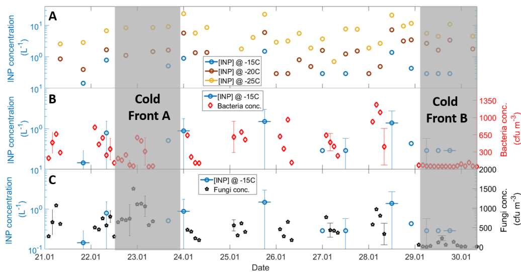
Fig. 9. A) Time series of the [INP] at -15 °C (blue), -20 °C (brown), and -25 °C (yellow), B) Time series of the [INP] at -15 °C (blue) together with bacteria concentration (red), and C) Time series of the [INP] at -15 °C (blue) together with fungal concentration (black). Each X-axis tick corresponds to 06:00 local time. The horizontal uncertainty bars indicate the time span the MOUDI-DFT measurements i.e., 6 h. Grey areas denote the periods affected by the entrance of a cold front (A and B).
