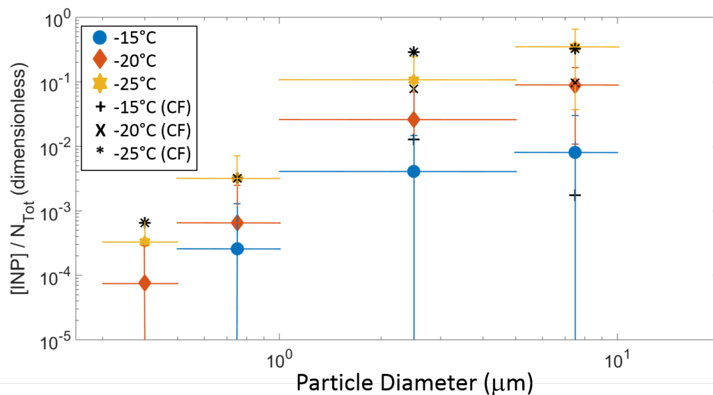
Fig. 7. Fraction of aerosol particles acting as an INP ( [INP] / N_{Tot} ) as a function of particle size at -15^{\circ}C , -20^{\circ}C , and -25^{\circ}C , respectively. N_{Tot} refers to the number of aerosol particles in a given size range measured by the LasAir. The solid colored symbols represent the entire campaign, while the black symbols represent the samples collected under the influence of the cold fronts (CF).
