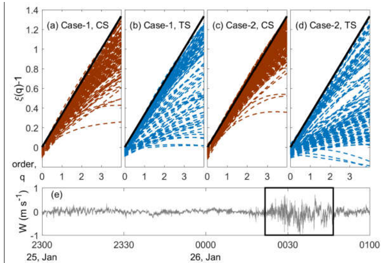
15 Figure 5. Hilbert-based scaling exponent function at 40 m during different stages for (a)–(b) Case-1 and (c)–(d) Case-2, where each dashed curve represents the result of 30-min vertical wind speed signal and the black solid line denotes the K41 result q/3 . (e) compares vertical wind fluctuation at 40 m between the CS (before 00:00 on 26 January 2017) and TS (after 00:00 on 26 January 2017). The latter shows apparent ‘bursts’ marked by the rectangular frame.
