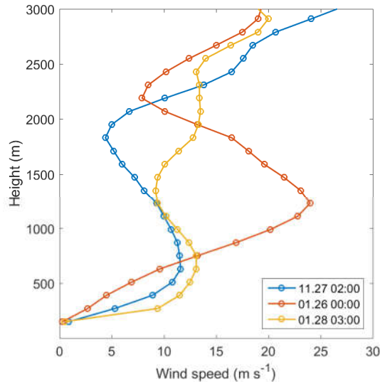
5 Figure 9. Sample LLJ profiles for three transitions between CSs and TSs.
