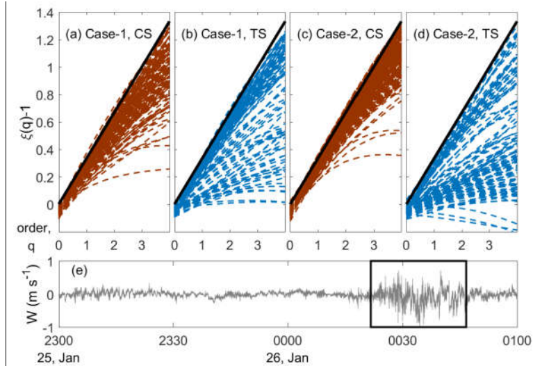
15 Figure 5. Hilbert-based scaling exponent function at 40 m during different stages for (a) – (b) Case-1 and (c) – (d) Case-2, where each dashed curve represents the result of 30-min vertical wind speed signal and the black solid line denotes the K41 result q/3 . (e) compares vertical wind fluctuation at 40 m between the CS (before 00:00 on 26 January 2017) and TS (after 00:00 on 26 January 2017). The latter shows apparent ‘bursts’ marked by the rectangular frame.
