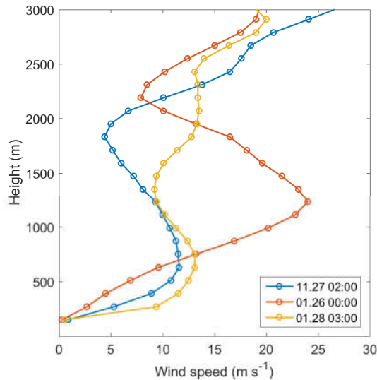
10 Figure 9. Sample LLJ profiles for three transitions between CSs and TSs.
