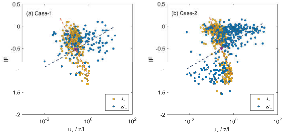
10 Figure 7. Scatter plot of IF vs. u_* and z/L (night time) for (a) Case-1 and (b) Case-2 at 40 m. The dashed lines are the fittings from least-squares regression and the triangle marks the cross point.
