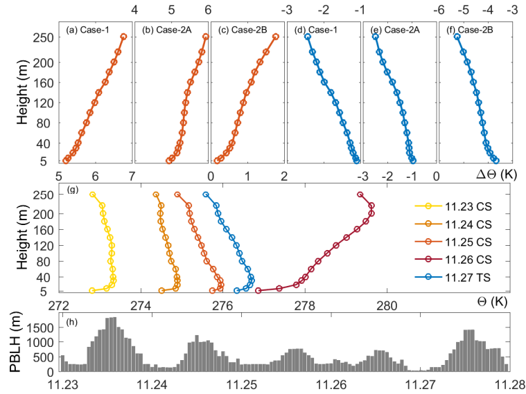
Figure 3. Vertical distribution of daily mean potential temperature. The change of daily mean potential temperature of CSs is showed in (a)–(c) and (d)–(f) are for TSs. (g) illustrates the evolution of inversion layer of Case-1. (h) is the PBLH simulated with WRF Model.
