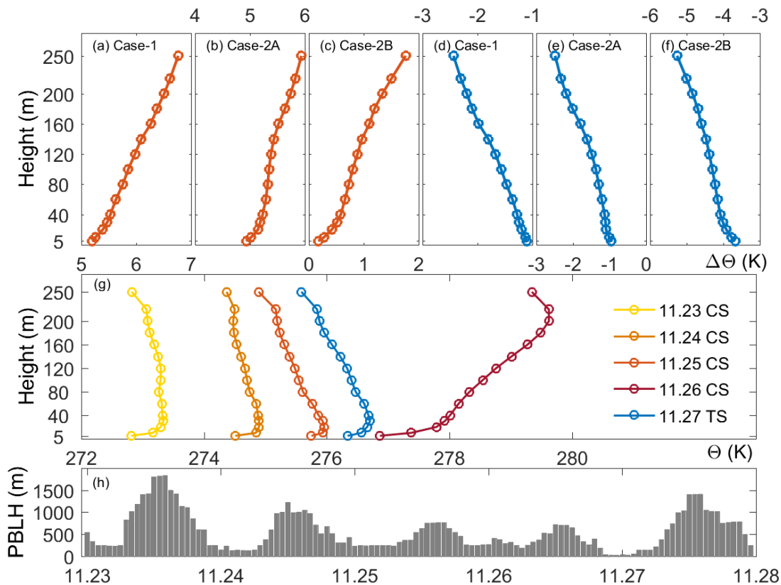
Fig. 4. Vertical distribution of daily mean potential temperature. The change of daily mean potential temperature of CSs is shown in (a)–(c) and (d)–(f) are for TSs. (g) illustrates the evolution of inversion
