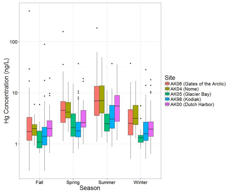
690 Figure 2. Summary boxplot of Hg concentrations separated by monitoring station and collection season. Similar seasonal trends are observed at each site with the highest concentrations occurring in summer and lowest concentrations in fall. Spring (March, April, May), Summer (June, July, August), Fall (September, October, November), Winter (December, January, February).
