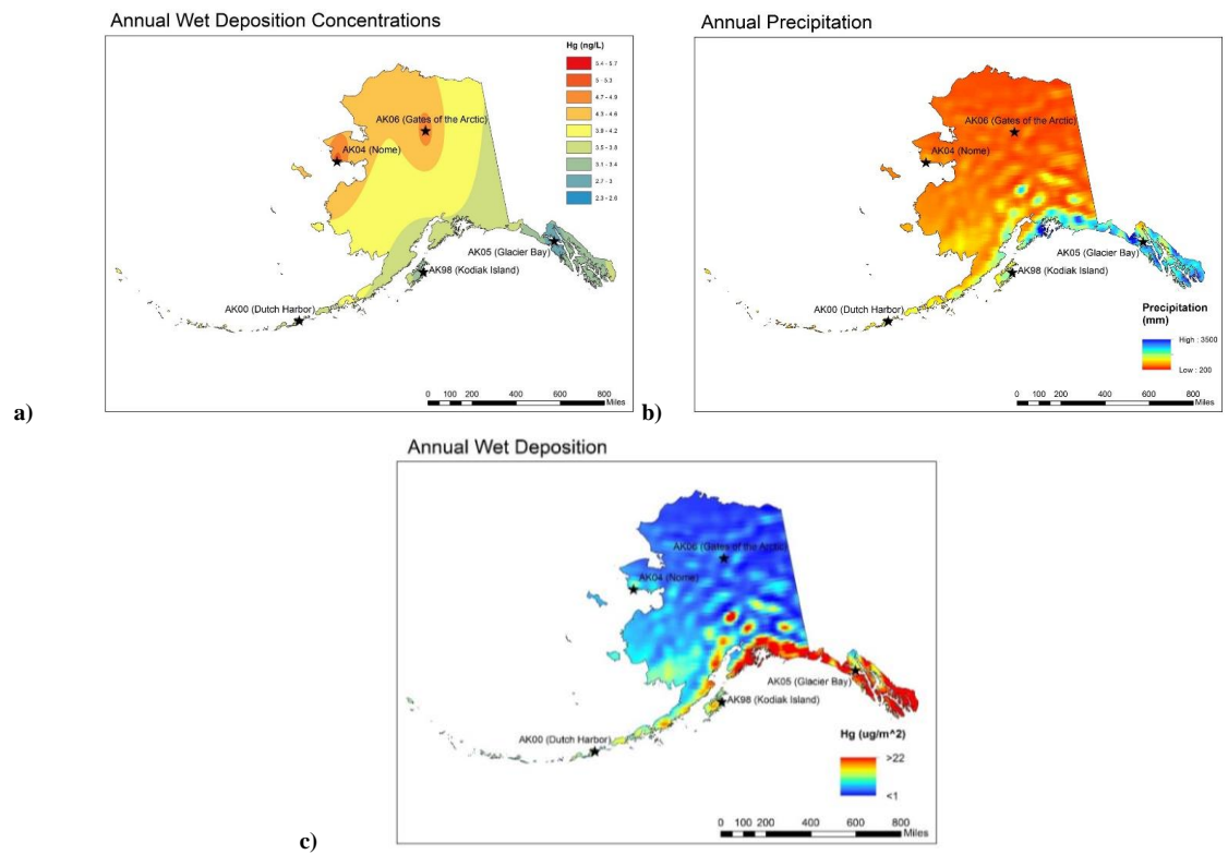
700 Figure 4. Average Annual Hg deposition maps for the state of Alaska: a) Inverse distance weighted concentration layer; b) NCEP Climate Forecast System Precipitation 2007-2015 annual average; c) Hg deposition estimates. Maps show large-scale concentration gradients (north/south) largely due to precipitation differences with total loading being highly dependent on precipitation.
