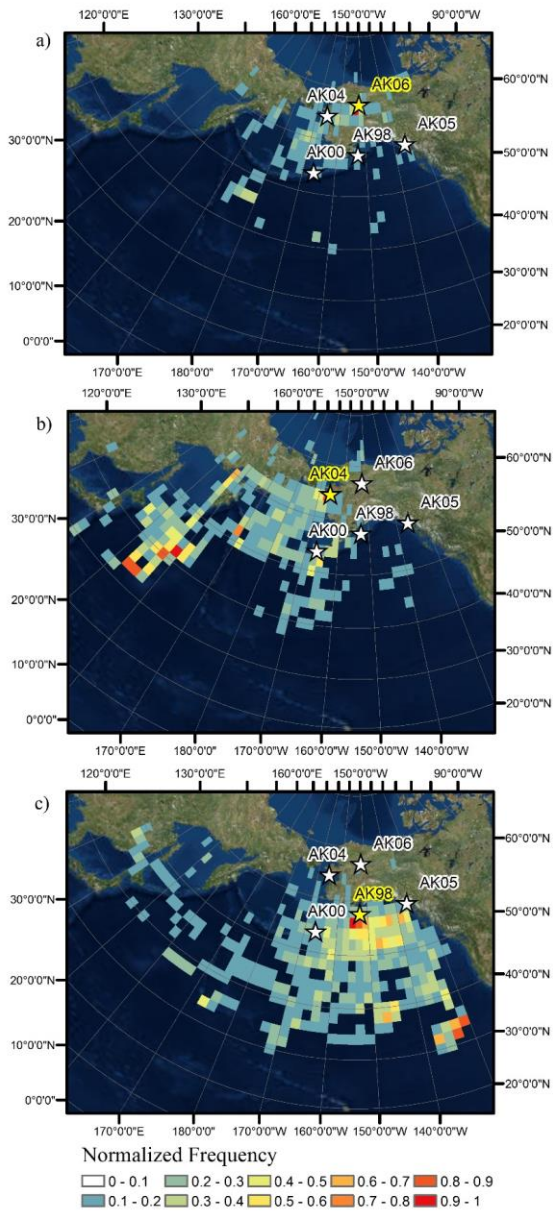
705 Figure 5. Normalized-frequency maps weighted by Hg deposition for top) Gates of the Arctic (AK06), middle) Nome (AK04), and bottom) Kodiak Island (AK98).
