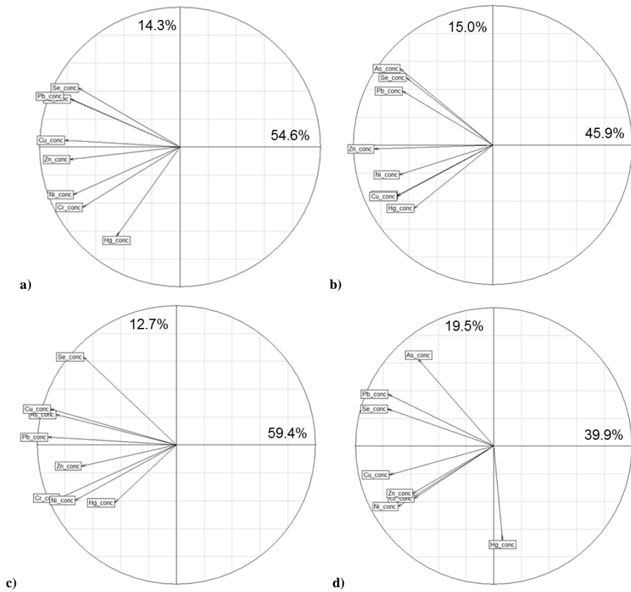
Figure 6. Trace metal rank-based principal component analysis bipoles of component 1 (x-axis) versus component 2 (y-axis) for a) All Sites, b) Dutch Harbor, c) Nome, and d) Kodiak Island. Values represent the % variance explained by each relative component.
