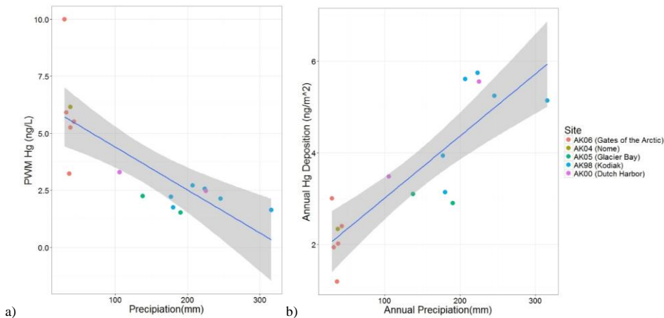
695 Figure 3. a) Plot of annual precipitation-weighted mean (PWM) Hg concentration versus annual precipitation (mm). Linear regression analysis shows a significant relationship with a correlation coefficient R^2=0.557 , p\text{-value} < 0.001 . b) Plot of annual Hg deposition versus annual precipitation (mm). Linear regression analysis shows a significant relationship with a correlation coefficient of R^2=0.7141 , p\text{-value} < 0.001 .
