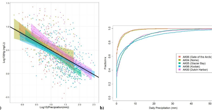
685 Figure 1. a) Scatterplots of observed Hg concentrations and precipitation amounts, separated by station. The black line shows the overall regression using all sites/all data. A clear dilution effect is observed at all sites. b) Empirical cumulative distribution plot of daily precipitation at five monitoring stations in Alaska (plot has been cropped at 50 mm). Distinct differences in storm size are observed between the northern (red and gold lines) and southern stations (green, blue, and purple lines).
