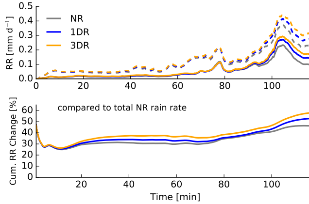
Figure 14. Vertically-integrated Total rain rate calculated from the trajectory ensemble simulation from recirculating parcels with a threshold of 0.01 \text{ gkg}^{-1} . The dashed lines show the total rain rate, the solid line the rain rate from recirculating parcels as well as the relative difference between the cumulated sum rain rates from recirculating parcels compared to the cumulated sum total NR rain rate.
