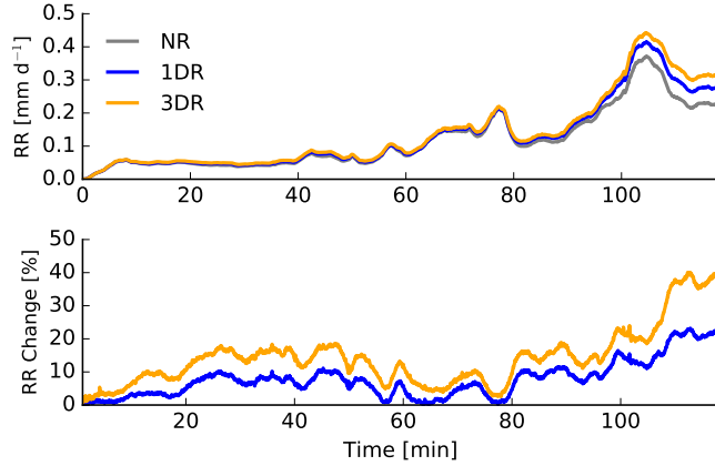
Figure 12. Vertically-integrated Total parcel rain rate calculated from the trajectory ensemble parcel-simulation (by integrating the size bins from 20 accounting for drop radii > 20 \mu\text{m} on). The top panel shows the absolute rain rate for the NR, the 1DR and the 3DR cases. The bottom panel shows the relative differences of 1DR simulation and the NR case, and 3DR simulation and the NR cases.
