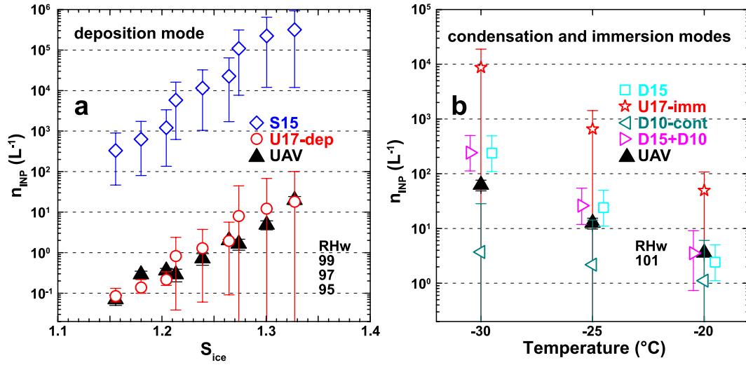
Figure 9. INP concentrations ( n_{\text{INP}} ) estimated from the CALIPSO lidar measurements on 21 April 2016 presented in Figure 7-6 (coloured symbols) and the UAV-FRIDGE measurements (black triangles) for (a) deposition freezing (as a function of saturation over ice) and (b) condensation and immersion freezing (as a function of temperature). Data in (a) are obtained for values of relative humidity over water of 95%, 97%, and 99%, leading to three values of S_{\text{ice}} for each analysed temperature. A relative humidity over water of 101% is used to obtain the values presented in (b).
