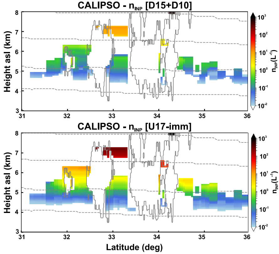
Figure 13. Spatial distribution of the INP concentrations during the event of 21 April 2016 at 11:01 UTC, as derived with the D15+D10 (top) and U17-imm (bottom) parameterisations. The location of the clouds observed are depicted with gray contours. The dotted lines correspond to T = 0, -10, -20 and -30 °C, based on the MERRA-2 model.
