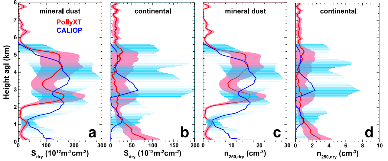
Figure 6. Profiles of the surface (a, b) and number concentrations (c, d) of mineral dust (a, c) and continental particles (b, d) with a dry radius larger than 250 nm derived from measurements with PollyXT between 1 and 2 UTC on 21 April 2016 (red) and retrieved from averaging 160 km of CALIOP measurements centred around an overpass at a distance of 5 km from Nicosia at 11:01 UTC on 21 April 2016 (blue).
