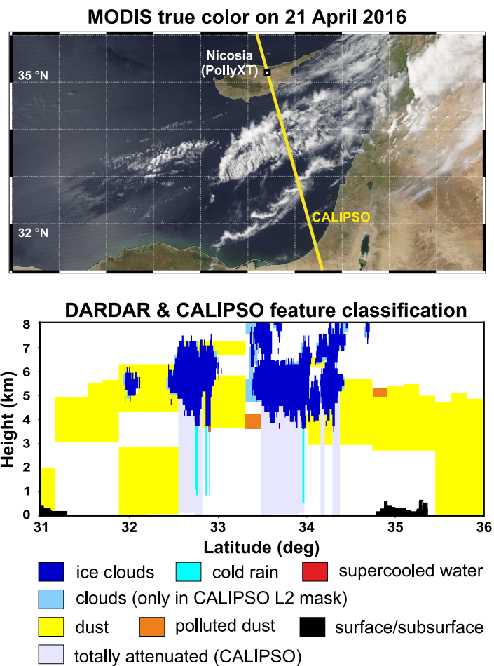
Figure 5. A-Train observations on 21 April 2016 at 11 UTC of MODIS-Aqua true color (up) and DARDAR & CALIPSO feature classification (bottom).
