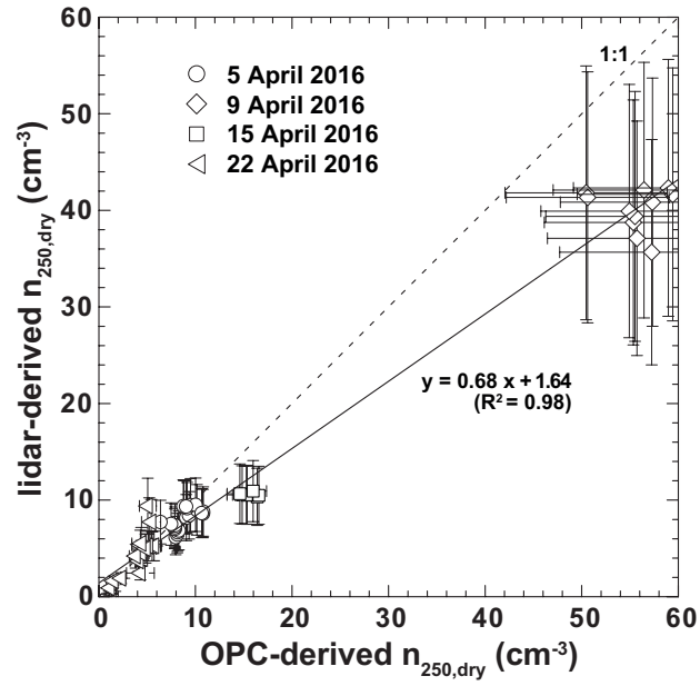
Figure 8. Correlation plot of n_{250,dry} obtained from drone-based OPC measurements and inferred from lidar observations (values for a mixture of mineral dust and continental pollution, black in in Figure 7) during coordinated activities on 5, 9, 15 and 22 April 2016. The solid line marks the linear regression with the corresponding function and squared correlation coefficient given in the plot. The 1:1 line is given as dashed line.
