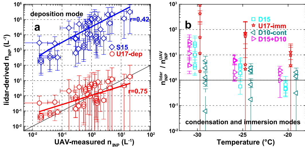
Figure 10. Comparison of INP concentrations derived from the CALIPSO and PollyXT lidar observations and UAV-FRIDGE measurements for (a) deposition freezing and (b) condensation and immersion freezing for cases with dust and continental presence. Colours and symbols refer to the used parameterization. Lines in (a) and (b) mark the 1:1 line. Numbers in (a) give Pearson's r of the linear fits.
