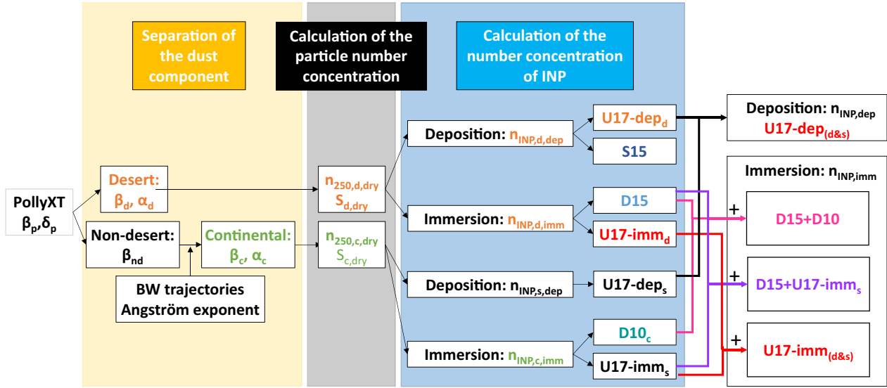
Figure A1. Overview of the data analysis scheme followed for the PollyXT measurements in this work. In the first step, we separate desert and non-desert backscatter coefficients ( \beta_d and \beta_{nd} ) by means of the particle linear depolarization ratio ( \delta_p ). The backscatter coefficients for the non-desert aerosol is estimated to be continental aerosol mixtures \beta_c by means of, e.g., backward (BW) trajectory analysis and Ångström exponent information. The two backscatter coefficients are then converted to aerosol-type-dependent particle extinction coefficients ( \alpha_i ). In the next step, the extinction coefficients are converted to aerosol-type-dependent profiles of particle number concentrations ( n_{250,i,dry} ) and particle surface area concentration ( S_{i,dry} ). In the next step, ice-nucleating particle number concentrations ( n_{INP,i} ) are estimated by applying INP parameterisations from the literature indicated by D10, D15, S15, U17 for DeMott et al. (2010), DeMott et al. (2015), Steinke et al. (2015) and Ullrich et al. (2017), respectively. Finally, the INP concentrations estimated for the different aerosol types are summed in order to estimate the total n_{INP} .
