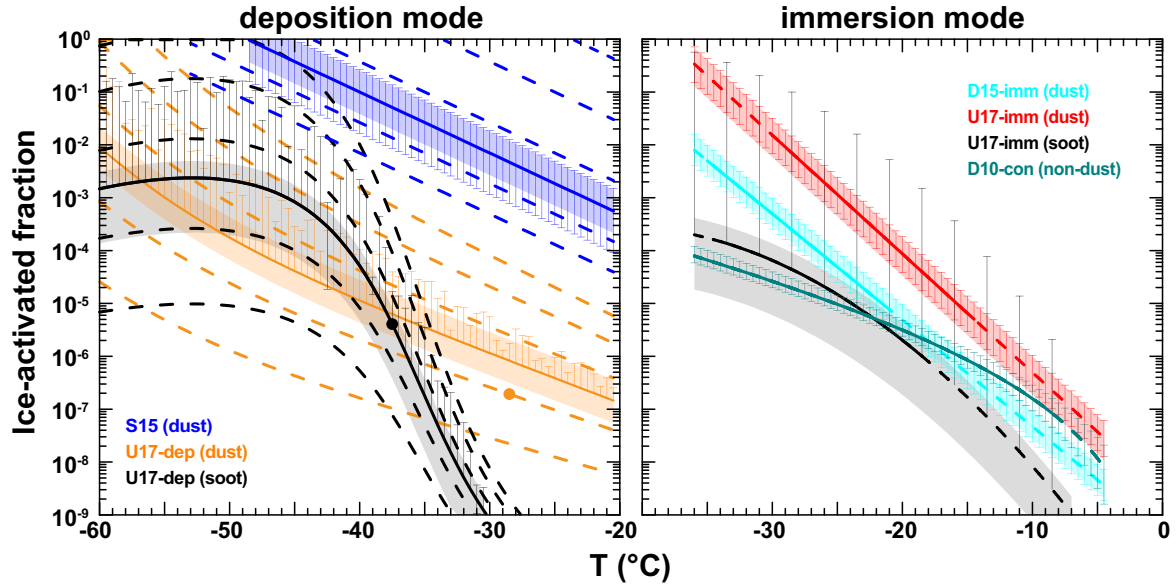
Figure 1. Fraction of ice activated particles for the deposition nucleation (left) and immersion freezing (right) parameterisations used in this study. The particle concentrations used are derived assuming an extinction coefficient of 50 \text{ Mm}^{-1} for each of the different aerosol types (dust, continental, soot). The shaded areas take into account a range of the extinction coefficient from 10 \text{ Mm}^{-1} (lower limit) to 200 \text{ Mm}^{-1} (upper limit). The error bars mark the error of the respective parameterisations from error propagation using the uncertainties provided in Table 2. Negative error bars that exceed the scale are not shown. In the deposition mode (left) panel, the bold lines correspond to ice supersaturation of 1.15 and the dashed lines to ice supersaturation of 1.05, 1.1, 1.2, 1.3 and 1.4. The black and orange dots indicate the maximum temperatures for which the parameterizations have been developed. In the immersion mode (right) panel, the parameterizations are extrapolated over the immersion-freezing temperature range (dashed lines).
