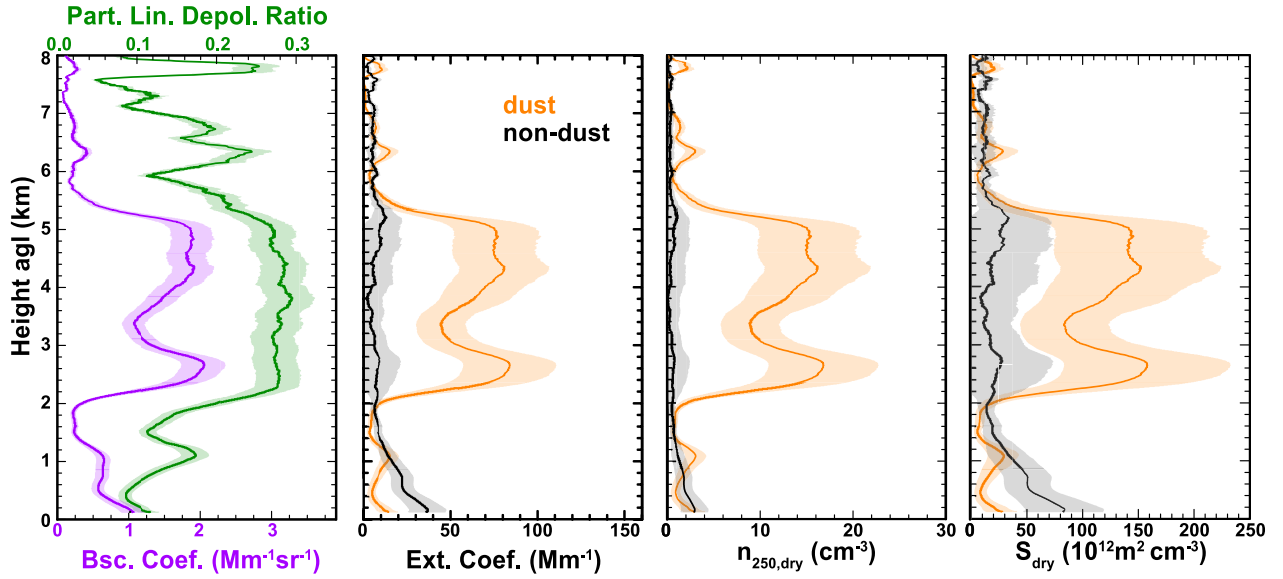
Figure 2. PollyXT profiles of the total particle backscatter coefficient (purple) and particle linear depolarisation ratio (green) measured between 1 and 2 UTC on 21 April 2016. The extinction coefficient as well as the number and surface concentration of particles with a dry radius larger than 250 nm related to mineral dust (orange) and non-dust aerosol (black) was obtained following the methodology described in Section 3.2.
