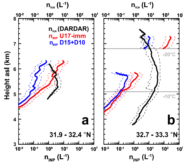
Figure 14. Concentration profiles of n_{\text{INP}} and n_{\text{ice}} from the A-Train measurements presented in Figure 12 and Figure 13 for the areas of (a) 31.9 to 32.4 °N (left) and (b) 32.7 to 33.3 °N (right). The n_{\text{INP}} dotted lines denote the uncertainties of the estimations. The n_{\text{ice}} dotted lines correspond to the 25 and 75% percentiles of the concentrations retrieved in the cloud. The overall uncertainty of the retrievals is discussed in the manuscript. The indicative temperature lines are from the MERRA-2 model.
