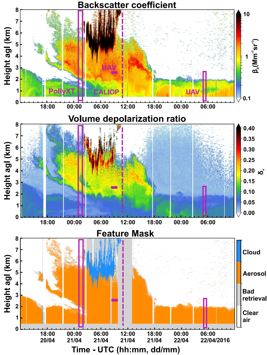
Figure 4. Time-height PollyXT observations between 12 UTC on 20 April 2016 and 12 UTC on 22 April 2016 of the backscatter coefficient at 1064-nm (up), the volume linear depolarization ratio at 532-nm (center) and the feature mask (bottom). The magenta markers refer to the analysed period of PollyXT (left box: 1 - 2 UTC on 21 April 2016), CALIOP (dashed line: 11:01 UTC on 21 April 2016) and UAV (horizontal bar: INP sampling between 8:30 and 9:40 UTC on 21 April 2016, right box: OPC measurements between 5:00 and 5:30 UTC on 22 April 2016) that are being referred to in this study. The bad retrievals in the feature mask refers to observations affected from (i) total attenuation due to clouds (ii) low signal-to-noise ratio and (iii) incomplete overlap.
