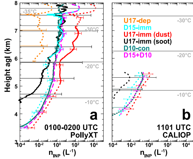
Figure 11. INP concentration profiles estimated from the measurements with (a) Polly-PollyXT between 0100-01:00 and 0200-02:00 UTC on 21 April 2016 and (b) CALIOP at 1101-11:01 UTC on 21 April 2016. Temperature levels have-been-extracted-are-derived from a-nearby the WRF profile-and MERRA-2 models. Colours refer to different INP parameterisations. Solid lines mark the temperature range for which the corresponding parameterisation has been developed. Dashed lines refer to the extrapolated temperature range (see Table 1).
