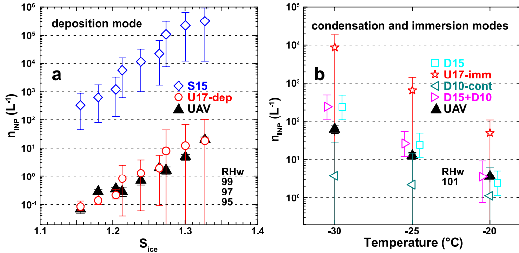
Figure 9. INP concentrations ( n_{\text{INP}} ) estimated from the lidar measurements on 21 April 2016 presented in Figure 7 (coloured symbols) and the UAV-FRIDGE measurements (black triangles) for (a) deposition freezing (as a function of saturation over ice) and (b) condensation and immersion freezing (as a function of temperature). Data in (a) are obtained for values of relative humidity over water of 95%, 97%, and 99%, leading to three values of S_{\text{ice}} for each analysed temperature. A relative humidity over water of 101% is used to obtain the values presented in (b).
