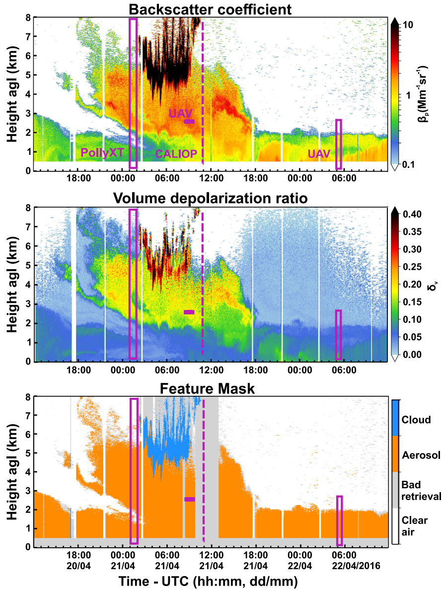
Figure 4. Time-height display of the 1064-nm range-corrected signal measured with PollyXT observations between 12 UTC on 20 April 2016 and 12 UTC on 22 April 2016 of the backscatter coefficient at 1064-nm (up), the volume linear depolarization ratio at 532-nm (center) and the feature mask (bottom). The magenta markers refer to the analysed period of PollyXT (left box; 1 - 2 UTC on 21 April 2016), CALIOP (dashed line; 11:01 UTC on 21 April 2016) and UAV (horizontal bar; INP sampling between 8:30 and 9:40 UTC on 21 April 2016 and right box; OPC measurements between 5:00 and 5:30 UTC on 22 April 2016) that are being referred to in this study. Vertical black lines - The bad retrievals in the lidar plot mark missing data. The feature mask refers to observations affected from (i) total attenuation due to clouds (ii) low signal-to-noise ratio and (iii) incomplete overlap.
