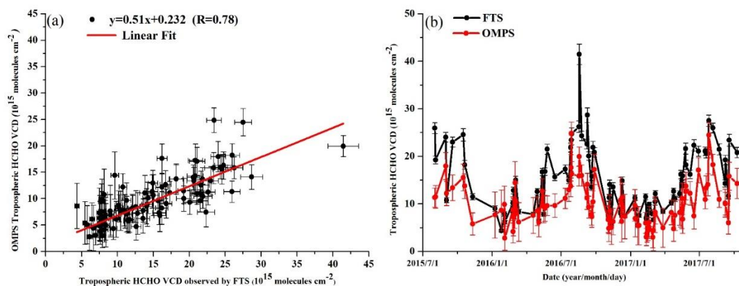
Figure 1. (a) Correlation analysis and (b) time series of tropospheric HCHO VCDs measured by OMPS and FTS from Jul.1 st , 2015 to Nov.20 th , 2017.
