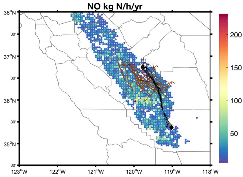
5 Figure 3 Soil NO emissions in kg N per hectare per year for the SJV with flight tracks (data from Almaraz et al. (2018)). Significant sources for soil NO show up in the middle SJV in Kings County.
