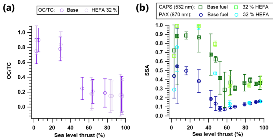
Figure 6. Thrust dependent (a) organic carbon to total carbon fraction (OC/TC), and (b) single scattering albedo (SSA) measured at 532 nm (green squares) and 870 nm (blue circles). Note: Dark colors represent measurements with base fuel (Jet A-1) and light colors represent measurements with the HEFA blend (32% vol.).
