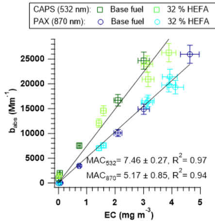
10 Figure 5. Scatter plot and linear regression lines between the absorption coefficient ( b_{abs} ) measured at 532 nm (green squares) and 870 nm (blue circles) and the elemental carbon (EC) mass concentration; Mass absorption cross section (MAC) values are retrieved from the slope of the linear fits. Note: Dark colors represent measurements with base fuel (Jet A-1) and light colors represent measurements with the HEFA blend (32% vol.).
