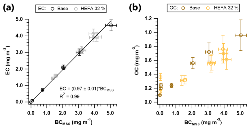
Figure 3. (a) Scatter plot and linear regression line of the mass concentrations of elemental carbon (EC) and black carbon measured with the micro soot sensor (BC MSS ); (b) Scatter plot of the mass concentrations of organic carbon (OC) and BC MSS . Note: Dark colors represent measurements with base fuel (Jet A-1) and light colors represent measurements with the HEFA blend (32% vol.).
