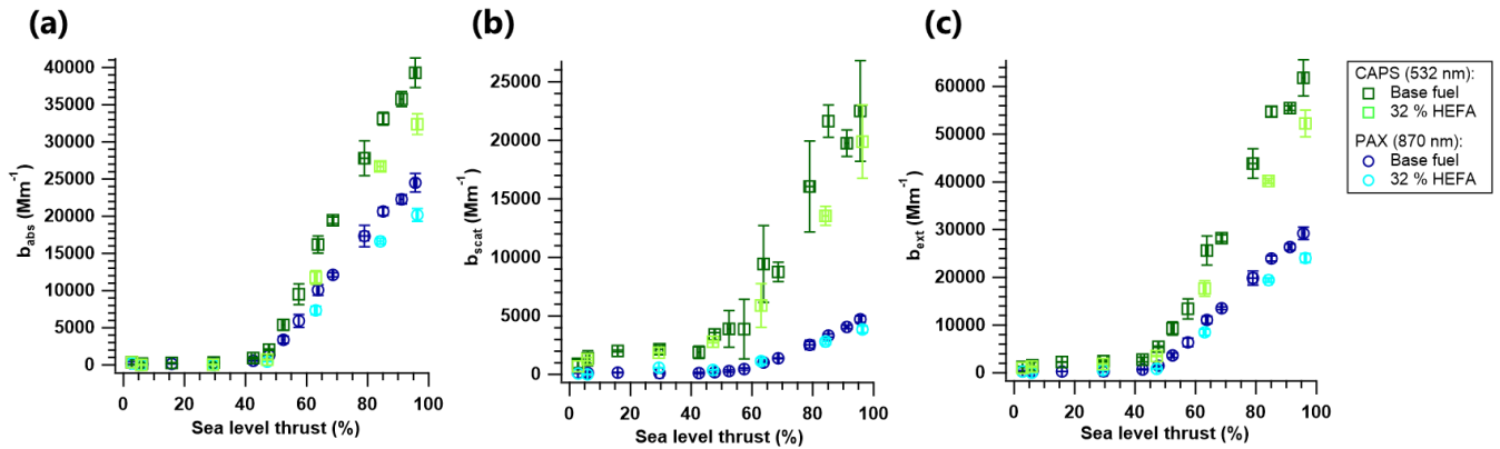
5 Figure 4. Thrust dependent (a) absorption coefficient ( b_{abs} ), (b) scattering coefficient ( b_{scat} ), and (c) extinction coefficient ( b_{ext} ) measured at 532 nm (green squares) and 870 nm (blue circles). Note: Dark colors represent measurements with base fuel (Jet A-1) and light colors represent measurements with the 32% vol. HEFA blend.
