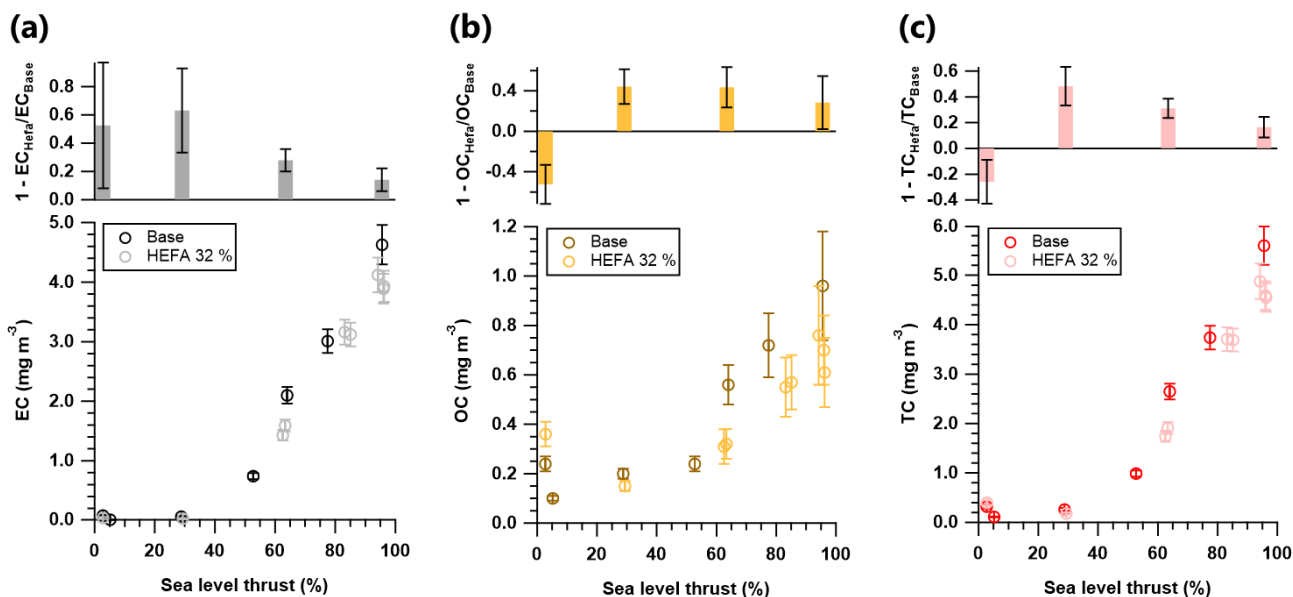
5 Figure 2. Thrust dependent mass concentration and decrease with the 32% HEFA blend compared to the base Jet A-1 fuel of (a) elemental carbon (EC), (b) organic carbon (OC), and (c) total carbon (TC). Note: Dark colors represent measurements with base fuel (Jet A-1) and light colors represent measurements with the HEFA blend (32% vol.).
