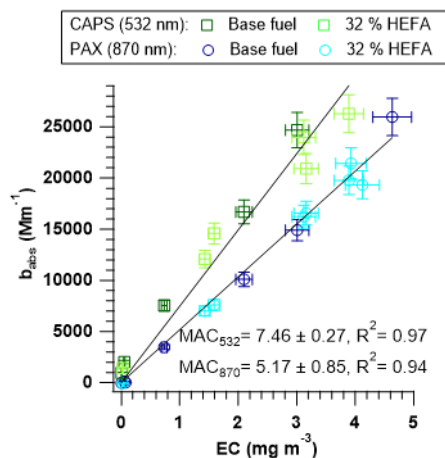
Figure 5. Scatter plot and linear regression lines Correlation between the absorption coefficients ( b_{abs} ) measured at 532 nm (green squares) and 870 nm (blue circles) and the elemental carbon (EC) mass concentration; Mass absorption cross section (MAC) values are retrieved from the slope of the linear fits. Note: Dark colors represent measurements with base fuel (Jet A-1) and light colors represent measurements with the HEFA blend (32% vol.).
