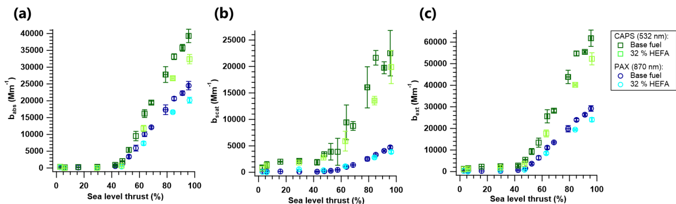
Figure 4. Thrust dependent (a) absorption coefficient ( b_{abs} ), (b) scattering coefficient ( b_{scat} ), and (c) extinction coefficient ( b_{ext} ) measured at 532 nm (green squares) and 870 nm (blue circles). Note: Dark colors represent measurements with base fuel (Jet A-1) and light colors represent measurements with the 32% vol. HEFA blend.
