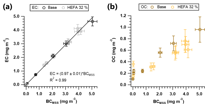
Figure 3. (a) Scatter plot and linear regression line of the mass concentrations of elemental carbon (EC) and black carbon measured with the micro soot sensor (BC MSS ) ; (b) Scatter plot of the mass concentrations of organic carbon (OC) and BC MSS . Correlation between the mass concentration of (a) EC, and (b) OC with BC MSS . Note: Dark colors represent measurements with base fuel (Jet A-1) and light colors represent measurements with the HEFA blend (32% vol.).
