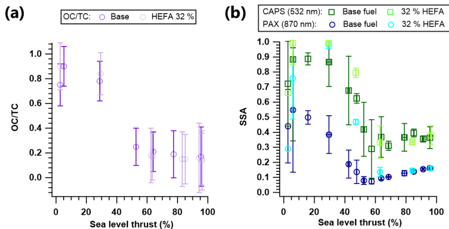
Figure 6. Thrust dependent (a) organic carbon to total carbon fraction (OC/TC) ratio , and (b) single scattering albedo (SSA) measured at 532 nm (green squares) and 870 nm (blue circles). Note: Dark colors represent measurements with base fuel (Jet A-1) and light colors represent measurements with the HEFA blend (32% vol.).
