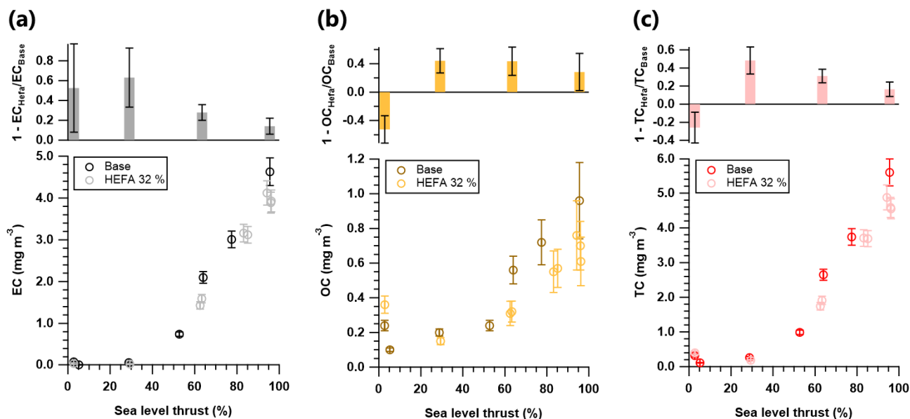
Figure 2. Thrust dependent mass concentration and decrease with the 32% HEFA blend compared to the base Jet A-1 fuel of (a) elemental carbon (EC) , (b) organic carbon (OC) , and (c) total carbon (TC) . Note: Dark colors represent measurements with base fuel (Jet A-1) and light colors represent measurements with the HEFA blend (32% vol.).
