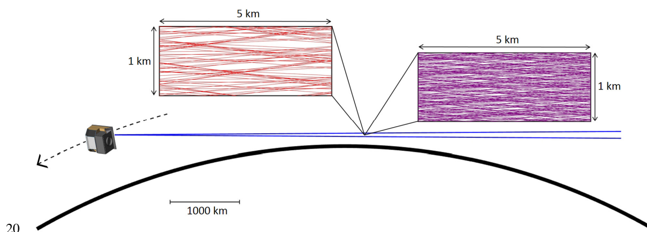
20 Figure 1. Illustration of the MATS limb observation geometry. From an orbit altitude of 585 km, the vertical field of view of the limb instrument covers nominal tangent altitudes from 75 to 110 km. The smaller inlays show examples of lines-of-sight filling a section of 5×1 km in the orbit plane. The density of the lines-of-sight is representative for the binned image pixels in an O 2 Atmospheric Band channel (left) and an NLC channel (right).
