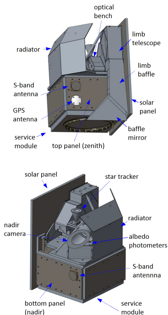
10 Figure 2. Layout of the MATS satellite.
