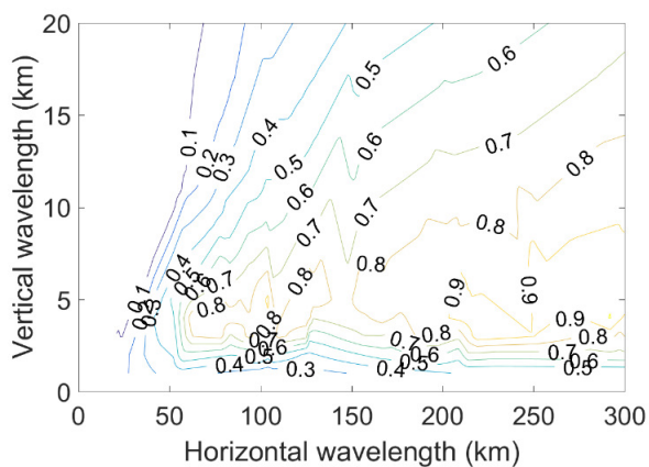
20 Figure 9. Simulated sensitivity of the MATS instrument to gravity waves of varying horizontal and vertical wavelengths. Results are shown for waves with wave fronts perpendicular to orbit plane. The sensitivity is defined as the ratio between the amplitude of the retrieved wave and the amplitude of the true wave field.
