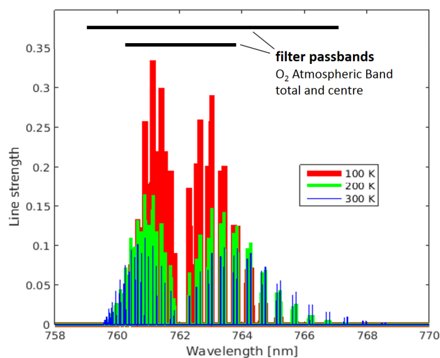
Figure 10. Spectral distribution of the O 2 Atmospheric Band rotational transitions in the 0-0 vibrational band as a function of temperature. The filter passbands of the limb instrument's Atmospheric Band channels cover the total band and its central part, respectively.
