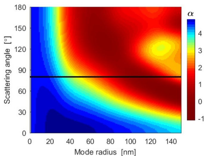
10 Figure 11. A lookup table for the NLC particle size analysis, generated from T-matrix simulations. Shown is the Ångström exponent as a function of mode radius and scattering angle. The black line indicates a typical scattering angle for MATS NLC observations.
