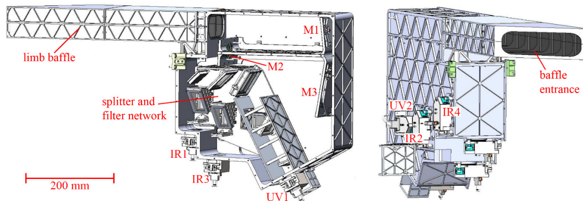
Figure 3. Overview of the MATS limb imager with one of the side covers removed (Hammer et al., 2018). Marked in the image are the telescope mirrors M1-M3, as well as the CCDs IR1-IR4 and UV1-UV2 for the six spectral channels.
