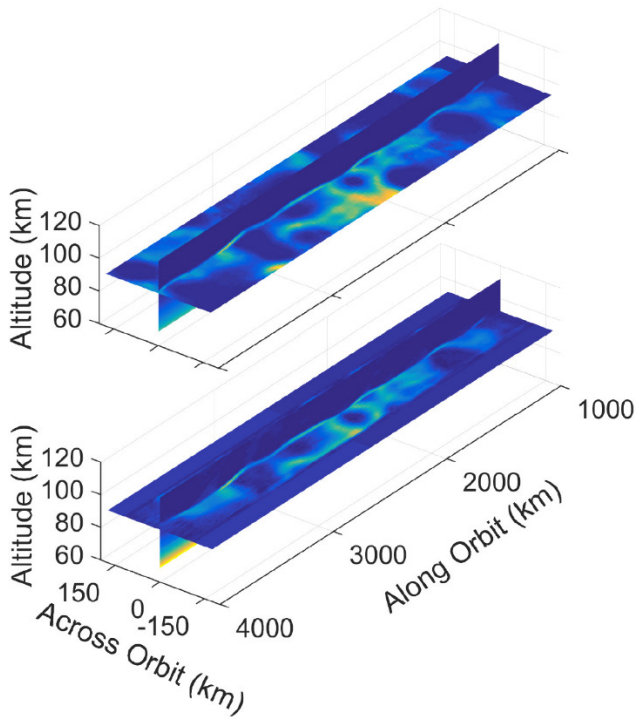
15 Figure 8. Example of tomographic retrieval simulations. The upper panel shows the simulated "true" NLC volume scattering coefficient. The lower panel shows the retrieved NLC. Based on the simulated lines of sight, full retrieval is available in an area 2000-3000 km along orbit and \pm 125 km across orbit.
