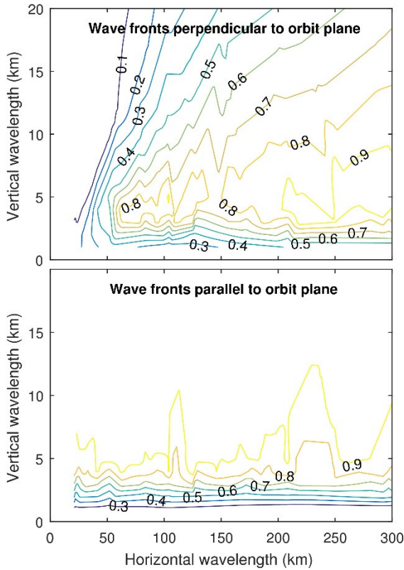
10 Figure 11. Simulated sensitivity of the MATS instrument to gravity waves of varying horizontal and vertical wavelengths. The sensitivity is defined as the ratio between the amplitude of the retrieved wave and the amplitude of the true wave field. Results are shown for waves with wave fronts perpendicular to the orbit plane (upper panel) and parallel to the orbit plane (lower panel).
