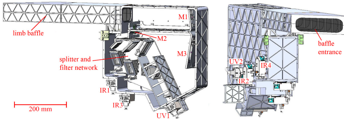
15 Figure 3. Overview of the MATS limb imager with one of the side covers removed (Hammar et al., 2018). Marked in the image are the telescope mirrors M1-M3, as well as the CCDs IR1-IR4 and UV1-UV2 for the six spectral channels.
