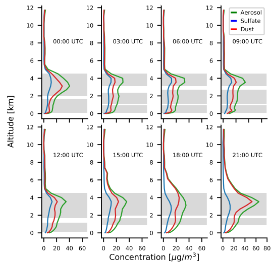
Fig. 2. CAMS total aerosol, sulfate and dust profiles for 04 April 2014, Pillersdorf. Grayed area represents the identified sulfate layers. Altitudes are given in km AGL. Local time is UTC+2
