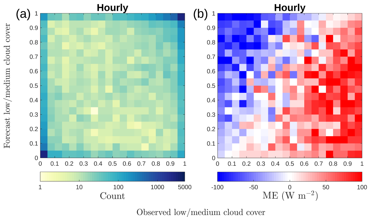
Figure 10. 2D-histogram of observed and forecast cloud cover (a), with colors representing counts on a logarithmic scale, and \text{MBE} - \text{ME} in solar radiation forecast (b) for each cloud cover pair in (a).
