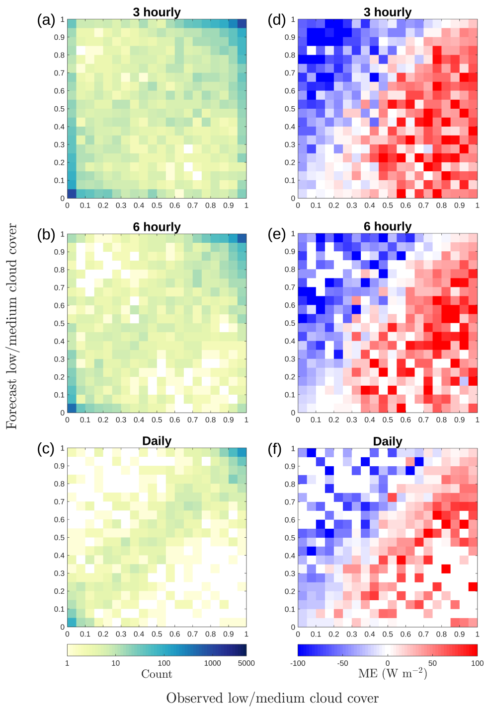
Figure 11. Same plots as Fig 10, except for different averaging time-windows.
