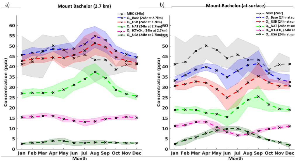
Fig. 1. Monthly 2004-2012 average 24-hour O 3 concentrations at Mount Bachelor Observatory. Observations (grey) are the same in both panels. Simulations from the GEOS-Chem model are sampled in the grid cell co
