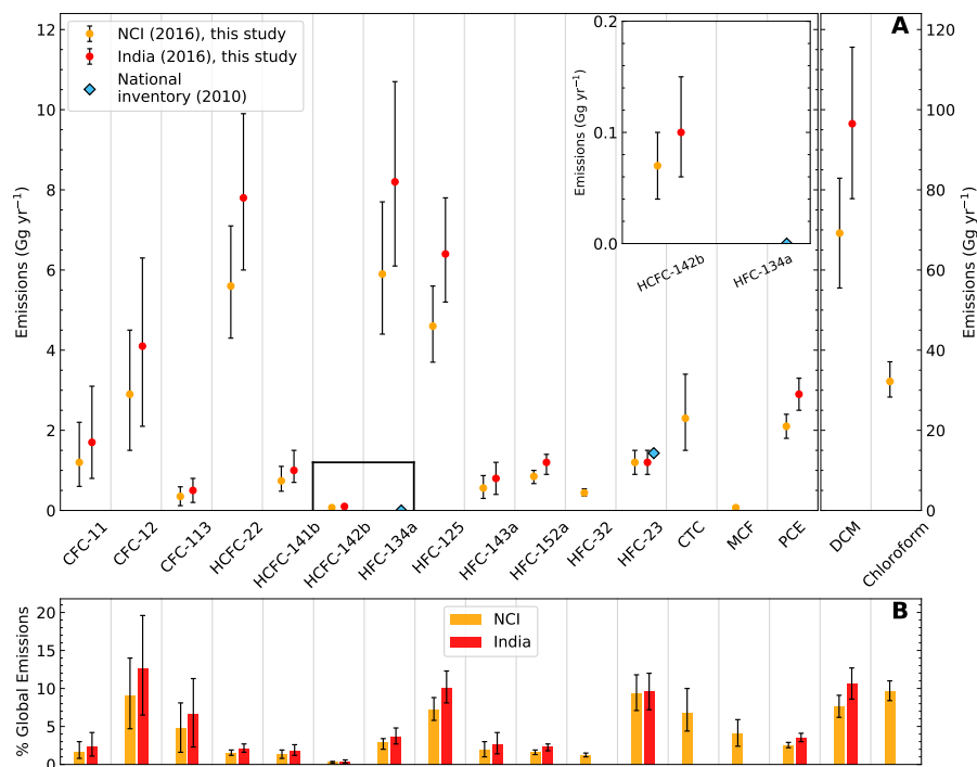
Figure 4. (A) NCI (orange) and India total (red) halocarbon emissions (Gg yr -1 ) derived in this study. India's most recent greenhouse gas inventory estimates (2010) are included where available. Note that emissions of DCM and chloroform are presented on a second y-axis for clarity. (B) The estimated contribution of the NCI and India to global halocarbon emissions (global estimates are an extension of the work by Rigby et al. (2014)). Error bars represent the 5 th -95 th percentiles of the posterior distribution.
