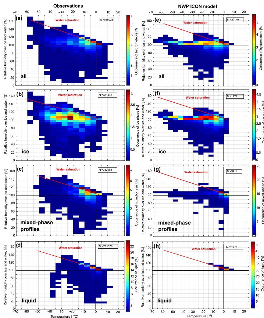
Figure 11. Two-dimensional histograms of in-cloud atmospheric temperature and relative humidity for all clouds (a,e), ice clouds (b,f), mixed-phase clouds (c,g). For a, c, e and g ice and/or liquid phases are present. For b and f only ice phase is present. Liquid phase of liquid-containing clouds is shown in d and h. Only cases of single-layer clouds are included and shown for observations (left) and for global NWP model ICON (right). Frequency of occurrence is normalized by the total number of bins of the correspondent single-layer clouds detected between the period of one hour before and after radiosonde launch.
