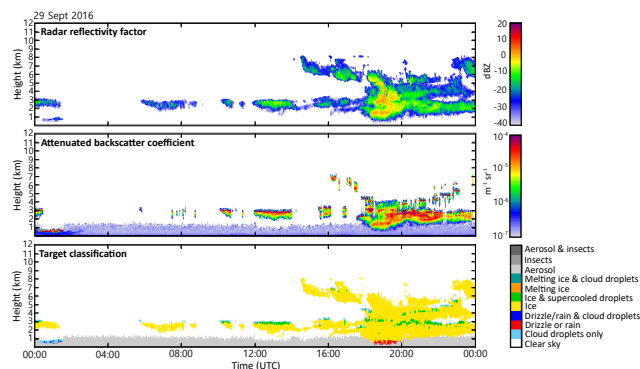
Figure 1. Radar reflectivity factor (top), lidar backscatter coefficient (middle) and Cloudnet target classification on 29 September 2016, AWIPEW observatory at Ny-Ålesund.
