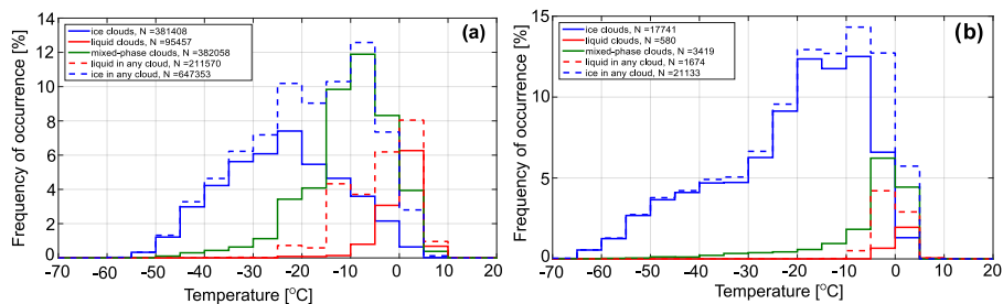
Figure 12. Distribution of in-cloud atmospheric temperature for different types of single-layer clouds, liquid and ice phase for observations (a) and global NWP ICON model (b).
