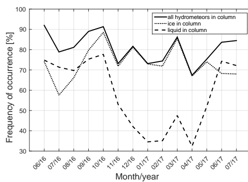
Figure 5. Frequency of occurrence of profiles with ice, liquid and any kind of hydrometeors. The frequency is given in % and normalized to the total number of Cloudnet profiles for each month.
