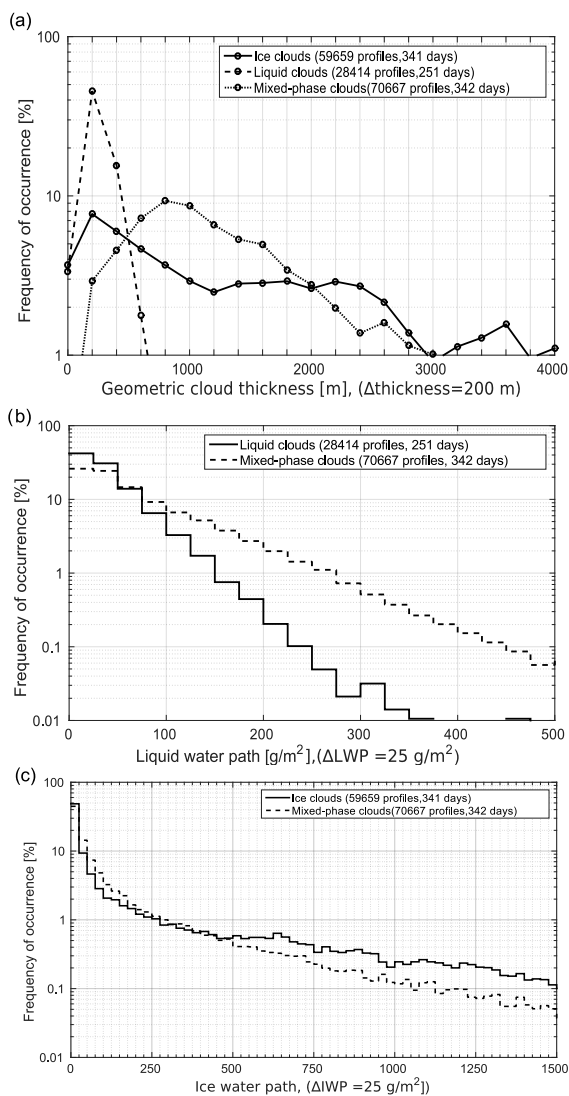
Figure 9. Frequency of occurrence of cloud thickness for single-layer clouds (a), of LWP for single-layer liquid and mixed-phase clouds (b) and of IWP for single-layer ice and mixed-phase clouds (c) for the period from June 2016 to August 2017. The y axis is shown in logarithmic scale. Frequency is normalized by the total number of corresponding cloud type.
