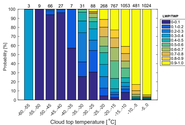
Figure 10. The relative probabilities of different ranges of the liquid fraction LWP/TWP given at various cloud top temperatures of single-layer mixed-phase clouds. The probability is normalized by the total number of profiles for each cloud top temperature range. Numbers at the top of plot show the number of cases included in the temperature range. The total number of all profiles is 3824.
