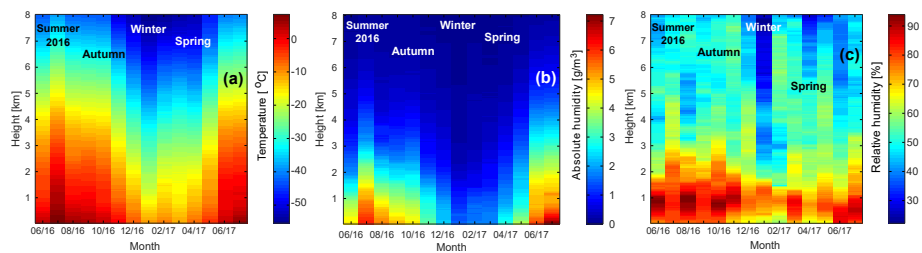
Figure 3. Vertical profiles of monthly mean atmospheric temperature (a), absolute (b) and relative humidity (c) from radiosonde observations at Ny-Ålesund from June 2016 to July 2017.
