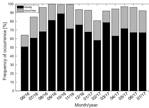
Figure 2. Cloudnet data availability for Ny-Ålesund for June 2016 to July 2017. Grey bars correspond to clear sky profiles, black bars to cloudy profiles.
