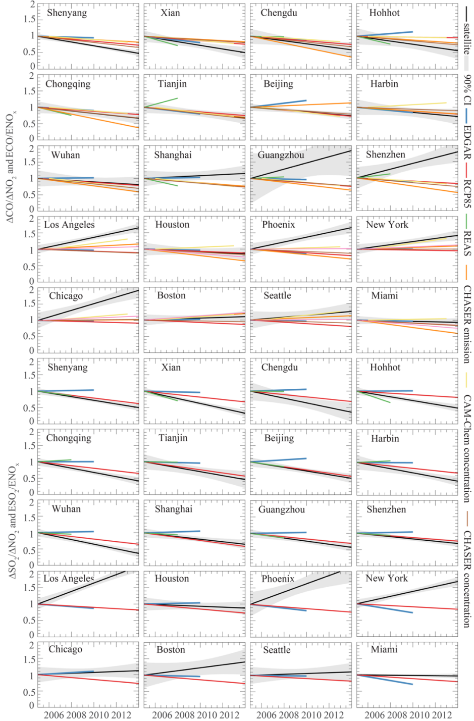
Fig. S1. Same as Figure 2 but for all the 12 Chinese cities and 8 U.S. cities.
