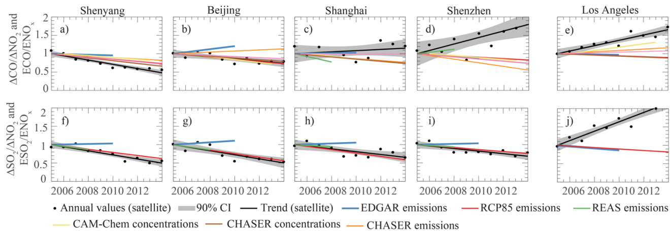
5 Figure 3: Changes in annual-mean enhancement ratios (black) from MOPITT and OMI retrievals of CO to NO 2 (top) and SO 2 to NO 2 (bottom) for select cities in China and U.S. relative to year 2005. Its associated emission ratios ((ECO/ENO x and ESO 2 /ENO x ) from RCP8.5 (red), EDGAR4.2 (blue) and top-down estimate from CHASER (orange) and model-simulated abundance ratios from CHASER (purple) and CAM-Chem (green) chemistry transport models are superimposed. Grey areas are 90% confidence intervals of the linear fit (black lines). The four Chinese cities represent the four classes/levels of urban development across 12 selected cities in China.
