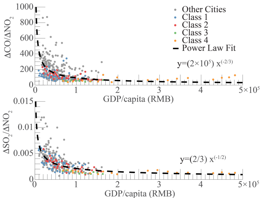
Figure 5: Annual-mean enhancement ratios (in units of mole/mole) of CO to NO 2 (panel a) and SO 2 to NO 2 (panel b) for all 36 provincial capitals and cities (2005 to 2014) as a function of its corresponding annual GDP/capita (in units of RMB/year/capita). The 12 select cities analyzed in this study are plotted in color, where each color represents four increasing levels or classes of urban development (e.g., Shenyang: Class 1, Beijing: Class 2, Shanghai: Class 3 and Shenzhen: Class 4). The rest of the 36 cities are plotted in gray. Superimposed on panel a) and b) is a fitted curve (black dashed line) based on power-law relationship of the data which is indicated in the plot by its corresponding equation.
