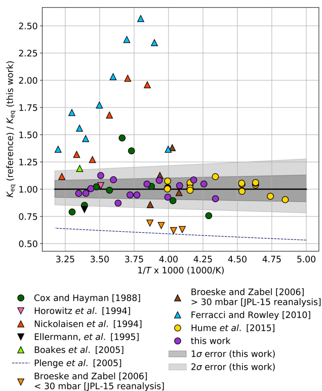
Figure 4. Ratio of K_{\text{eq}} values from prior laboratory studies to K_{\text{eq}} determined in this work ( K_{\text{eq}} = 2.16 \times 10^{-27} e^{(8533 \text{ K}/T)} \text{ cm}^3 \text{ molecule}^{-1} ) as a function of 1000/T . Circles indicate studies in which K_{\text{eq}} was measured with UV spectroscopy of equilibrium mixtures, while triangles indicate works in which K_{\text{eq}} was determined from individual reaction kinetic rates. Dark gray shading encompasses the total estimated 1\sigma error from this study and light shading encompasses the 2\sigma error.
