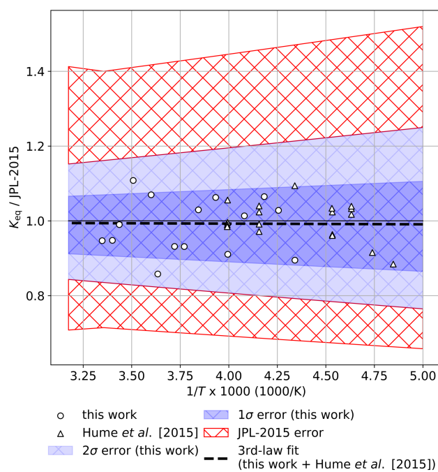
Figure 6. Ratio of third law fit of K_{\text{eq}} (black dashed line) determined from a combination of this work (circles) and Hume et al. (2015) (triangles) to the JPL compendium recommended value (Burkholder et al. , 2015). Error intervals as reported in this work (darker blue = 1\sigma , lighter blue = 2\sigma ) and as recommended by JPL-2015 (red cross hatch).
