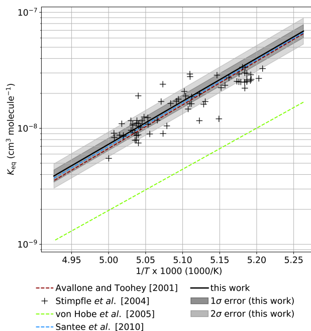
Figure 5. Comparison of extrapolated K_{\text{eq}} values from this work to atmospheric observations. K_{\text{eq}} (solid black) and error boundaries (gray shaded regions) determined in this study are extrapolated to the temperature range of 190 – 203 K. Expressions for K_{\text{eq}} derived from previous atmospheric measurements are presented as dashed lines. Observations of [\text{ClOOCl}] / [\text{ClO}]^2 from the nighttime ER-2 flight on 3 Feb 2000 in the SOLVE/THESEO mission out of Kiruna, Sweden are indicated as black crosses.
