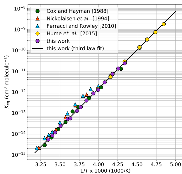
Figure 3. K_{\text{eq}} values as a function of 1000/T . Data from this work are plotted as purple circles; multiple samples are binned and averaged in 5 K intervals as shown in Table 1. The black line is a third law fit of the purple circles, K_{\text{eq}} = 2.16 \times 10^{-27} e^{(8533 \text{ K}/T)} \text{ cm}^3 \text{ molecule}^{-1} . The colored markers are K_{\text{eq}} values from prior laboratory studies as reported in the literature.
