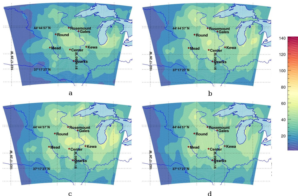
Figure 5. Filtered variances of in situ CO 2 mole fractions (about 100m agl) (in ppm 2 ) using 25 members (upper left panel), 10 members (upper right panel), 8 members (lower left panel), and 5 members (lower right panel).
