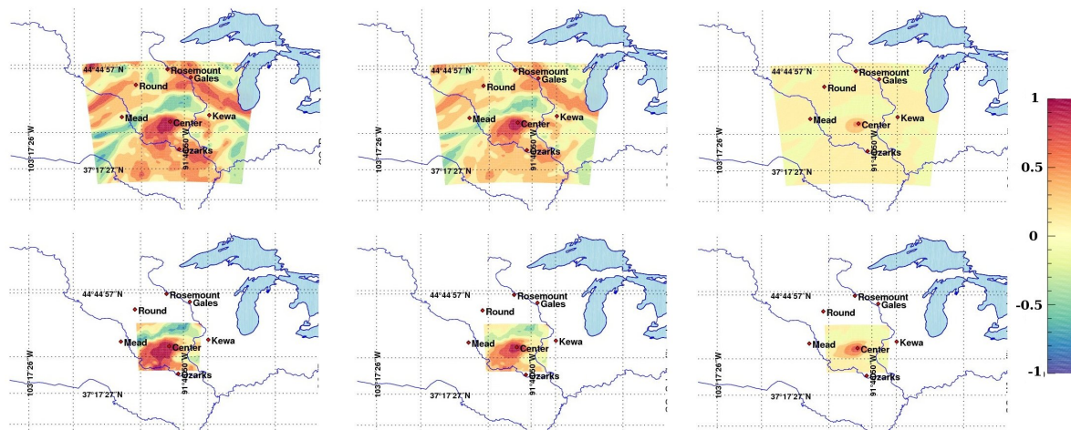
Figure 7. Hourly raw (left column) and filtered correlations using Schur (middle column) and Wiener (right column) filtered correlations of in situ \text{CO}_2 mole fractions at the Centerville tower (at about 100m agl) on June 26, 2008. The correlations are based on the original 45-member ensemble (top row) with a large subdomain ( 900 \times 900 \text{ km}^2 ) and the 25-member ensemble (bottom row) over the reference subdomain ( 400 \times 400 \text{ km}^2 ). The highlighted domain also corresponds to the domain used for the spatial averaging of the correlations in the optimality conditions.
