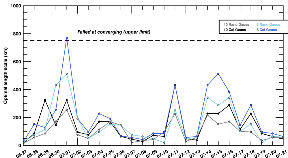
Figure 11. Length scale (in km) of the variance filter for 10-member random (in grey) and calibrated (in black) ensembles, and 8-member random (in light blue) and calibrated (royal blue) ensembles, for in situ CO 2 mole fractions at about 100m agl using Gaussian equations from 27 June to 21 July, 2008.
