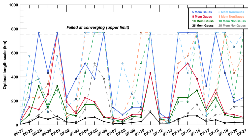
Figure 2. Length scale (in km) of the variance filter for in situ CO 2 mole fractions at about 100m agl using Gaussian (solid lines) and non-Gaussian (dash lines) equations from 27 June to 21 July, 2008.
