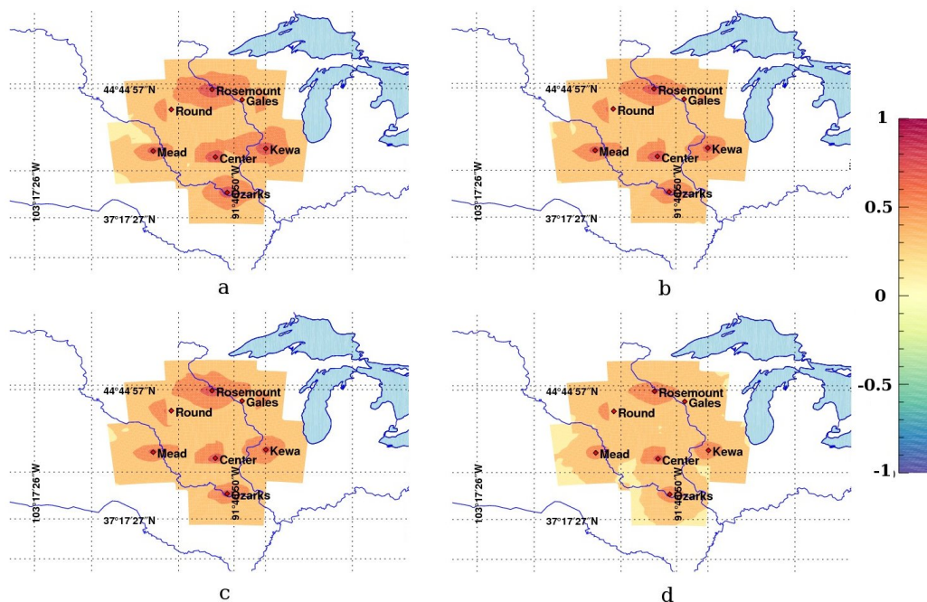
Figure 10. Filtered correlations (using Wiener & Schur product) of CO 2 in situ mole fractions (about 100m agl) (in ppm 2 ) (about 100m agl) (in ppm 2 ) using 25 members (upper left panel), 10 members (upper right panel), 8 members (lower left panel), and 5 members (lower right panel).
