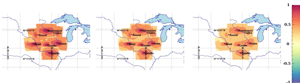
Figure 8. Raw (left panel) and filtered correlations of \text{CO}_2 in situ mole fractions at about 100m agl based on 25 members using the Schur localization (middle panel) and Wiener and Schur filter (right panel).
