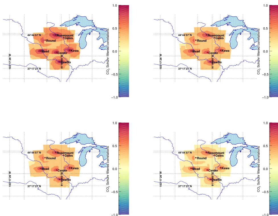
Figure 9. Filtered correlations (using Schurr product only) of \text{CO}_2 in situ mole fractions (about 100m agl) (in \text{ppm}^2 ) (about 100m agl) (in \text{ppm}^2 ) using 25 members (upper left panel), 10 members (upper right panel), 8 members (lower left panel), and 5 members (lower right panel).
