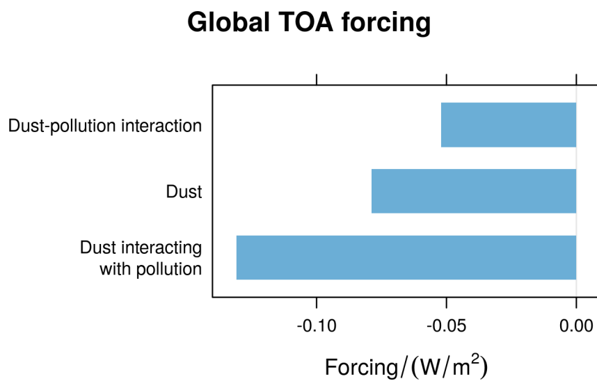
Figure 7. Global mean top of the atmosphere (TOA) forcing of the dust-pollution interaction in comparison with the mineral dust forcing from the same EMAC simulation excluding/including the dust-pollution interaction. The CVs of the interannual variation are (from top to bottom) 7 %, 6 % and 5 %.
