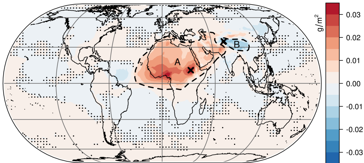
Figure 1. Impact of dust-pollution interaction on the coarse mode (top) and accumulation mode (bottom) aerosol burden (including aerosol water). The more efficient removal of aged dust particles reduces the coarse mode burden throughout the dust belt. This in turn reduces the coagulation efficiency of coarse mode with smaller particles, increasing the accumulation mode burden especially where the dust and the African biomass burning regions coincide. The strong hygroscopic growth of aged Saharan dust particles over the western Atlantic results in a regional maximum of the coarse mode burden increase. Generally, the hygroscopic growth of accumulation mode particles is reduced by the interaction with mineral dust cations manifested in a decreased accumulation mode burden over Tibet. The burdens over points A and B (crosses) are analysed in Fig. 2, relevant variables over regions A and B in Table 3 and Fig. S13. Dots indicate regions where the effect of the dust-pollution interaction is insignificant.
