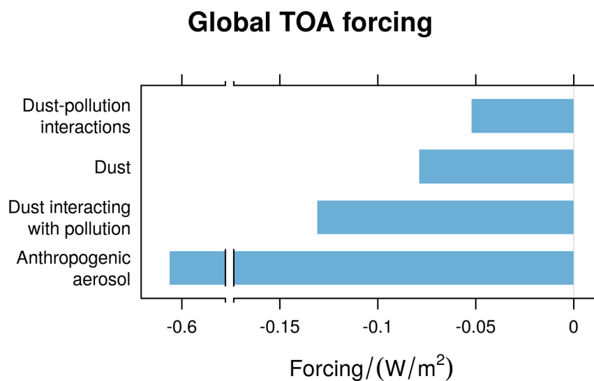
Figure 7. Global mean top of the atmosphere (TOA) forcing of the dust-pollution interaction interactions in comparison with the mineral dust forcing from the same EMAC simulation excluding/including the dust-pollution interaction interactions , and the anthropogenic aerosol forcing . The CVs of the interannual variation are (from top to bottom) 7 %, 6 % and , 5 % and 2 % .
