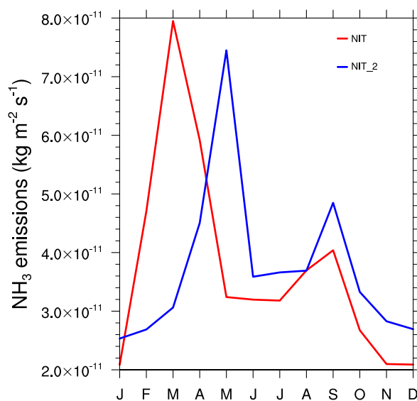
Figure 2. 1979-2016 monthly means of NH 3 emissions (kg m -2 s -1 ) over Europe as defined in Figure 1, used for NIT (red, based on MACCity) and NIT_2 (blue, from CMIP6) simulations. The annual total is equal in the two versions (4.5 10 -10 kg m -2 s -1 ).
