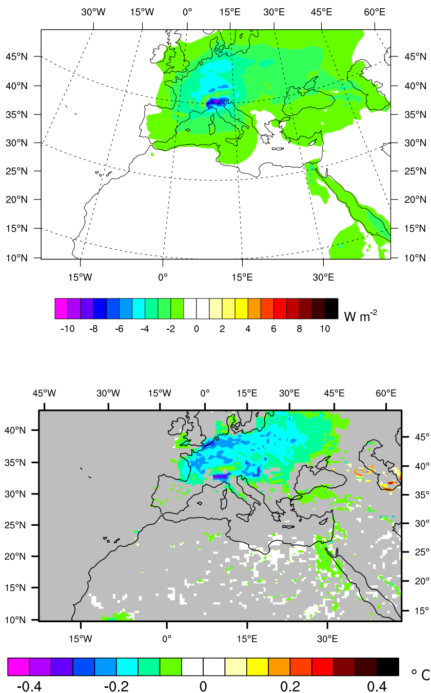
Figure 15. DRF SW ( \text{W m}^{-2} , top) at the surface in all sky conditions and the A&N aerosols impact on the near-surface air temperature at 2 m ( ^{\circ}\text{C} , bottom) on average over the period 1979-2016 in summer (JJA) obtained by difference between the REF and NIT simulations. For the temperature map, the grey area is not statistically significant at the 0.05 level.
