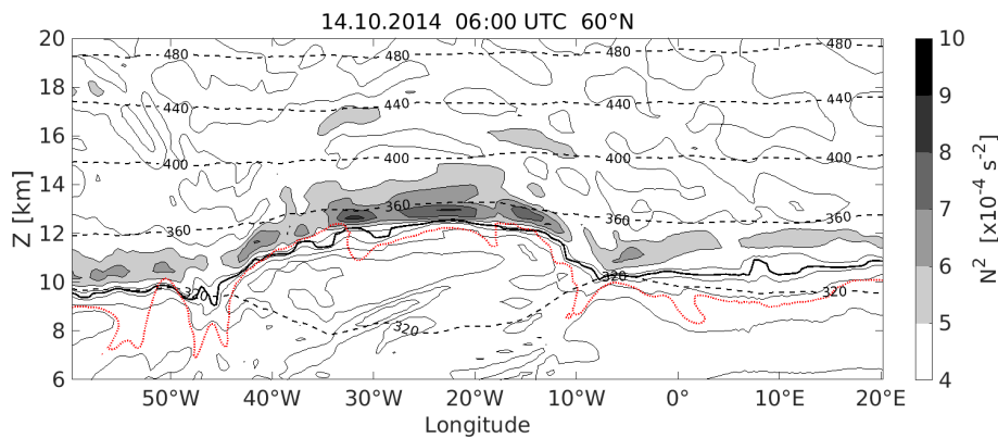
Figure R3. Vertical crosssection over the North Atlantic on 14.10.2014 at 06:00 UTC at 60^\circ N. The filled contour as well as the thin solid black contour lines show static stability N^2 in steps of 1 \times 10^{-4} \text{ s}^{-2} , dashed black lines show isentropes. The bold solid black line indicates the lapse rate tropopause, the dotted red line shows the 2 pvu isoline of potential vorticity.
