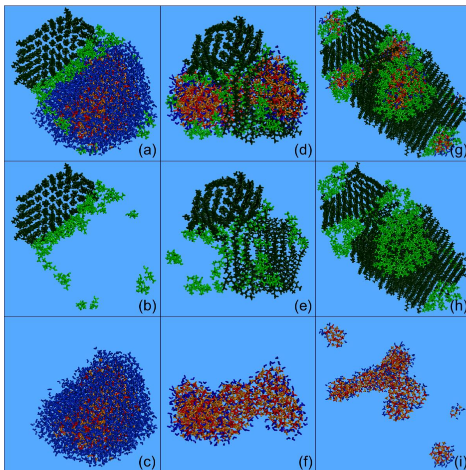
Figure 11. Characteristic snapshots from the MD simulations of the nanoparticle containing CPA and n -triacontane: (a) at 86 % RH (53 % dry organic content), (b) at 86 % RH (53 % organics) showing only organic molecules, (c) at 86 % RH (53 % organics) omitting organic molecules, (d) at 30 % RH (53 % dry organic content), (e) at 30 % RH (53 % organics) including only organic molecules, (f) at 30 % RH (53 % organics) omitting organic molecules, (g) at 18 % RH (82 % dry organic content), (h) at 18 % RH (82 % organics) including only organic molecules, and (i) at 18 % RH (82 % organics) omitting organic molecules. Colour coding: green for CPA, dark green for n -triacontane, red for sulfate, orange for ammonium, and blue for water.
