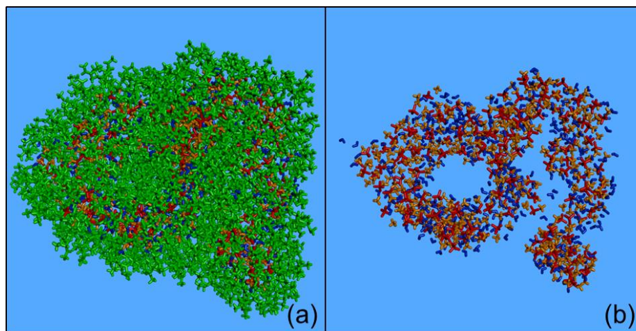
Figure 6. Characteristic snapshot from the MD simulation of the nanoparticle containing CPA (74 % dry) at 20 % RH, (a) including and (b) omitting CPA molecules. Colour coding: green for CPA, red for sulfate, orange for ammonium, and blue for water.
