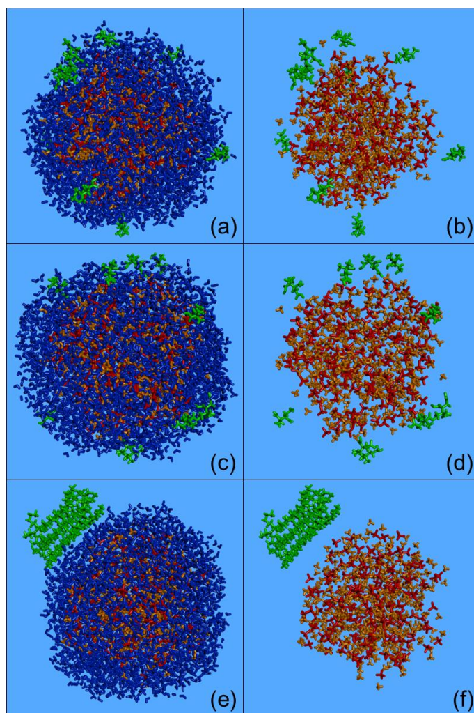
Figure 4. Characteristic snapshots from the MD simulations of the nanoparticles containing CPA (a–b), MBTCA (c–d), and n -icosane (e–f) at low organic mass fraction (7–10 %) and 88 % RH, including (a, c, e) and omitting (b, d, f) water molecules. Colour coding: green for CPA, MBTCA, and n -icosane, red for sulfate, orange for ammonium, and blue for water.
