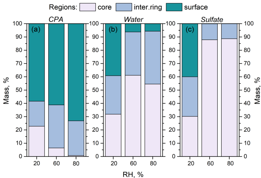
Figure 8. Percentage of: (a) CPA molecules, (b) water molecules and (c) sulfate ions in the three regions (core, intermediate ring, outer surface) of the simulated nanoparticles, as a function of RH. The dry organic mass content is 74 %.
