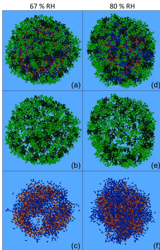
Figure 10. Characteristic snapshots from the MD simulations of the nanoparticles containing (dry mass fraction) 36 % CPA and 39 % MBTCA (a) at 67 % RH, (b) at 67 % RH including only organic molecules, (c) at 67 % RH omitting organic molecules, (d) at 80 % RH, (e) at 80 % RH including only organic molecules, and (f) at 80 % RH omitting organic molecules. Colour coding: green for CPA, dark green for MBTCA, red for sulfate, orange for ammonium, and blue for water.
