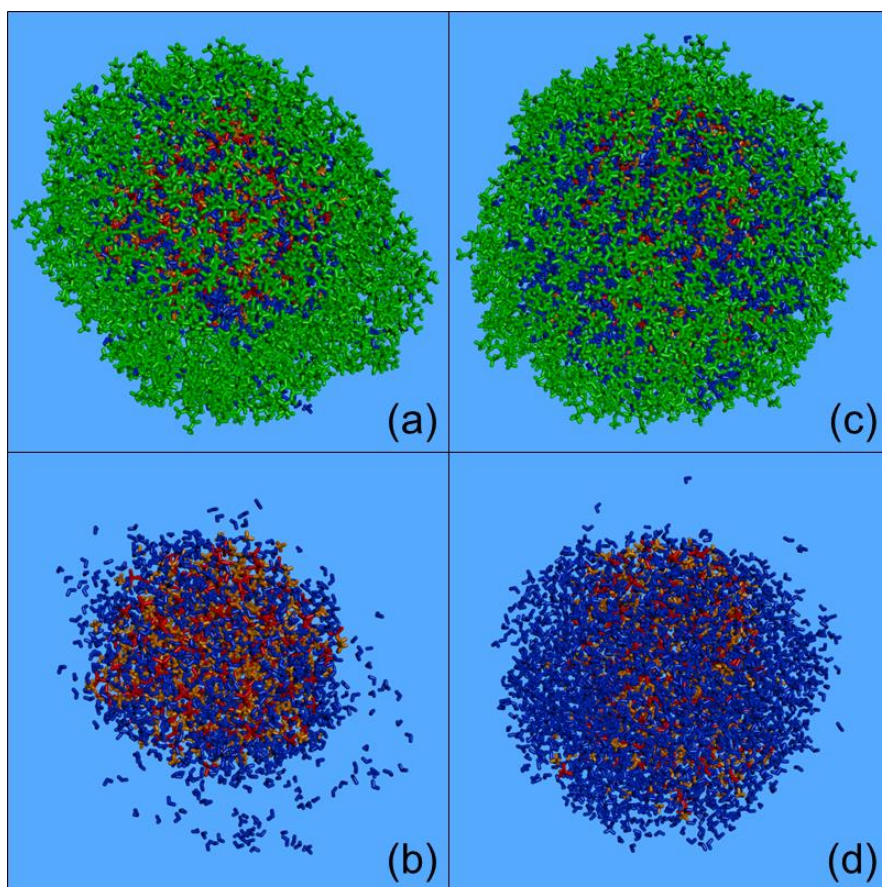
Figure 9. Characteristic snapshots from the MD simulation of the nanoparticles containing CPA (74 % dry): (a) at 60 % RH including CPA molecules, (b) at 60 % 5 RH omitting CPA molecules, (c) at 80 % RH including CPA molecules, and (d) at 80 % RH omitting CPA molecules. Colour coding: green for CPA, red for sulfate, orange for ammonium, and blue for water.
