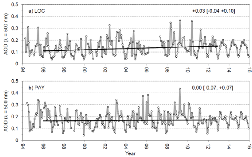
10 Figure 3: Time series of monthly AOD averages ( \lambda = 500 \text{ nm} ) available since 1994 at: a) LOC and b) PAY. The 1996 – 2012 decadal trend is shown in the top right-hand corner where values in brackets represent the upper and lower bounds of the 90 % confidence interval. Trend values are only calculated for observations during 1996 – 2013, and a climatology (1996 – 2012) was used for the 2013 – 2015 period. See text for further details.
