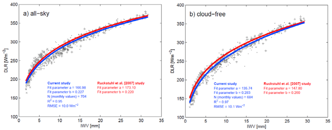
Figure 4: Monthly average DLR at all four stations (symbols: LOC = plus symbols, PAY = closed circles, DAV = open circles, and JFJ = crosses) for the 2000 – 2015 period versus IWV values during: a) all-sky conditions, and b) cloud-free conditions.
