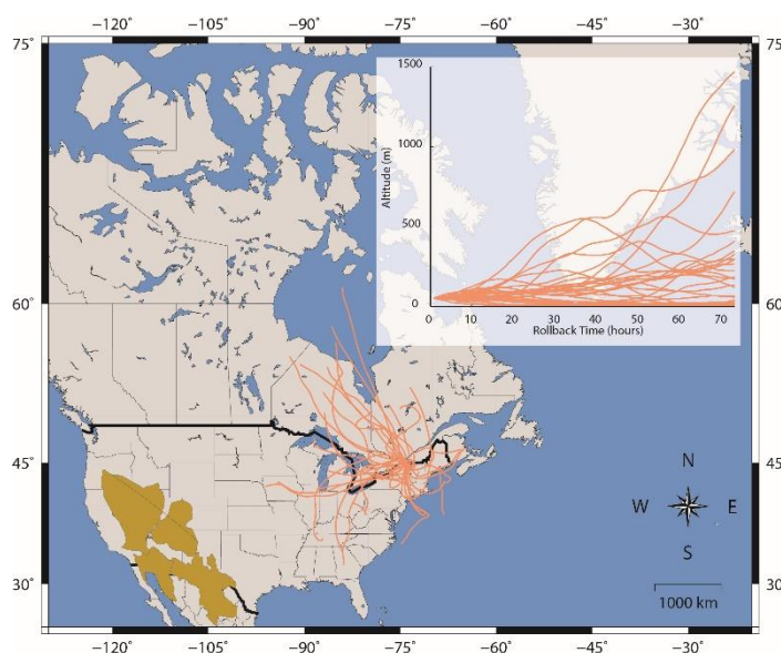
20 Figure 4 : Three-days back-trajectories modelled using the HYSPLIT software for the sampling stations in Montreal. Back trajectories are calculated using an initial height of 50 m above the sea level. American deserts are also shown in brown and include the Great Basin, the Mohave desert, the Chihuahua desert and the Sonoran desert.
