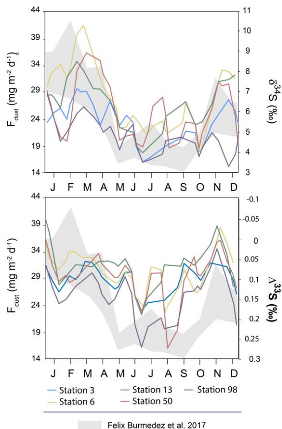
15 Figure 5 : Variations of the mean \delta^{34}\text{S} and \Delta^{33}\text{S} -values over time in sulfate aerosols collected in Montreal. The grey band represents the seasonality of the dust deposition rate determined by Félix-Bermúdez et al. (2017)
