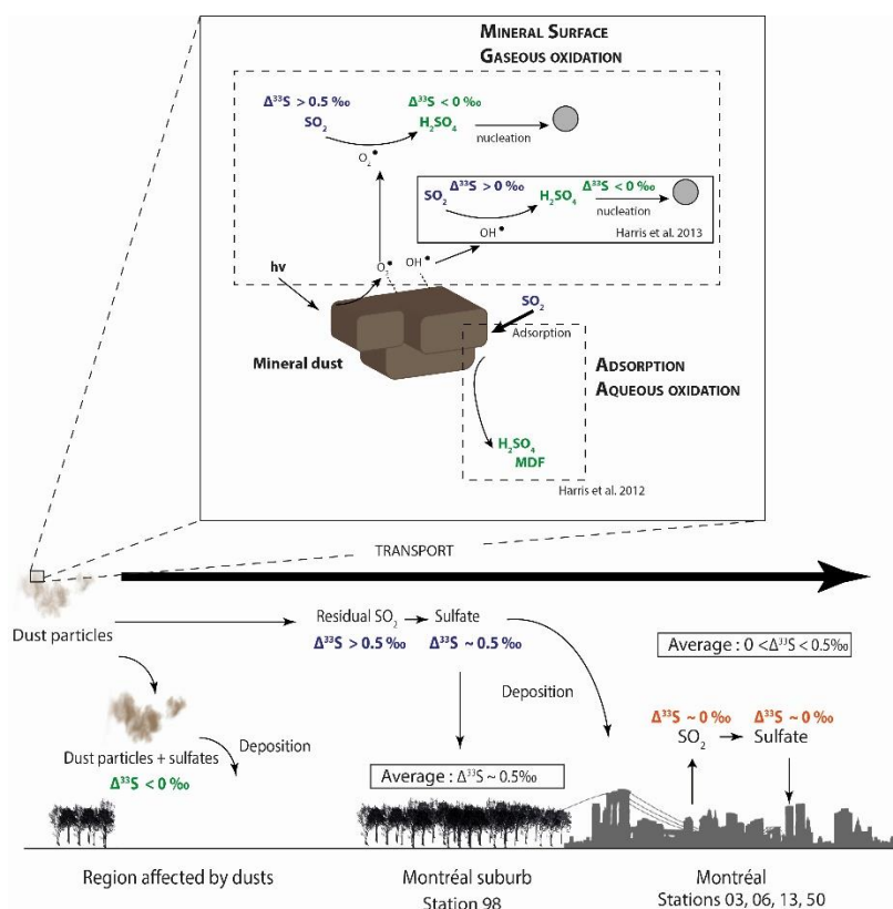
15 Figure 6 : Scheme of the reaction mechanisms leading to the formation of sulfates (modified from Dupart et al. (2012)) driven by airborne mineral dust. The ^{33}\text{S} enriched residual \text{SO}_2 is supposedly transported to cities while the ^{33}\text{S} depleted sulfates is deposited along with dust particles in the rural environment. The dotted lines would depend on the meteorological conditions, which could transport dust particles and sulfates into the city.
