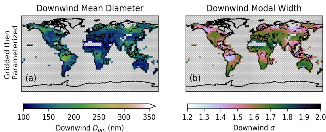
5 Figure 3: Annual-mean median diameter (a) and modal width (b) for sub-grid-processed biomass burning emissions predicted for 2010 using the Sakamoto et al. (2016) parameterization after 24 hours of sub-grid coagulation with an emitted median diameter of 100 nm and an emitted modal width of 2. Fire (FINNv1.5) and meteorological data is averaged over a 4°x5° grid and then that gridded data is run through the Sakamoto et al. (2016) parameterization. The regions with grey cross-hatching are grid-cells with no fire data.
