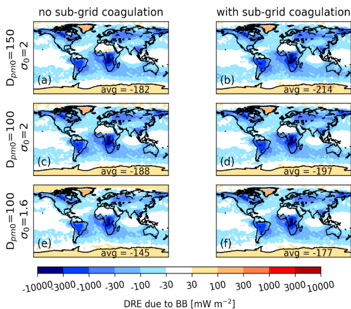
5 Figure 8: All-sky direct radiative effect (DRE) due to biomass burning aerosols using GFED emissions and the internal, core-shell mixing assumption. Panels (a), (c), and (e) are without sub-grid coagulation ( DI50_noSubCoag , noSubCoag , and s1.6_noSubCoag , respectively). Panels (b), (d), and (f) are with sub-grid coagulation ( DI50_SubCoag , SubCoag , and s1.6_SubCoag , respectively). Panels (a) and (b) have an emitted median diameter of 150 nm and an emitted modal width of 2. Panels (c) and (d) have an emitted median diameter of 100 nm and an emitted modal width of 2. Panels (e) and (f) have an emitted median diameter of 100 nm and an emitted modal width of 1.6. The number in the bottom right of each panel is the global mean DRE value [ \text{mW m}^{-2} ]. 10
