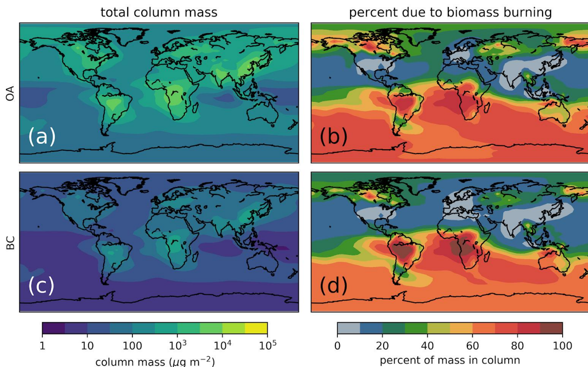
Figure 1: Effect of biomass burning on annually averaged total column OA and BC mass concentrations. The left side shows the total column mass concentration of (a) OA and (c) BC in the simulations with GFED biomass burning emissions (i.e., noSubCoag ). The right side shows the percent of the mass in the column that is due to biomass burning emissions for (b) OA and (d) BC by taking the difference between the noSubCoag and noBB simulations.
