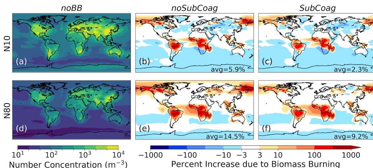
Figure 2: Effect of biomass burning on surface-level number concentration of particles larger than 10 nm (a, b, c) and 80 nm (d, e, f). Panels (a) and (d) show the absolute number concentration for the noBB simulation. Panels (b) and (e) show the percent increase due to GFED biomass burning emissions from the noBB simulation to the noSubCoag simulation. Panels (c) and (f) show the percent increase due to GFED biomass burning emissions from the noBB simulation to the SubCoag simulation. The number in the bottom right of each panel is the global mean percent increase due to biomass burning.
