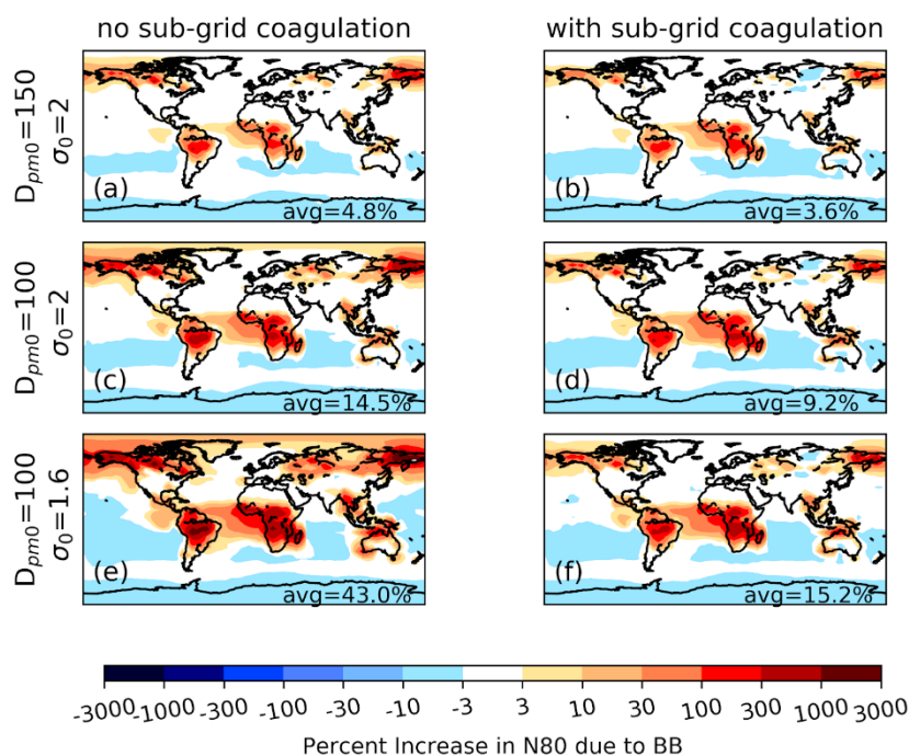
5 Figure 4: Annual-average percent changes in N80 at the surface level due to the inclusion of GFED biomass burning emissions relative to the simulation without biomass burning ( noBB ). Panels (a), (c), and (e) have no sub-grid coagulation ( D150_noSubCoag , noSubCoag , and s1.6_noSubCoag , respectively). Panels (b), (d), and (f) have sub-grid coagulation ( D150_SubCoag , SubCoag , and s1.6_SubCoag , respectively). Panels (a) and (b) have an emitted median diameter of 150 nm and an emitted modal width of 2. Panels (c) and (d) have an emitted median diameter of 100 nm and an emitted modal width of 2. Panels (e) and (f) have an emitted median diameter of 100 nm and an emitted modal width of 1.6. The number in the bottom right of each panel is the global mean percent increase in N80 due to biomass burning.
