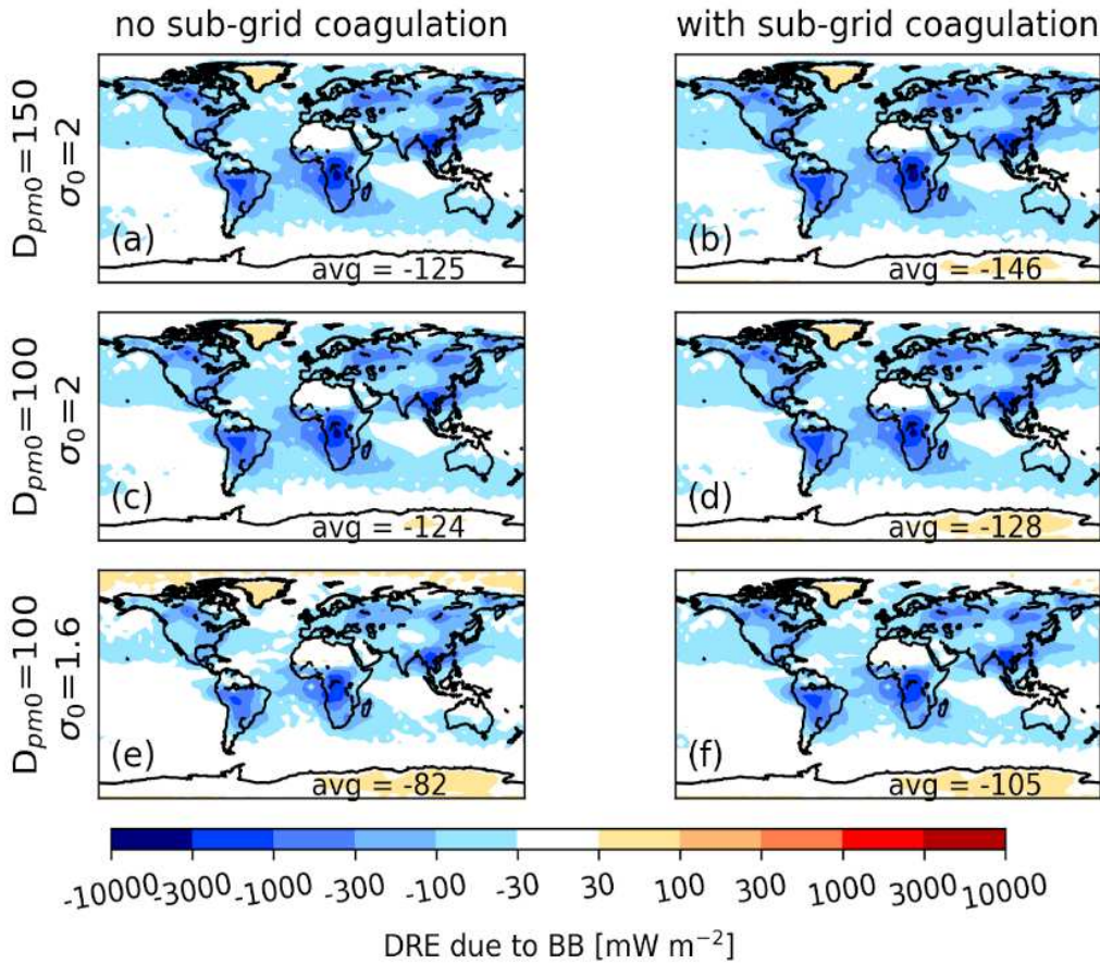
Figure S127: All-sky direct radiative effect (DRE) due to biomass burning aerosols using FINNv1 emissions and using the external-mixing assumption. Panels (a), (c), and (e) are without sub-grid coagulation ( DI50_noSubCoag_FINN , noSubCoag_FINN , and s1.6_noSubCoag_FINN , respectively). Panels (b), (d), and (f) are with sub-grid coagulation ( DI50_SubCoag_FINN , SubCoag_FINN , and s1.6_SubCoag_FINN , respectively). Panels (a) and (b) have an emitted median diameter of 150 nm and an emitted modal width of 2. Panels (c) and (d) have an emitted median diameter of 100 nm and an emitted modal width of 2. Panels (e) and (f) have an emitted median diameter of 100 nm and an emitted modal width of 1.6. The number in the bottom right of each panel is the global mean DRE value [ \text{mW m}^{-2} ].
