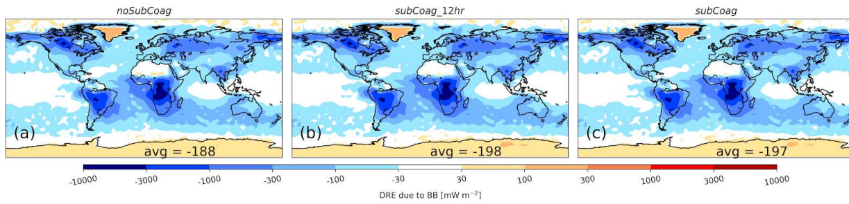
Figure S2143: All-sky direct radiative effect due to biomass burning aerosols using GFED emissions and the internal, core-shell mixing assumption. On the left, there is no sub-grid coagulation ( noSubCoag ). In the middle, the sub-grid coagulation time is 12 hours ( SubCoag_12h ). On the right, the sub-grid coagulation time is 24 hours ( SubCoag ). The number in the bottom right corner of each panel is the global mean value [ \text{mW m}^{-2} ].
