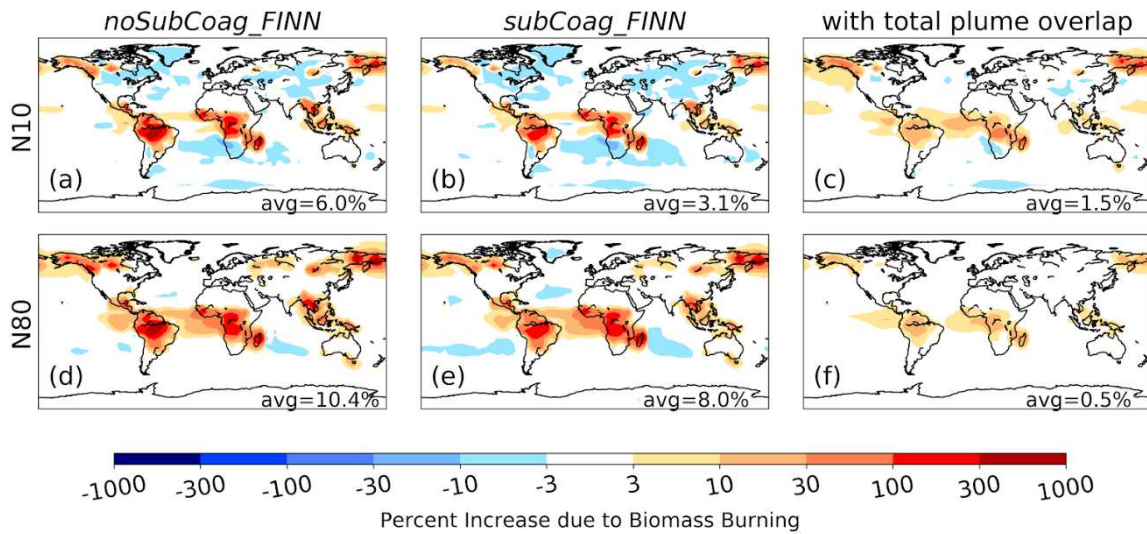
Figure S180: Effect of biomass burning on surface-level N10 (a-c) and N80 (d-f) under three sub-grid coagulation conditions. Panels (a) and (d) show the noSubCoag_FINN case (no sub-grid coagulation). Panels (b) and (e) show the SubCoag_FINN case (with sub-grid coagulation as in the rest of the paper, where the smoke plumes are treated as without overlap). Panels (c) and (f) show a new case where all smoke plumes in the gridbox completely overlap and form a single “superplume” upon emission into the sub-grid coagulation parameterization. All panels show the percent increase due to FINNv1 biomass burning emissions relative to the noBB simulation. The number in the bottom right of each panel is the global mean percent increase due to biomass burning.
