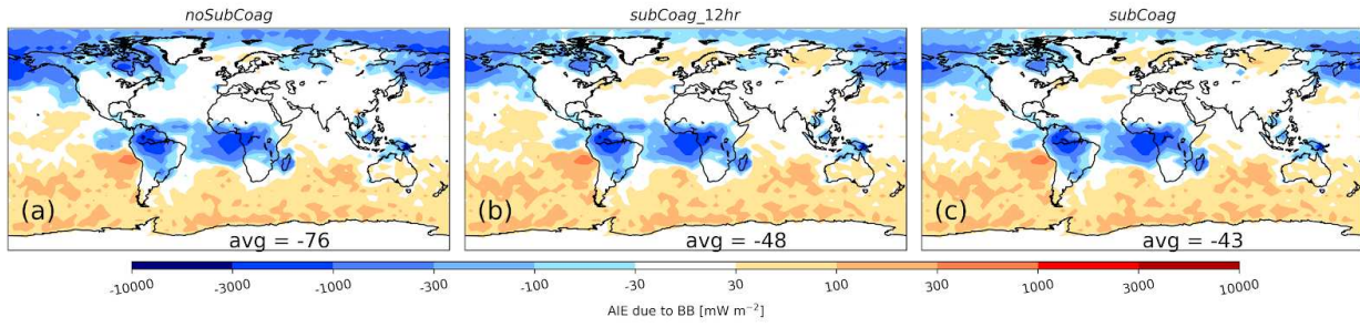
Figure S2214: Cloud-albedo aerosol indirect effect due to biomass burning aerosols using GFED emissions. On the left, there is no sub-grid coagulation ( noSubCoag ). In the middle, the sub-grid coagulation time is 12 hours ( SubCoag_12h ). On the right, the sub-grid coagulation time is 24 hours ( SubCoag ). The number in the bottom right corner of each panel is the global mean value [ \text{mW m}^{-2} ].
