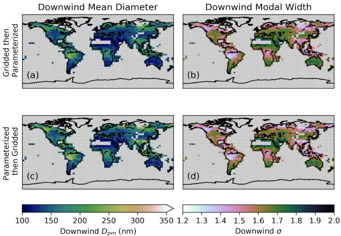
Figure S32: Annual-mean median diameter (a and, c) and modal width (b and, d) for biomass burning emissions predicted for 2010 using the Sakamoto et al. (2016) parameterization after 24 hours of sub-grid coagulation with an emitted initial median diameter of 100 nm and an emitted initial modal width of 2. Panels (a) and (b) show the resulting D_{pm} and \sigma when the fire (FINNv1.5) and meteorological data is averaged over a 4^\circ \times 5^\circ grid and then that gridded data is run through the Sakamoto et al. (2016) parameterization. Panels (c) and (d) show the results when the individual fires are run through the Sakamoto et al. (2016) parameterization and then the output D_{pm} and \sigma are averaged over a 4^\circ \times 5^\circ grid. The regions with grey cross-hatching are grid-cells with no fire data.
