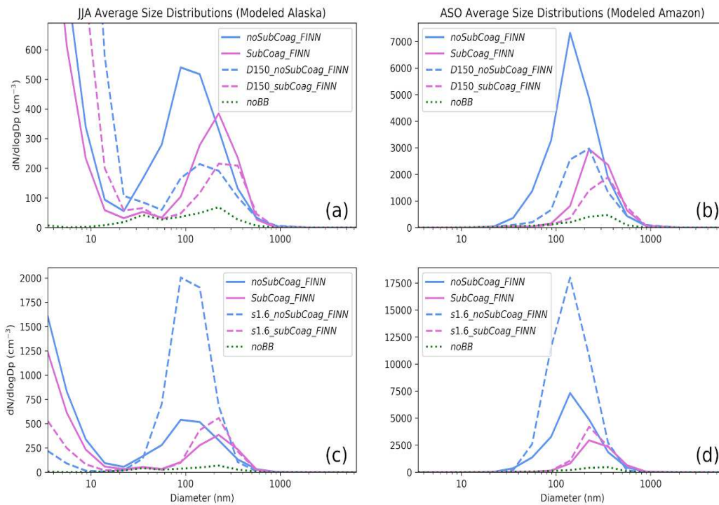
Figure S116: Predicted grid-resolved aerosol size distributions with FINNv1 biomass burning emissions over Alaska at 62° N, 140° W, averaged over the June, July, and August fire season (a and c) and the Amazon at 6° S, 60° E, averaged over the August, September, and October fire season (b and d). All panels show the size distributions for the noBB , noSubCoag_FINN , and SubCoag_FINN simulations in the dashed green, solid blue, and solid pink lines, respectively. The top panels (a and b) show the sensitivity to the emitted median diameter, and the bottom panels (c and d) show the sensitivity to the emitted modal width. Note the different y-axis scales.
