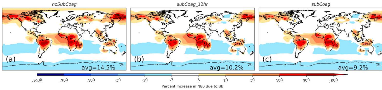
Figure S194: Annual-average percent changes in N80 at the surface level due to the inclusion of GFED biomass burning emissions relative to the simulation without biomass burning ( noBB ). On the left, there is no sub-grid coagulation ( noSubCoag ). In the middle, the sub-grid coagulation time is 12 hours ( SubCoag_12h ). On the right, the sub-grid coagulation time is 24 hours ( SubCoag ). The number in the bottom right corner of each panel is the global mean percent increase in N80 due to biomass burning.
