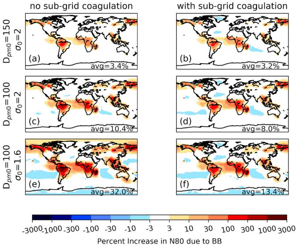
Figure S95: Annual-average percent changes in N80 at the surface level due to the inclusion of FINNv1 biomass burning emissions relative to the simulation without biomass burning ( noBB ). Panels (a), (c), and (e) have no sub-grid coagulation ( D150_noSubCoag_FINN , noSubCoag_FINN , and s1.6_noSubCoag_FINN , respectively). Panels (b), (d), and (f) have sub-grid coagulation ( D150_SubCoag_FINN , SubCoag_FINN , and s1.6_SubCoag_FINN , respectively). Panels (a) and (b) have an emitted median diameter of 150 nm and an emitted modal width of 2. Panels (c) and (d) have an emitted median diameter of 100 nm and an emitted modal width of 2. Panels (e) and (f) have an emitted median diameter of 100 nm and an emitted modal width of 1.6. The number in the bottom right of each panel is the global mean percent increase in N80 due to biomass burning.
