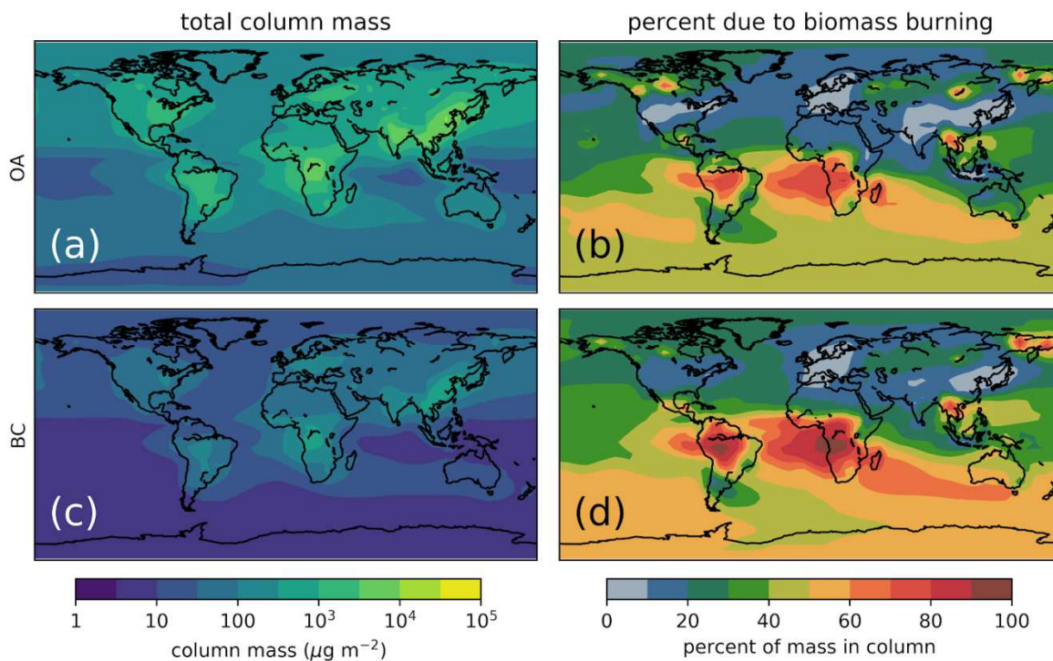
Figure S63: Effect of biomass burning on annually averaged total column OA and BC mass concentrations. The left side shows the total column mass concentration of (a) OA and (c) BC in the simulations with FINNv1 biomass burning emissions (i.e., noSubCoag_FINN ). The right side shows the percent of the mass in the column that is due to biomass burning emissions for (b) OA and (d) BC by taking the difference between the noSubCoag_FINN and noBB simulations.
