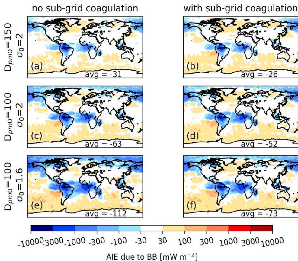
Figure S169: Cloud-albedo aerosol indirect effect (AIE) due to biomass burning aerosols using FINNv1 emissions. Panels (a), (c), and (e) are without sub-grid coagulation ( D150_noSubCoag_FINN , noSubCoag_FINN , and s1.6_noSubCoag_FINN , respectively). Panels (b), (d), and (f) are with sub-grid coagulation ( D150_SubCoag_FINN , SubCoag_FINN , and s1.6_SubCoag_FINN , respectively). Panels (a) and (b) have an emitted median diameter of 150 nm and an emitted modal width of 2. Panels (c) and (d) have an emitted median diameter of 100 nm and an emitted modal width of 2. Panels (e) and (f) have an emitted median diameter of 100 nm and an emitted modal width of 1.6. The number in the bottom right of each panel is the global mean AIE value [ \text{mW m}^{-2} ].
