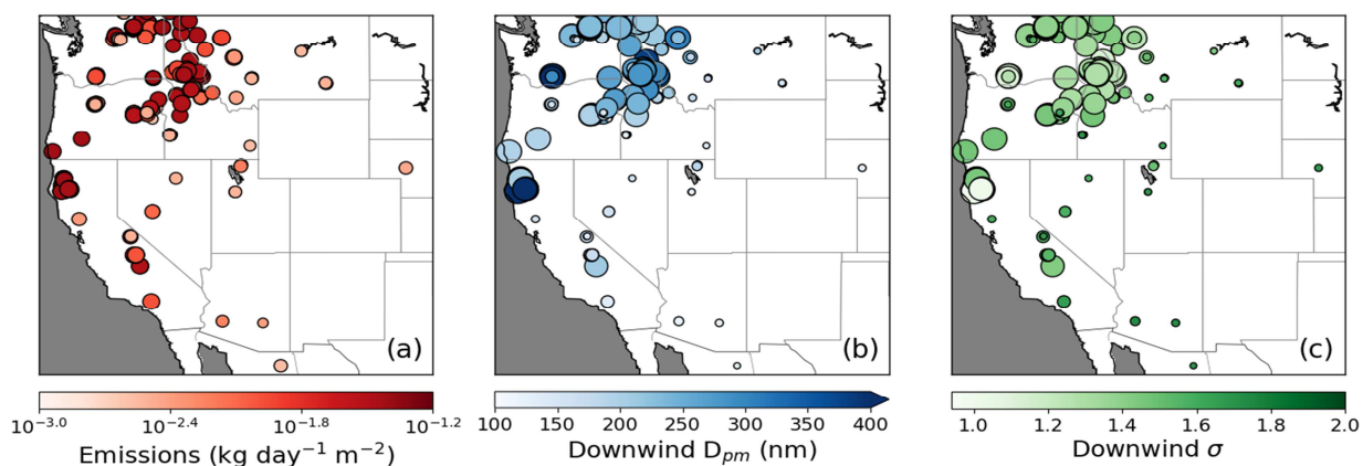
Figure S1: Demonstration of the effect of per-fire coagulation parameterization on all the fires in the Western US on 15 August 8/15/2015 from FINNv1.5. The emissions of OA and BC are indicated in the color in (a) and in the size of the markers in (b) and (c). In (a) the size indicated the area of the fire. In (b) and (c) the color indicates the median diameter and modal width, respectively, after 24 hours of coagulation where the emitted median diameter is 100 nm and the emitted modal width is 2.
