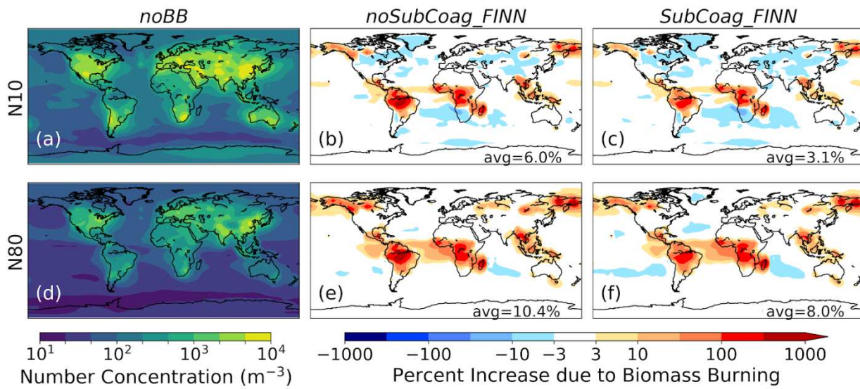
Figure S74: Effect of biomass burning on surface-level number concentration of particles above 10 nm (a, b, c) and 80 nm (d, e, f). Panels (a) and (d) show the absolute number concentration for the noBB simulation. Panels (b) and (e) show the percent increase due to FINNv1 biomass burning emissions from the noBB simulation to the noSubCoag_FINN simulation. Panels (c) and (f) show the percent increase due to FINNv1 biomass burning emissions from the noBB simulation to the SubCoag_FINN simulation. The number in the bottom right of each panel is the global mean percent increase due to biomass burning.
