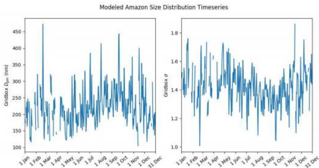
Figure S2: Daily temporal evolution of the predicted grid-resolved median diameter ( D_{pm} ; left) and modal width ( \sigma ; right) in a box that spans 8^\circ latitude and 10^\circ for biomass burning emissions predicted for 2010 using FINNv1.5 fire emissions and the Sakamoto et al. (2016) parameterization after 24 hours of sub-grid coagulation with an emitted initial median diameter of 100 nm and an emitted initial modal width of 2. The top plots are centered over Alaska at 62^\circ N, 135^\circ W. Times that are not shown have no fire data in this gridbox. The bottom plots are centered over the Amazon at 6^\circ S, 60^\circ W.
