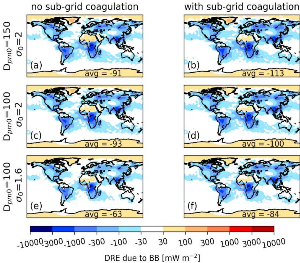
Figure S148: All-sky direct radiative effect (DRE) due to biomass burning aerosols using FINNv1 emissions and using the core-shell mixing assumption. Panels (a), (c), and (e) are without sub-grid coagulation ( D150_noSubCoag_FINN , noSubCoag_FINN , and s1.6_noSubCoag_FINN , respectively). Panels (b), (d), and (f) are with sub-grid coagulation ( D150_SubCoag_FINN , SubCoag_FINN , and s1.6_SubCoag_FINN , respectively). Panels (a) and (b) have an emitted median diameter of 150 nm and an emitted modal width of 2. Panels (c) and (d) have an emitted median diameter of 100 nm and an emitted modal width of 2. Panels (e) and (f) have an emitted median diameter of 100 nm and an emitted modal width of 1.6. The number in the bottom right of each panel is the global mean DRE value [ \text{mW m}^{-2} ].
