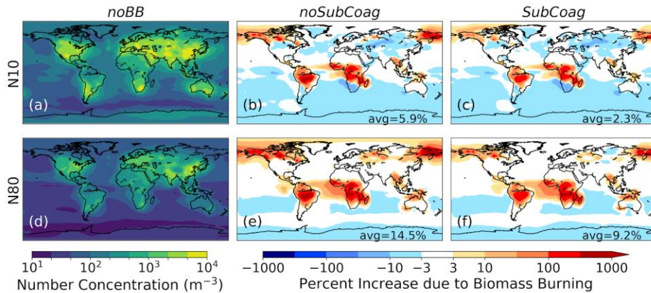
Figure 23: Effect of biomass burning on surface-level number concentration of particles larger than 10 nm (a, b, c) and 80 nm (d, e, f). Panels (a) and (d) show the absolute number concentration for the noBB simulation. Panels (b) and (e) show the percent increase due to GFED biomass burning emissions from the noBB simulation to the noSubCoag simulation. Panels (c) and (f) show the percent increase due to GFED biomass burning emissions from the noBB simulation to the SubCoag simulation. The number in the bottom right of each panel is the global mean percent increase due to biomass burning.
