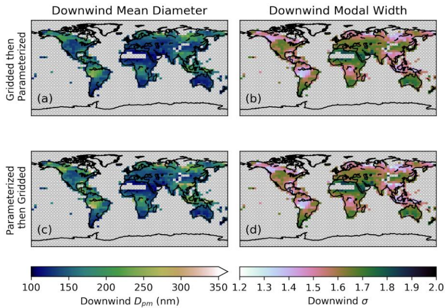
Figure S2S3: Annual-mean median diameter (a and, c) and modal width (b and, d) for biomass burning emissions predicted for 2010 using the Sakamoto et al. (2016) parameterization after 24 hours of sub-grid coagulation with an emitted initial median diameter of 100 nm and an emitted initial modal width of 2. Panels (a) and (b) show the resulting D_{pm} and \sigma when the fire (FINNv1.5) and meteorological data is averaged over a 4^\circ \times 5^\circ grid and then that gridded data is run through the Sakamoto et al. (2016) parameterization. Panels (c) and (d) show the results when the individual fires are run through the Sakamoto et al. (2016) parameterization and then the output D_{pm} and \sigma are averaged over a 4^\circ \times 5^\circ grid. The regions with grey cross-hatching are grid-cells with no fire data.
