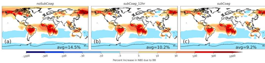
Figure S4S19: Annual-average percent changes in N80 at the surface level due to the inclusion of GFED biomass burning emissions relative to the simulation without biomass burning ( noBB ). On the left, there is no sub-grid coagulation ( noSubCoag ). In the middle, the sub-grid coagulation time is 12 hours ( SubCoag_12h ). On the right, the sub-grid coagulation time is 24 hours ( SubCoag ). The number in the bottom right corner of each panel is the global mean percent increase in N80 due to biomass burning.
