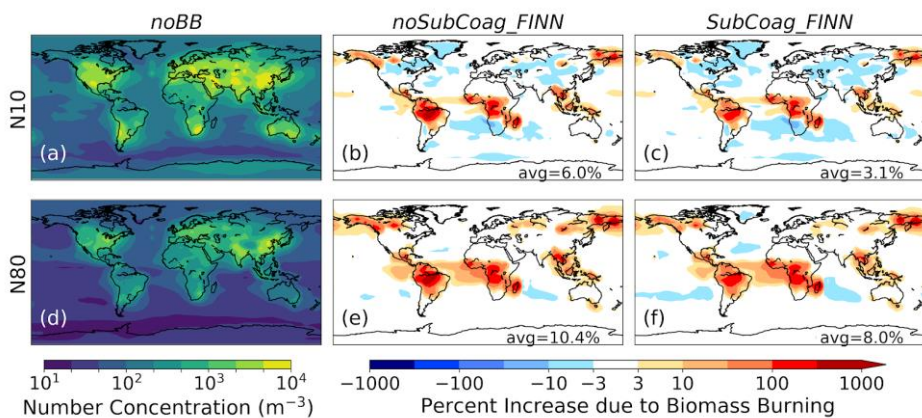
Figure S4S7: Effect of biomass burning on surface-level number concentration of particles above 10 nm (a, b, c) and 80 nm (d, e, f). Panels (a) and (d) show the absolute number concentration for the noBB simulation. Panels (b) and (e) show the percent increase due to FINNv1 biomass burning emissions from the noBB simulation to the noSubCoag_FINN simulation. Panels (c) and (f) show the percent increase due to FINNv1 biomass burning emissions from the noBB simulation to the SubCoag_FINN simulation. The number in the bottom right of each panel is the global mean percent increase due to biomass burning.
