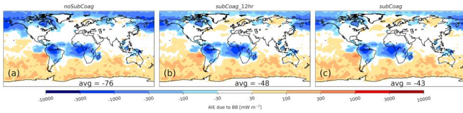
Figure S14S22: Cloud-albedo aerosol indirect effect due to biomass burning aerosols using GFED emissions. On the left, there is no sub-grid coagulation ( noSubCoag ). In the middle, the sub-grid coagulation time is 12 hours ( SubCoag_12h ). On the right, the sub-grid coagulation time is 24 hours ( SubCoag ). The number in the bottom right corner of each panel is the global mean value [ \text{mW m}^{-2} ].
