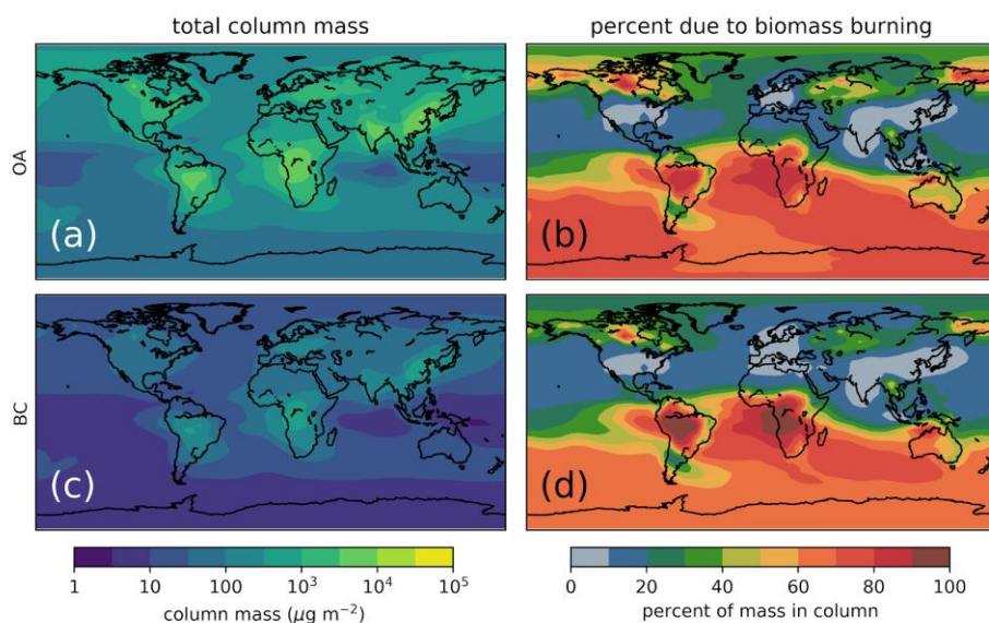
Figure 12: Effect of biomass burning on annually averaged total column OA and BC mass concentrations. The left side shows the total column mass concentration of (a) OA and (c) BC in the simulations with GFED biomass burning emissions (i.e., noSubCoag ). The right side shows the percent of the mass in the column that is due to biomass burning emissions for (b) OA and (d) BC by taking the difference between the noSubCoag and noBB simulations.
