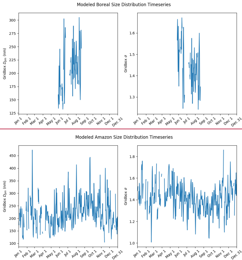
Figure S2: Daily temporal evolution of the predicted grid-resolved median diameter ( D_{pm} ; left) and modal width ( \sigma ; right) in a box that spans 8^\circ latitude and 10^\circ for biomass burning emissions predicted for 2010 using FINNv1.5 fire emissions and the Sakamoto et al. (2016) parameterization after 24 hours of sub-grid coagulation with an emitted initial median diameter of 100 nm and an emitted initial modal width of 2. The top plots are centered over Alaska at 62^\circ N, 135^\circ W. Times that are not shown have no fire data in this gridbox. The bottom plots are centered over the Amazon at 6^\circ S, 60^\circ E.
