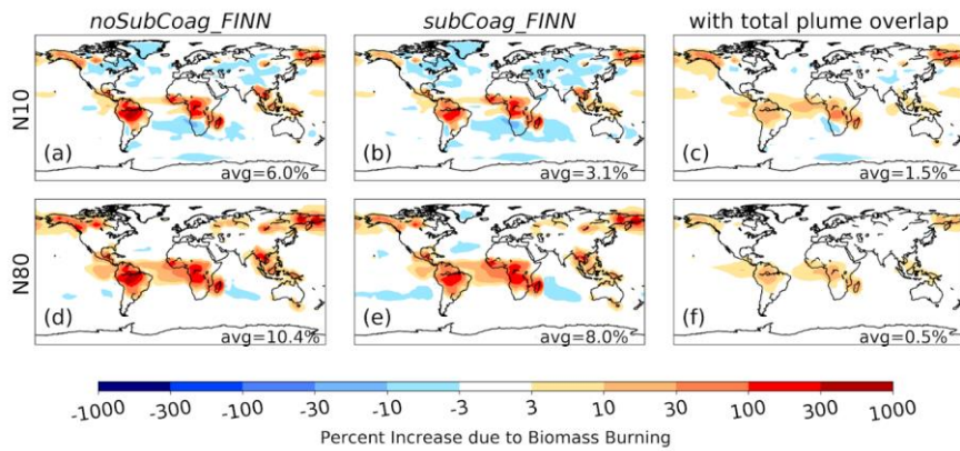
Figure S10S18: Effect of biomass burning on surface-level N10 (a-c) and N80 (d-f) under three sub-grid coagulation conditions. Panels (a) and (d) show the noSubCoag_FINN case (no sub-grid coagulation). Panels (b) and (e) show the SubCoag_FINN case (with sub-grid coagulation as in the rest of the paper, where the smoke plumes are treated as without overlap). Panels (c) and (f) show a new case where all smoke plumes in the gridbox completely overlap and form a single “superplume” upon emission into the sub-grid coagulation parameterization. All panels show the percent increase due to FINNv1 biomass burning emissions relative to the noBB simulation. The number in the bottom right of each panel is the global mean percent increase due to biomass burning.
