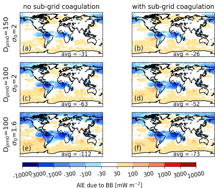
Figure S9S16: Cloud-albedo aerosol indirect effect (AIE) due to biomass burning aerosols using FINNv1 emissions. Panels (a), (c), and (e) are without sub-grid coagulation ( D150_noSubCoag_FINN , noSubCoag_FINN , and s1.6_noSubCoag_FINN , respectively). Panels (b), (d), and (f) are with sub-grid coagulation ( D150_SubCoag_FINN , SubCoag_FINN , and s1.6_SubCoag_FINN , respectively). Panels (a) and (b) have an emitted median diameter of 150 nm and an emitted modal width of 2. Panels (c) and (d) have an emitted median diameter of 100 nm and an emitted modal width of 2. Panels (e) and (f) have an emitted median diameter of 100 nm and an emitted modal width of 1.6. The number in the bottom right of each panel is the global mean AIE value [ \text{mW m}^{-2} ].
