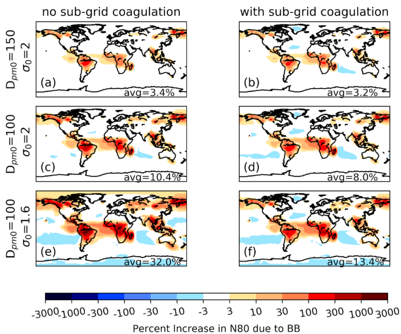
Figure S559: Annual-average percent changes in N80 at the surface level due to the inclusion of FINNv1 biomass burning emissions relative to the simulation without biomass burning ( noBB ). Panels (a), (c), and (e) have no sub-grid coagulation ( D150_noSubCoag_FINN , noSubCoag_FINN , and s1.6_noSubCoag_FINN , respectively). Panels (b), (d), and (f) have sub-grid coagulation ( D150_SubCoag_FINN , SubCoag_FINN , and s1.6_SubCoag_FINN , respectively). Panels (a) and (b) have an emitted median diameter of 150 nm and an emitted modal width of 2. Panels (c) and (d) have an emitted median diameter of 100 nm and an emitted modal width of 2. Panels (e) and (f) have an emitted median diameter of 100 nm and an emitted modal width of 1.6. The number in the bottom right of each panel is the global mean percent increase in N80 due to biomass burning.
