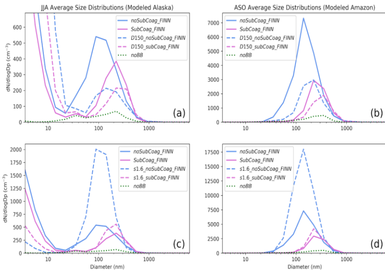
Figure S6S11: Predicted grid-resolved aerosol size distributions with FINNv1 biomass burning emissions over Alaska at 62° N, 140° W, averaged over the June, July, and August fire season (a and c) and the Amazon at 6° S, 60° E, averaged over the August, September, and October fire season (b and d). All panels show the size distributions for the noBB , noSubCoag_FINN , and SubCoag_FINN simulations in the dashed green, solid blue, and solid pink lines, respectively. The top panels (a and b) show the sensitivity to the emitted median diameter, and the bottom panels (c and d) show the sensitivity to the emitted modal width. Note the different y-axis scales.
