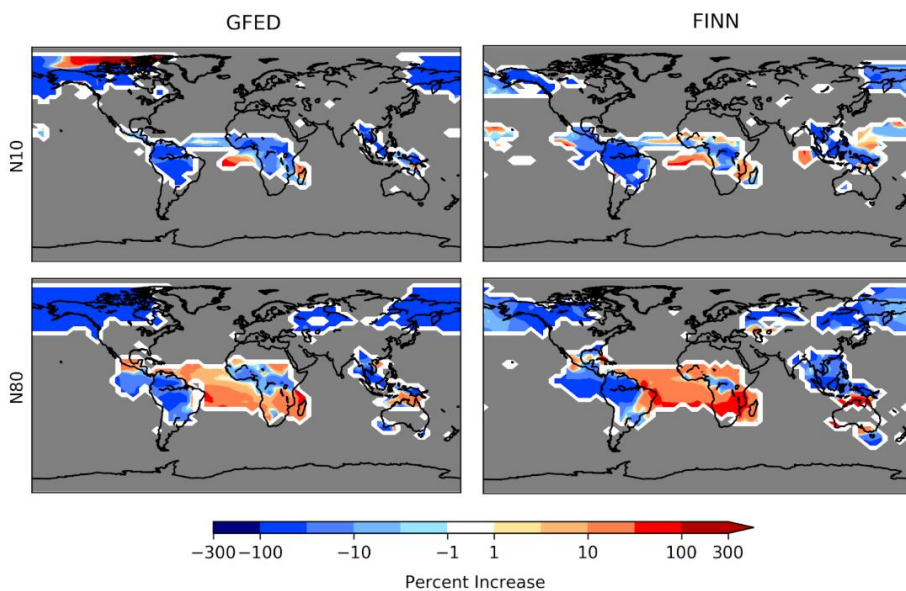
Figure S8: Percent change in the relative contribution of biomass burning to particles larger than 10 nm (N10) and particles larger than 80 nm (N80) due to sub-grid coagulation when using GFED emissions (left) or FINNv1 emissions (right), and an initial median diameter of 100 nm, initial modal width of 2, and coagulation time of 24 hours. Negative values correspond to a reduced impact of biomass burning when sub-grid coagulation is added. Regions where the percent increase of N10 or N80 due to biomass burning is less than 1% (with or without sub-grid coagulation, see Figs. 3 and S7) are shaded in grey.
