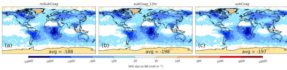
Figure S43S21: All-sky direct radiative effect due to biomass burning aerosols using GFED emissions and the internal, core-shell mixing assumption. On the left, there is no sub-grid coagulation ( noSubCoag ). In the middle, the sub-grid coagulation time is 12 hours ( SubCoag_12h ). On the right, the sub-grid coagulation time is 24 hours ( SubCoag ). The number in the bottom right corner of each panel is the global mean value [ \text{mW m}^{-2} ].
