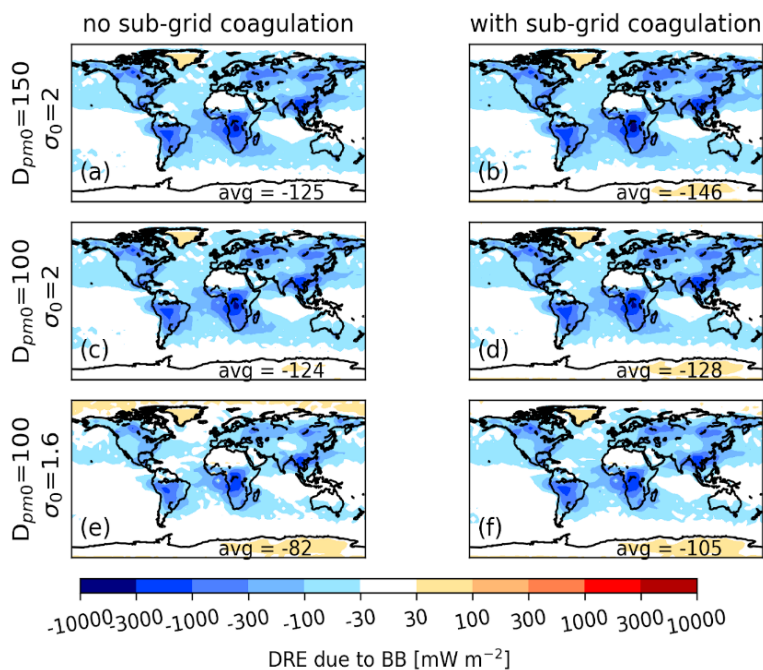
Figure S7S12: All-sky direct radiative effect (DRE) due to biomass burning aerosols using FINNv1 emissions and using the external-mixing assumption. Panels (a), (c), and (e) are without sub-grid coagulation ( D150_noSubCoag_FINN , noSubCoag_FINN , and s1.6_noSubCoag_FINN , respectively). Panels (b), (d), and (f) are with sub-grid coagulation ( D150_SubCoag_FINN , SubCoag_FINN , and s1.6_SubCoag_FINN , respectively). Panels (a) and (b) have an emitted median diameter of 150 nm and an emitted modal width of 2. Panels (c) and (d) have an emitted median diameter of 100 nm and an emitted modal width of 2. Panels (e) and (f) have an emitted median diameter of 100 nm and an emitted modal width of 1.6. The number in the bottom right of each panel is the global mean DRE value [ \text{mW m}^{-2} ].
