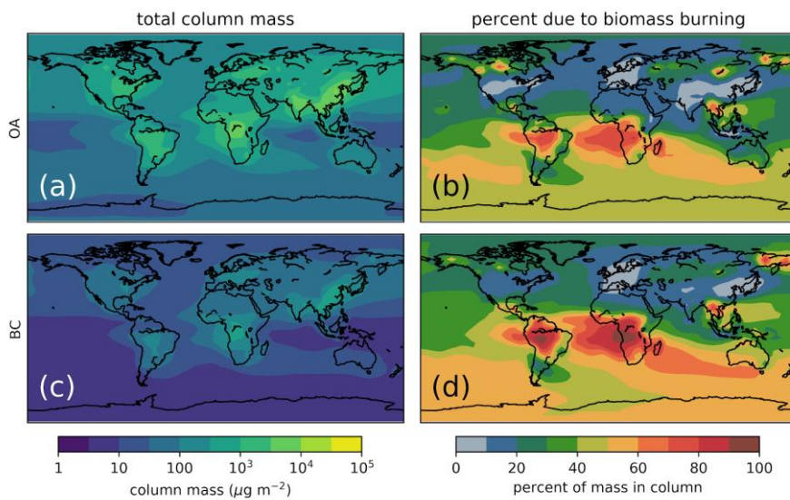
Figure S3S6: Effect of biomass burning on annually averaged total column OA and BC mass concentrations. The left side shows the total column mass concentration of (a) OA and (c) BC in the simulations with FINNV1 biomass burning emissions (i.e., noSubCoag_FINN ). The right side shows the percent of the mass in the column that is due to biomass burning emissions for (b) OA and (d) BC by taking the difference between the noSubCoag_FINN and noBB simulations.
