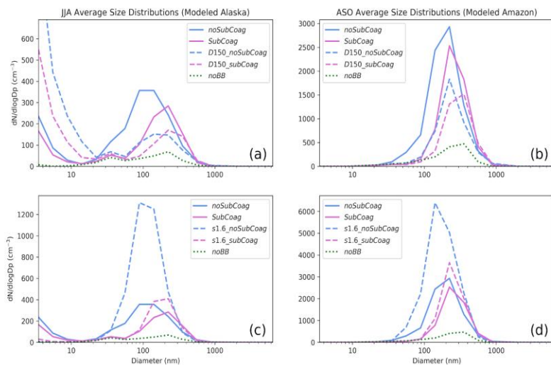
Figure 5: Predicted, grid-resolved surface-level aerosol size distributions with GFED biomass burning emissions over Alaska at 62^{\circ} N, 140^{\circ} W, averaged over the June, July, and August fire season (a and c) and the Amazon at 6^{\circ} S, 60^{\circ} E, averaged over the August, September, and October fire season (b and d). All panels show the size distributions for the noBB , noSubCoag , and SubCoag simulations in the dashed green, solid blue, and solid pink lines, respectively. The top panels (a and b) show the sensitivity to the emitted median diameter, and the bottom panels (c and d) show the sensitivity to the emitted modal width. Note the different y-axis scales.
