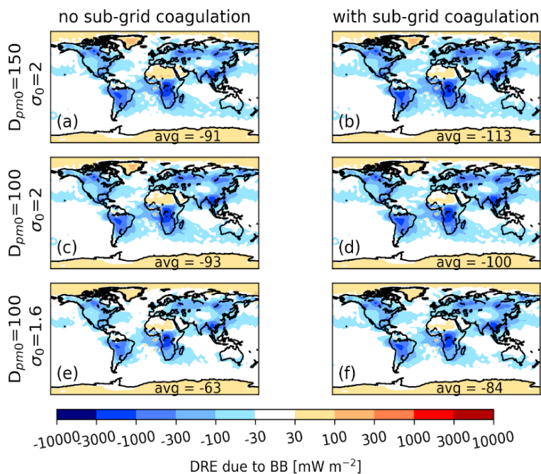
Figure S8S14: All-sky direct radiative effect (DRE) due to biomass burning aerosols using FINNv1 emissions and using the core-shell mixing assumption. Panels (a), (c), and (e) are without sub-grid coagulation ( D150_noSubCoag_FINN , noSubCoag_FINN , and s1.6_noSubCoag_FINN , respectively). Panels (b), (d), and (f) are with sub-grid coagulation ( D150_SubCoag_FINN , SubCoag_FINN , and s1.6_SubCoag_FINN , respectively). Panels (a) and (b) have an emitted median diameter of 150 nm and an emitted modal width of 2. Panels (c) and (d) have an emitted median diameter of 100 nm and an emitted modal width of 2. Panels (e) and (f) have an emitted median diameter of 100 nm and an emitted modal width of 1.6. The number in the bottom right of each panel is the global mean DRE value [ \text{mW m}^{-2} ].
