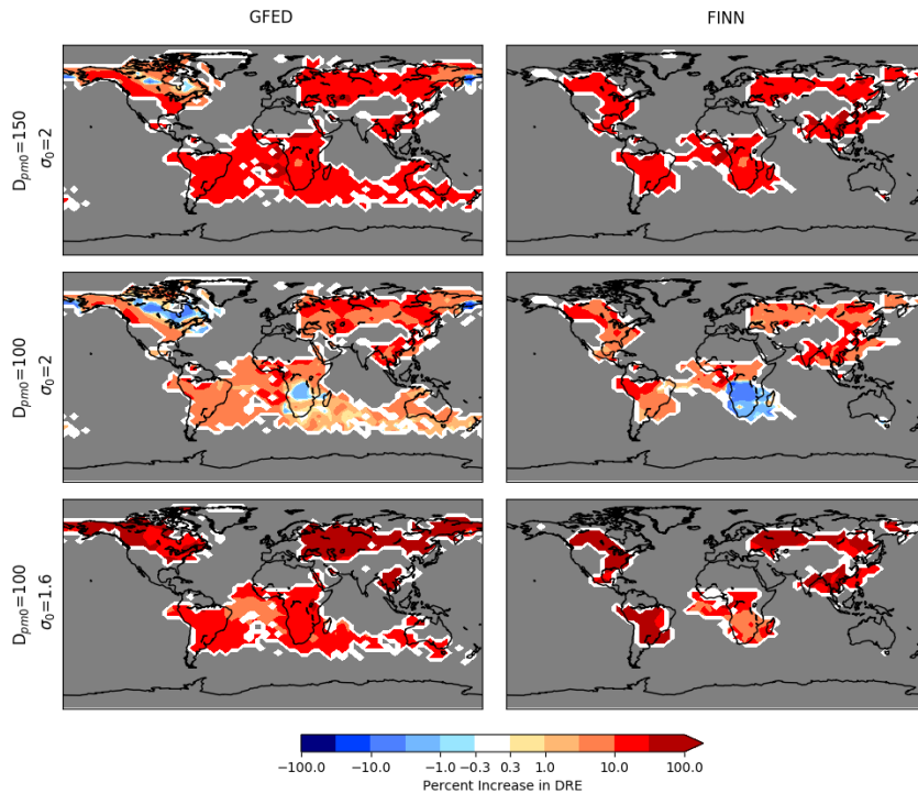
Figure S15: Percent change in all-sky direct radiative effect (DRE) of biomass burning aerosol due to sub-grid coagulation when using the core-shell mixing and GFED emissions (left) or FINNv1 emissions (right) and an assumed in-plume coagulation time of 24 hours. Panels in the top row have an emitted median diameter of 150 nm and an emitted modal width of 2. Panels in the middle row have an emitted median diameter of 100 nm and an emitted modal width of 2. Panels in the bottom row have an emitted median diameter of 100 nm and an emitted modal width of 1.6. Positive (red) values correspond to an increased cooling tendency of biomass burning DRE due to sub-grid coagulation being added. Regions in grey indicate that the DRE due to biomass burning is a more positive value than -100 \text{ mW m}^{-2} (i.e. there is less than 100 \text{ mW m}^{-2} of cooling) with or without sub-grid coagulation (see Figs. 8 and S14).
