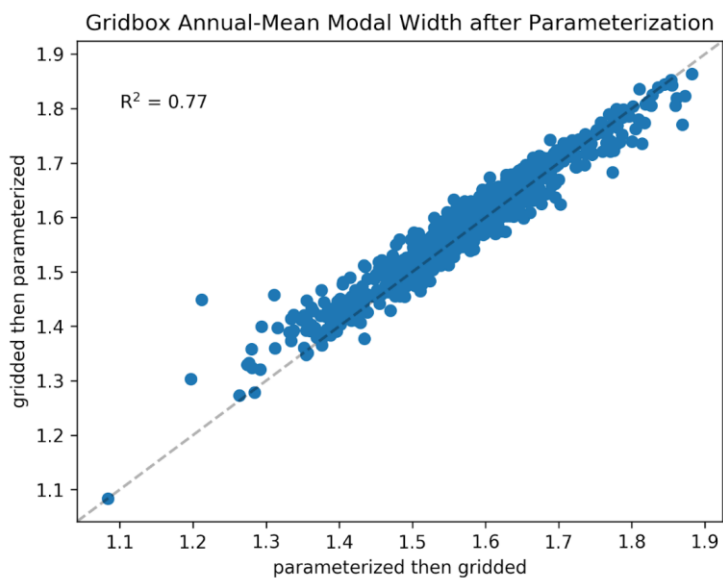
Figure S5: Annual-mean modal width for biomass burning emissions predicted for 2010 using the Sakamoto et al. (2016) parameterization after 24 hours of sub-grid coagulation with an emitted initial median diameter of 100 nm and an emitted initial modal width of 2. The y-axis shows the resulting lognormal modal width when the fire (FINNv1.5) and meteorological data is averaged over a 4°x5° grid and then that gridded data is run through the Sakamoto et al. (2016) parameterization (what we use in GEOS-Chem in this study). The x-axis shows the results when the individual fires are run through the Sakamoto et al. (2016) parameterization and then the output lognormal modal width is averaged over a 4°x5° grid. Each gridbox globally is represented as a point on the plot. The 1:1 line is in grey dash.
