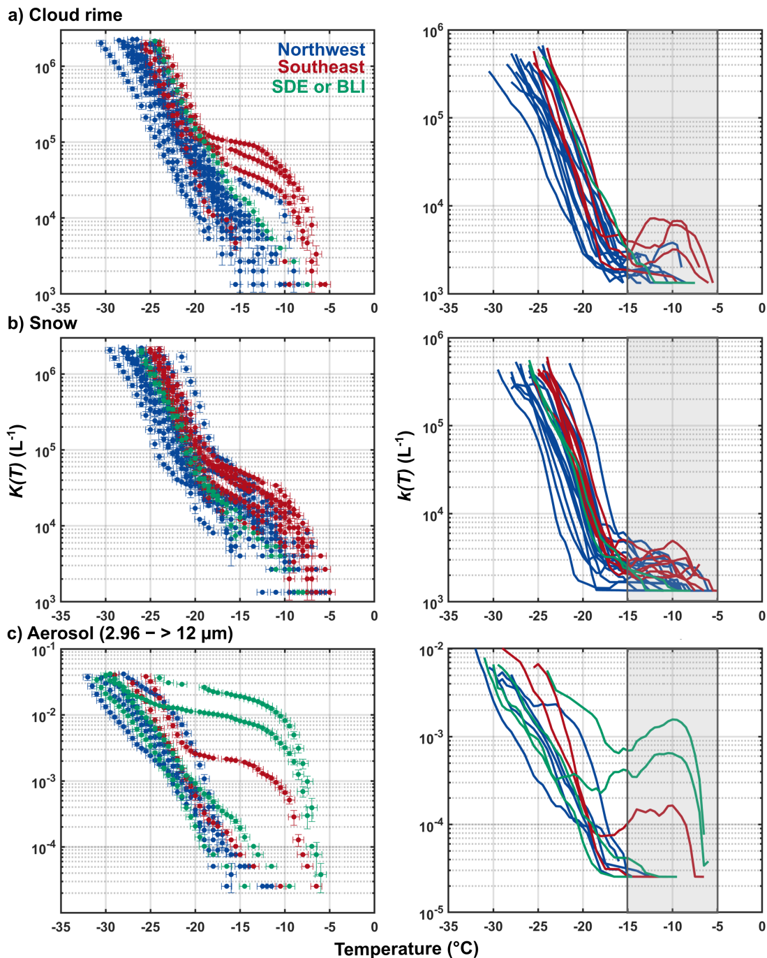
Figure 5. Cumulative INP spectra ( K(T) , on left) and differential INP spectra ( k(T) , on right) for the same samples of a) cloud rime, b) snow, and c) aerosol for the size range 2.96 – >12 μm in diameter. Spectra shown are for samples from the northwest (blue) and southeast (red) case study dates, in addition to SDE and boundary layer intrusion (BLI) case days (green). Multiple cloud rime and snow samples were collected while one aerosol sample from each size range was collected on northwest and southeast case study days (see Table 1). The warm mode region is indicated by the dark grey shading in the k(T) spectra. Note the axes are not all the same ranges.
