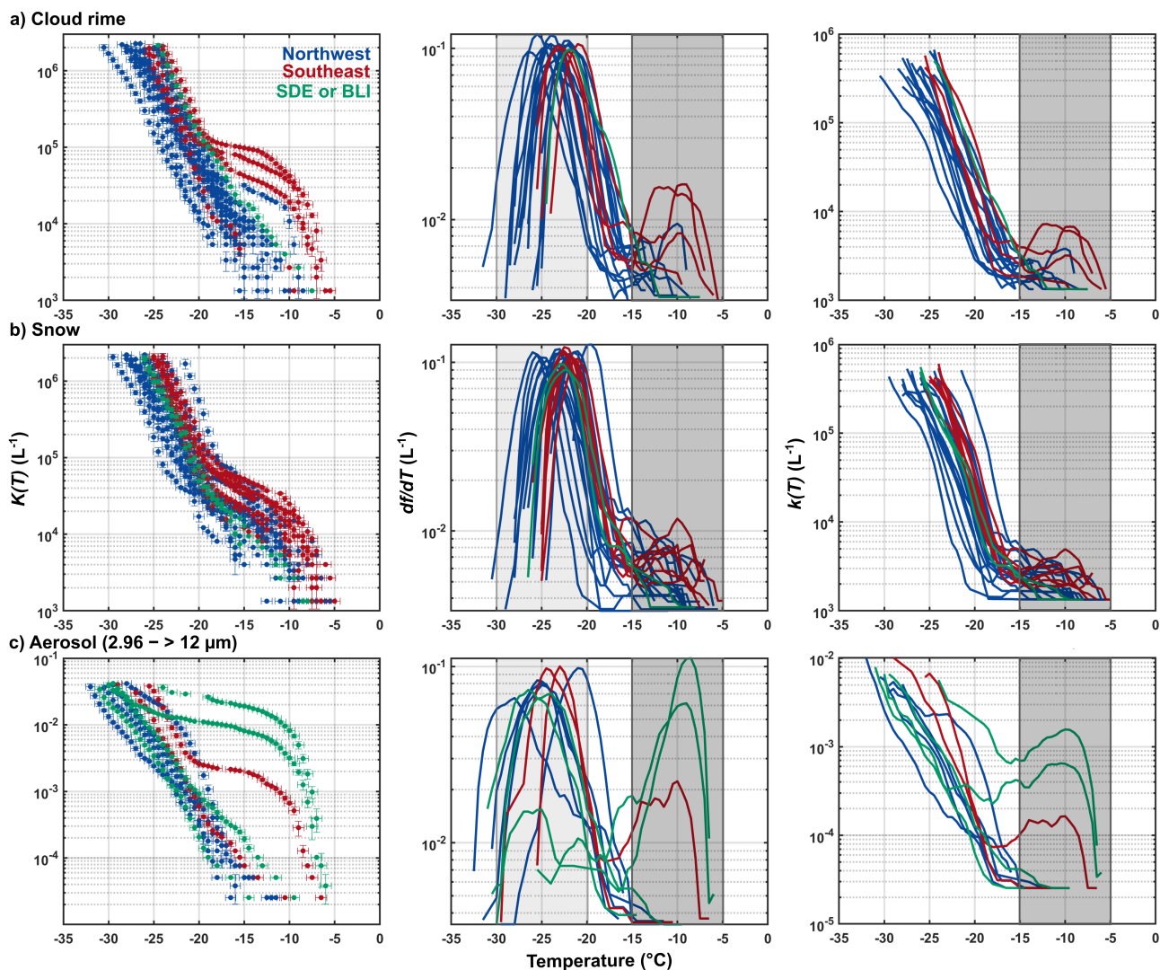
Figure 5. Cumulative INP spectra ( K(T) , on left), differential of fraction frozen per temperature interval ( df/dT ), and differential INP spectra ( k(T) , on right) for the same samples of a) cloud rime, b) snow, and c) aerosol for the size range 2.96 - >12 \mu\text{m} in diameter. Spectra shown are for samples from the northwest (blue) and southeast (red) case study dates, in addition to SDE and boundary layer intrusion (BLI) case days (green). Multiple cloud rime and snow samples were collected while one aerosol sample from each size range was collected on northwest and southeast case study days (see Table 1). The warm mode region is indicated by the dark grey shading in both the df/dT and k(T) spectra, while the cold mode region (for df/dT only) is shown in the df/dT spectra.
