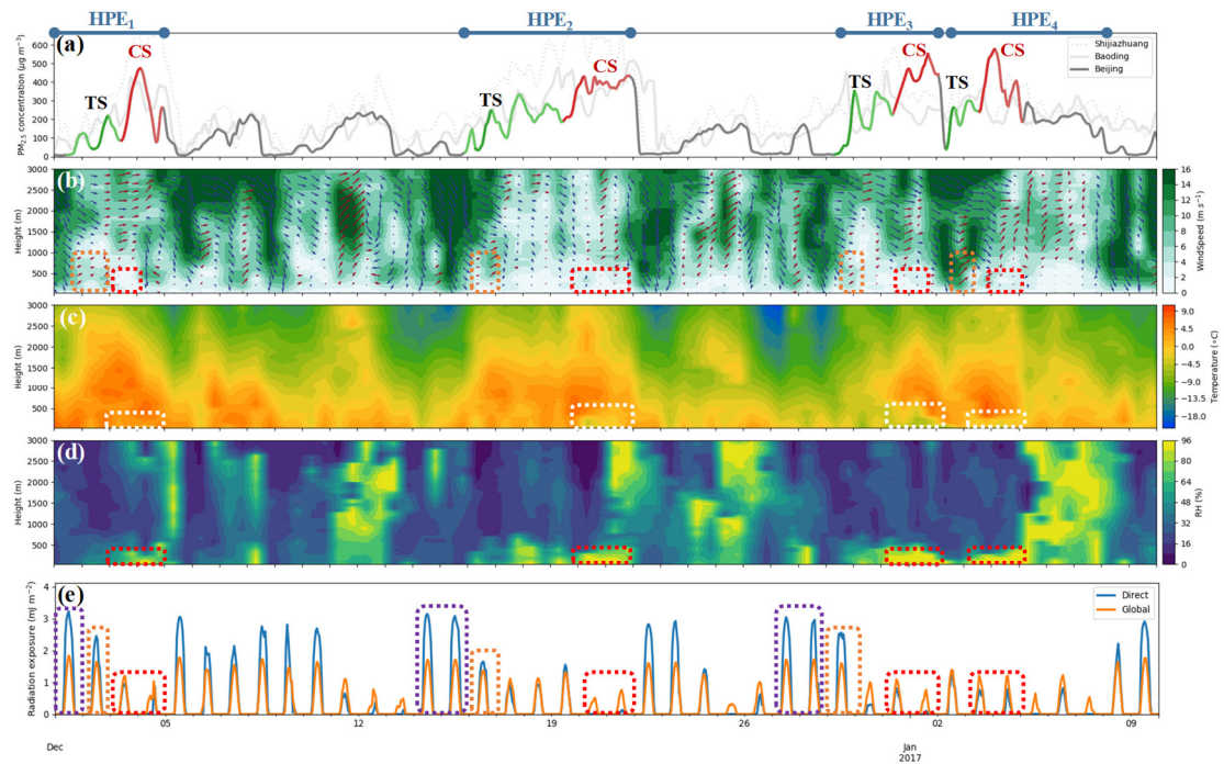
Figure S1: Temporal variations in PM 2.5 , surface radiation, and vertical distributions of meteorological factors from December 1, 2016 to January 10, 2017. (a) PM 2.5 mass concentration (gray or colored line: Beijing; light gray line: Baoding; gray dot: Shijiazhuang); (b) winds (vectors) and wind velocity (shadings; units: m s -1 ); (c) temperature (shadings; units: °C); (d) RH (shadings; units: %); and (e) global radiant exposure. (Blue line: HPEs; green line and orange box: TSs; red line and white or red box: CSs; purple box: clean periods)
