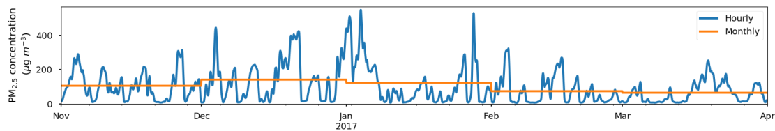
Fig. 1. The time series of PM 2.5 mass concentration in the urban area of Beijing
