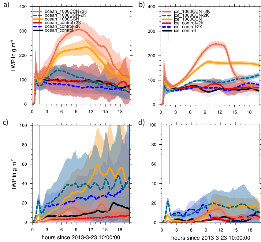
Figure 10. Domain averaged a,b) LWP and c,d) IWP over the open ocean (left) and sea ice (right) in control and the respective 1000CCN simulations in their regular state and 2 K warmer and colder conditions. The solid lines depict the means, the shadings the standard deviations. The vertical black lines indicate the CCN perturbation injections.
