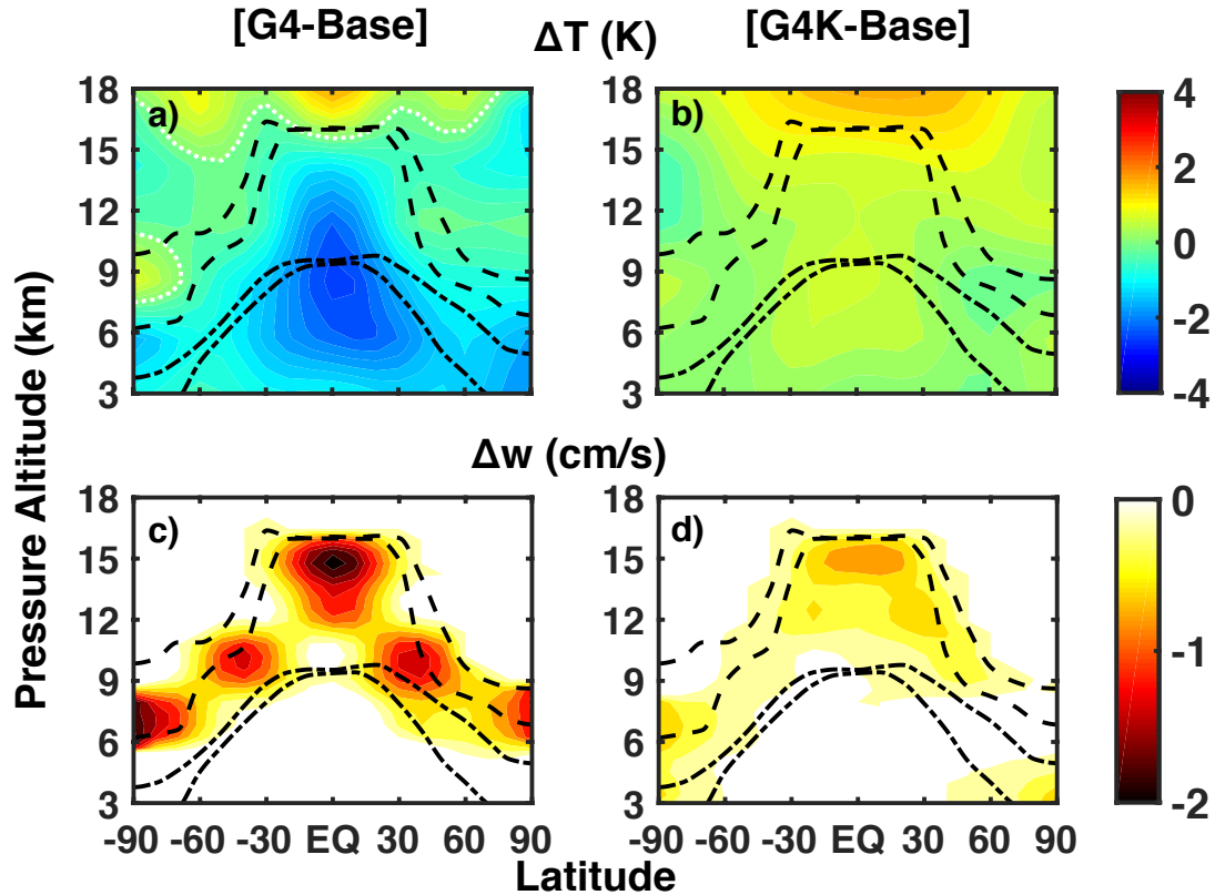
Figure 7. Zonally and time-averaged changes of temperature (panels a,b) and vertical velocity (panels c,d) in experiments G4 (panels a,c) and G4K (panels b,d) with respect to the Base case (years 2030-69). The dashed lines show the mean tropopause height (with seasonal variability). The dash-dotted lines show the mean height at which T=238 K (with seasonal variability). The dotted white lines in panel a) highlights where \Delta T=0 K.
