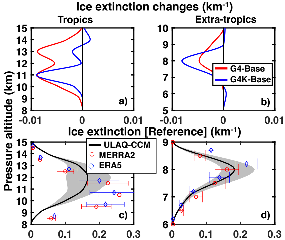
Figure 12. Average upper tropospheric profiles of ice particle extinction ( \lambda=0.55 \mu\text{m} ) ( \text{km}^{-1} ) for the tropics (25S-25N) and extratropics (35S-90S, 35N-90N) in panels (a,c) and (b,d), respectively. Panels (a,b): ice extinction changes for G4-Base (red curves) and G4K-Base (blue curves) (years 2030-69). Panels (c,d): comparison of ULAQ-CCM calculated values of ice extinction with indirectly derived values from the MERRA-2 and ERA5 ice mass mixing ratio and ULAQ-CCM effective radius (red and blue circles) (see text). The time average is over the years 2003-2012. The shaded areas represent \pm 1 \sigma for the ensemble over the 10-year period.
