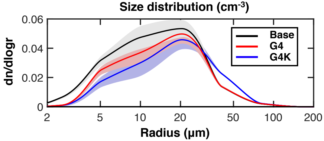
Figure 10. Globally and time-averaged number density values of ice crystals as a function of particle radius ( dn/d\log r , \text{cm}^{-3} ) (years 2030-69). Shaded areas of the same colour represent \pm 1 \sigma for the ensemble over the 40-year period 2030-69. The calculated global mean values of the ice particle effective radius are as follows: Base \rightarrow 31.2 \pm 3.2 \mu\text{m} ; G4 \rightarrow 33.5 \pm 3.6 \mu\text{m} ; G4K \rightarrow 36.8 \pm 4.1 \mu\text{m} . The reference MODIS value in Table 2 is 33.4 \pm 2.1 \mu\text{m} .
