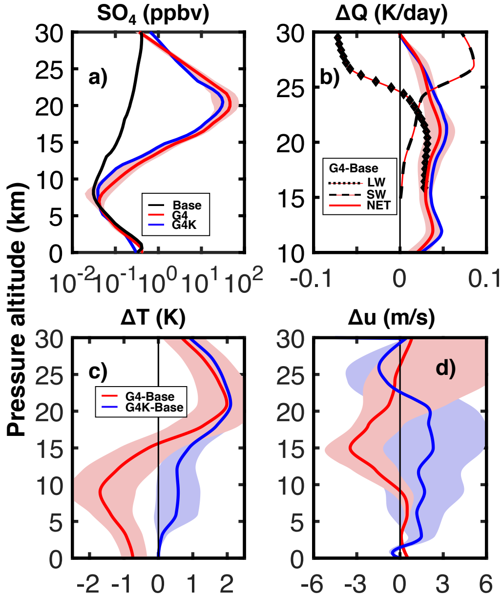
Figure 9. Average tropical vertical profiles (25S-25N, years 2030-69) of the SO 4 volume mixing ratio for G4, G4K and Base experiments (ppbv, panel a); G4-Base changes of net, shortwave and longwave heating rates (K/day, panel b) (LW is calculated with temperature fixed at Base values) (net heating rate changes are also shown for G4K-Base, with the blue line); G4-Base and G4K-Base temperature changes (K, panel c); G4-Base and G4K-Base changes of mean zonal winds (m/s, panel d). The shaded areas of the same colour represent \pm 1 \sigma for the ensemble over the 40-year period 2030 to 69.
