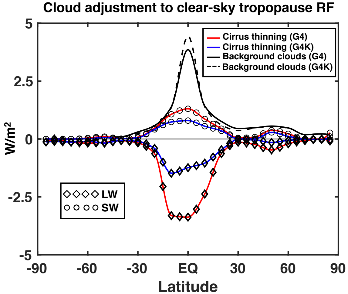
Figure 14. Zonally averaged cloud adjustments to the clear-sky SG aerosol RF ( \text{W/m}^2 ), as a function of latitude (time average 2030-2069). See legends for line meaning. The positive adjustment due to (passive) background clouds (black solid line for G4, black dashed line for G4K) shows the net value (SW+LW), which is, however, largely controlled by the SW contribution (see Table 4 and Fig. S3).
