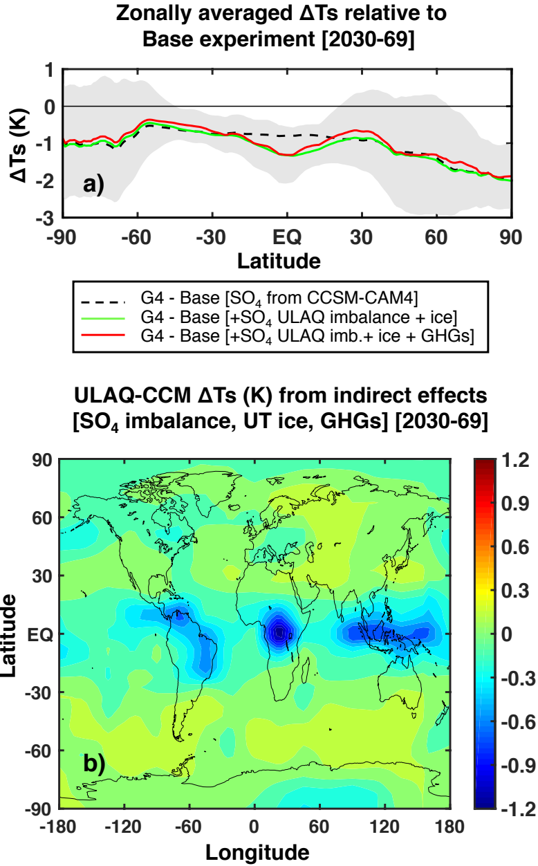
Figure 6. Panel (a): zonally averaged T_s anomalies G4-RCP4.5 (K), under different conditions for the G4 perturbed case (time average 2030-69): from the atmosphere-ocean coupled model CCSM-CAM4 (black dashed line); as above, but adding the T_s anomalies in the ULAQ-CCM with on-line coupling of cirrus ice changes and the SO_4 imbalance between CCSM-CAM4 and ULAQ-CCM (green line); as above, but adding also the T_s anomalies in the ULAQ-CCM with on-line coupling of GHG changes (red line) (see text and legend). The shaded area represents \pm 1 \sigma of the zonally averaged T_s over the 40-year period. b) Lat-lon distribution of the T_s anomalies (K) calculated on-line in the ULAQ-CCM model considering cirrus ice changes, the SO_4 imbalance between CCSM-CAM4 and ULAQ-CCM and GHG changes (time average 2030-2069).
