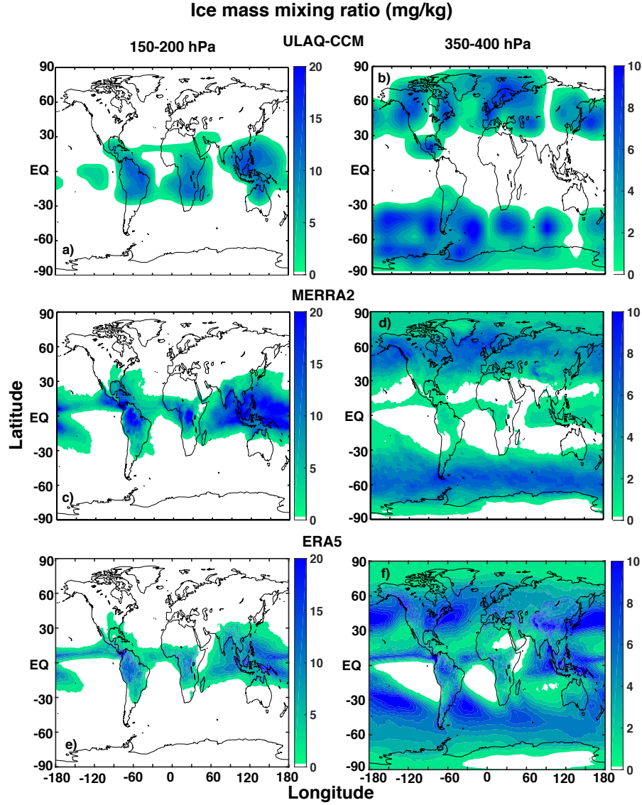
Figure 1. Lat/lon maps of the ice mass mixing ratio (mg/kg-air) for pressure layers representative of tropical (panels a,c,e) and extratropical (panels b,d,f) upper troposphere. Panels (a,b) are for the ULAQ-CCM; panels (c,d) are for MERRA-2 data (Bosilovich et al. (2017)); panels (e,f) are for ERA5 data (Stephens et al. (2000)). Time average is on years 2003-2012.
