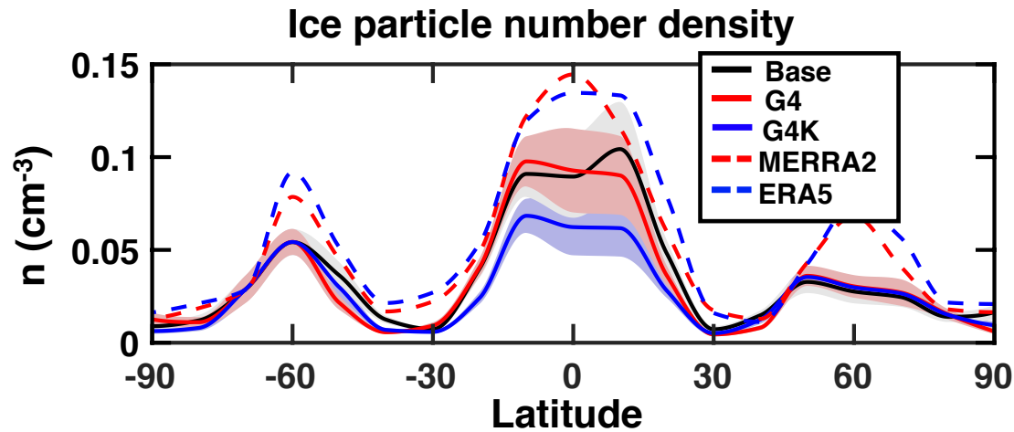
Figure 11. Zonally and time-averaged total number density values of ice crystals as a function of latitude ( n , \text{cm}^{-3} ) (years 2030-69), as calculated in the ULAQ-CCM (for Base, G4, G4K experiments) and compared with indirectly derived values from the MERRA-2 and ERA5 ice mass mixing ratio and ULAQ-CCM (Eq. 4). Number densities are calculated at pressure layers 150-200 hPa for 25S-25N, 200-250 hPa for 25-35 (N/S), 250-300 hPa for 35-45 (N/S), 300-350 for 45-55 (N/S) and 350-400 for 55-90 (N/S).
