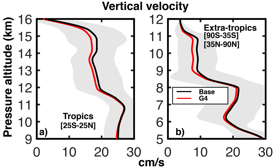
Figure 8. Average upper tropospheric profiles of the vertical velocity (cm/s) in G4 and Base experiments (years 2030-69). Panels (a) and (b) are for the tropics and extratropics, respectively (see legends). The vertical velocity w is obtained as the sum of the large-scale value and that calculated as a function of the TKE (see Lohmann and Karcher (2002) and Eq. 5), which essentially accounts for the synoptic scale and gravity wave motions. The shaded areas of the same color represent \pm 1\sigma for the ensemble over the 40-year period 2030 to 69.
