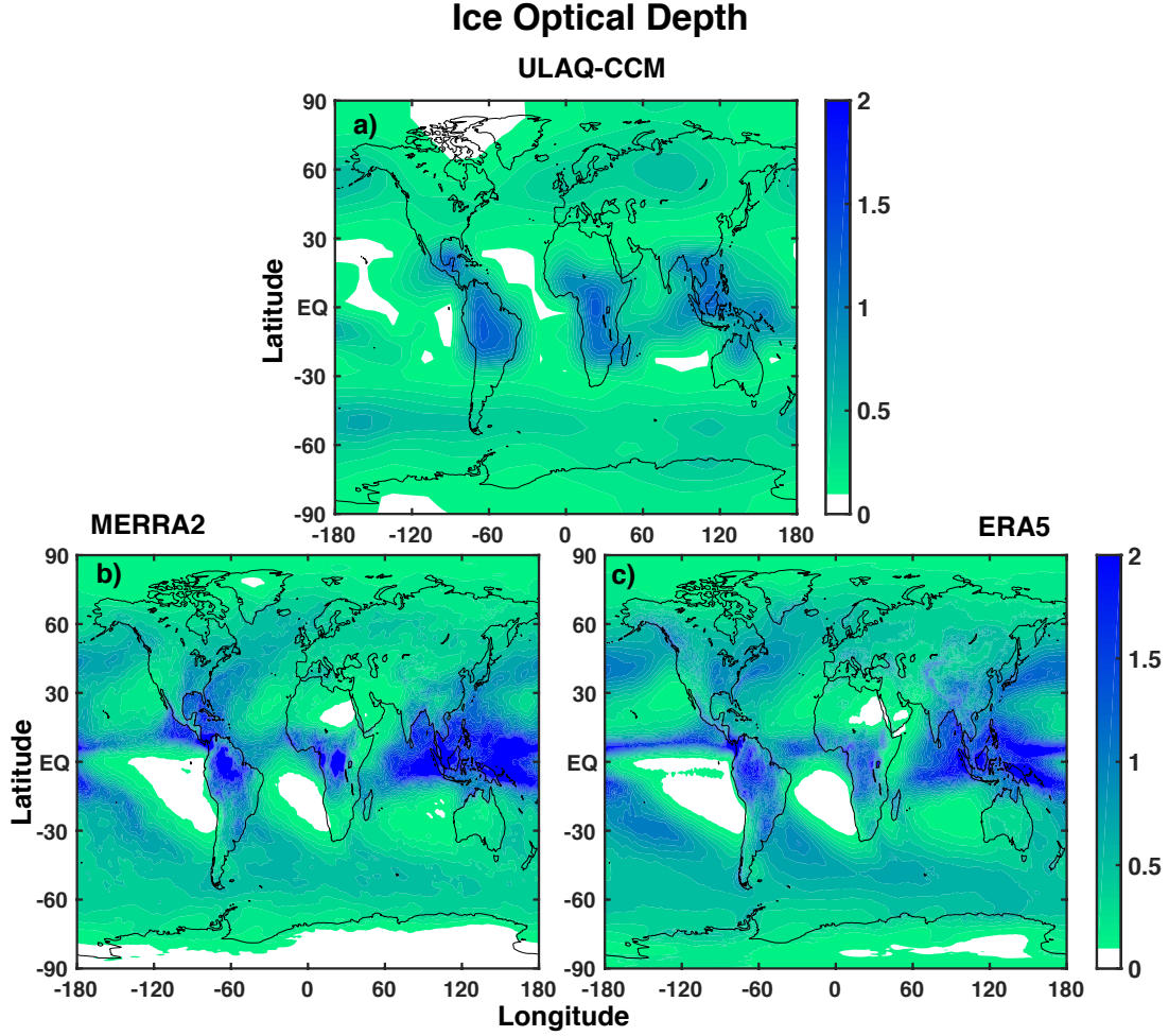
Figure 2. Ice optical depth at \lambda=0.55 \mu\text{m} , from ULAQ-CCM calculations (a) and from the MERRA-2 (b) and ERA5 (c) ice mass mixing ratio ( 100 < p < 450 \text{ hPa} ), with ULAQ-CCM particle effective radius. Time is averaged over the years 2003-2012.
