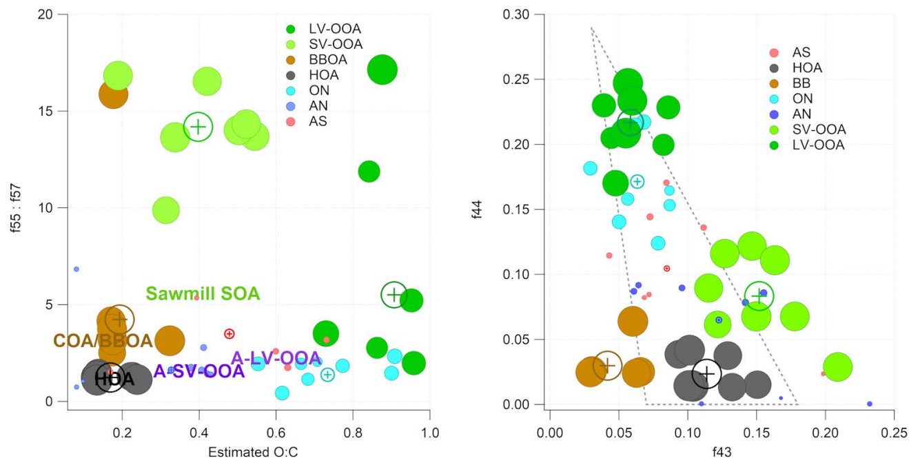
Figure 7. (Left panel:) P-III (r-CMB) solution - cluster projections onto a f_{55}/f_{57} (Mohr et al., 2012), O:C (estimated, Aiken et al., 2008) plane. Circles correspond to the members of the cluster and the cross markers to cluster centroids. The text markers indicate
