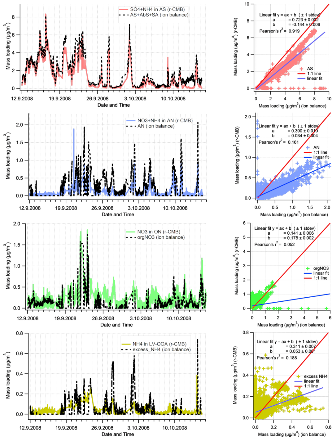
Figure 10. Comparison of Inorganics apportionment methods (r-CMB and ion balance scheme). The estimates from the ion balance scheme (Section 2.4.1) are shown in black, and the r-CMB model results in colour. The linear fits (right panels) represent the data poorly due to high amount of zero-value points and outliers.
