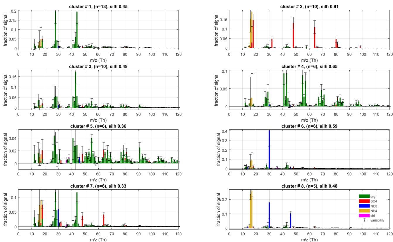
Figure 3. The 8 largest clusters for P-I classification of factorisation results. Cluster centroids (coloured bars) and variabilities (error bars) are silhouette-weighted averages and standard deviations for the cluster members. The main anthropogenic aerosol types were identified as Clusters #2 (‘Ammonium sulfate’, AS), #4 (‘Hydrocarbon-like organic aerosol’, HOA), #5 (‘Biomass burning organic aerosol’, BBOA) and #8 (‘Ammonium nitrate’, AN). Cluster number, silhouette and population (n) are shown in panel titles.
