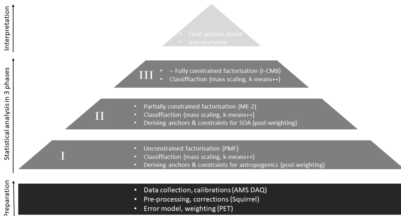
5 Figure 2. A flowchart illustrating the analysis using combined methodology. After initial data collection and preparation, statistical analysis is performed in three phases (P-I to P-III). Each phase limits the freedom given to factorisation from completely free (PMF) to nearly fully constrained (r-CMB). Finally, we evaluate and interpret the r-CMB model from an aerosol chemical perspective.
