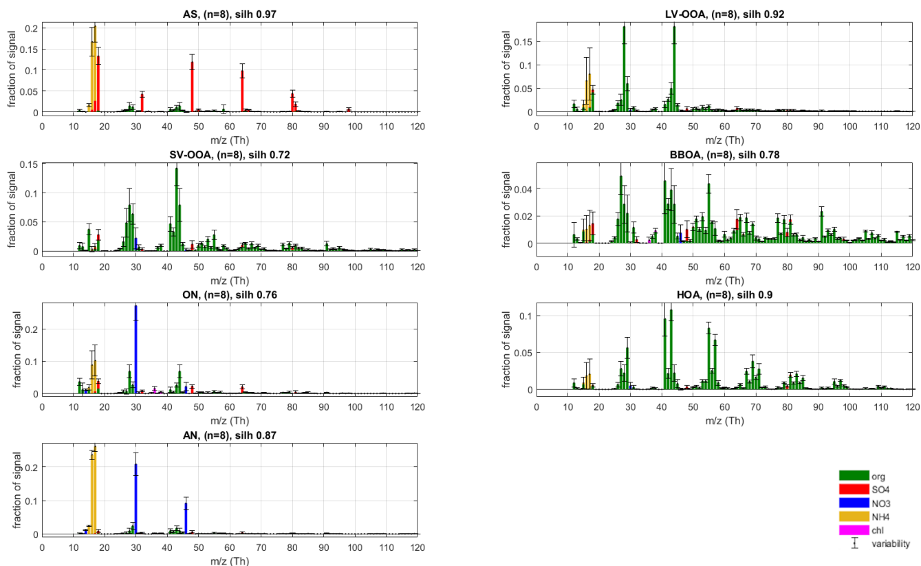
15 Figure 4. Final silhouette-weighted reference spectra (coloured bars) and variabilities (error bars) for the r-CMB model components.
