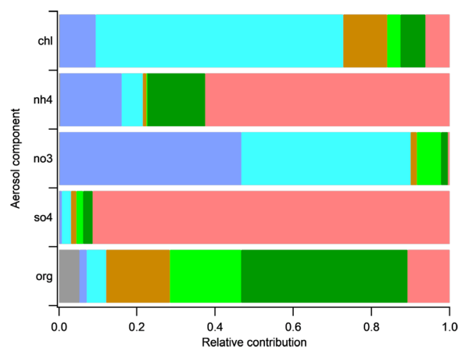
5 Figure 5. “Default” chemical speciation for r-CMB components; mass loadings (upper left) and relative contributions (upper right) of default species in components. Apportionment of default species to r-CMB components by mass (lower left) and relative contribution (lower right).
