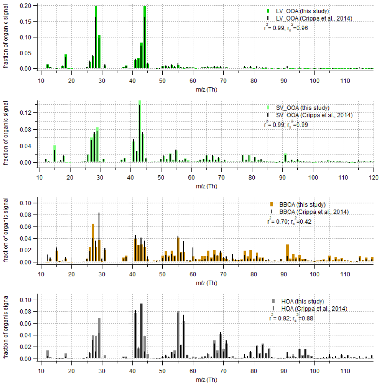
Figure 9. Comparison of organic part of spectra with Crippa et al. (2014) for data set II. The r-CMB model results from this study are shown in colour, and the Crippa et al. spectra in black. For comparability, the Crippa et al. spectra were corrected for a difference in fragmentation tables used (included m/z 28 Th, updated to modern calculation of m/z 16, 17 and 18 Th organic signals) and total signal subsequently re-normalised to unity. Spectra similarity is evaluated using Pearson's squared correlation coefficients; unscaled ( r^2 ) and with mass scaling ( r_s^2 ).
