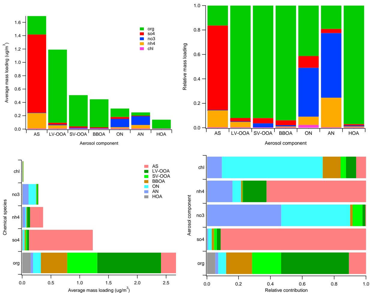
5 Figure 5. “Default” chemical speciation for r-CMB components; mass loadings (upper left) and relative contributions (upper right) of default species in components. Apportionment of default species to r-CMB components by mass (lower left) and relative contribution (lower right).
