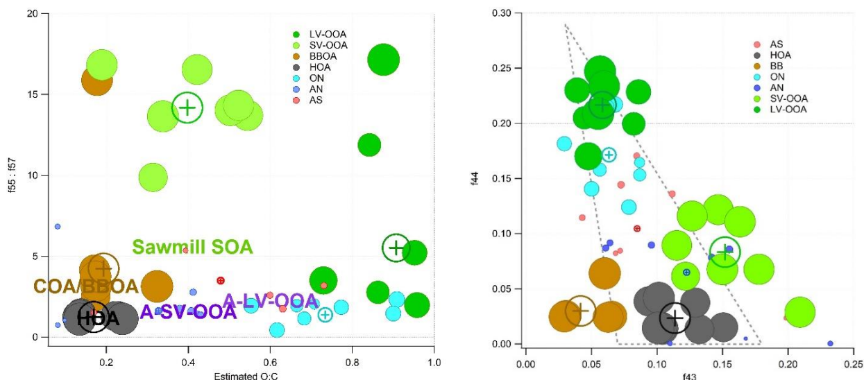
5 Figure 7. (Left panel:) P-III (r-CMB) solution - cluster projections onto a f55/f57 (Mohr et al., 2012), O:C (estimated, Aiken et al., 2008) plane. Circles correspond to the members of the cluster and the cross markers to cluster centroids. The text markers indicate respective positions of anthropogenic organic aerosol types from Äijälä et al. (2017). Marker size indicates organic mass fraction in spectra. Axes are truncated. (Right panel:) P-III solution, projected onto f44, f43 plane (i.e. the ‘Sally’s triangle’ plot; Ng et al., 2011). Circles correspond to objects in cluster and the cross markers to cluster centroids. Marker size indicates organic mass fraction in spectra. Dotted line marks the area where most laboratory data for organic aerosol falls (Ng et al., 2010).
