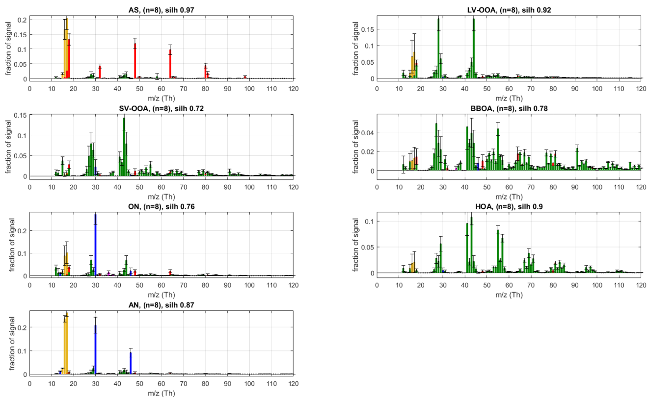
5 Figure 4. Final silhouette-weighted reference spectra and variabilities for the r-CMB model components. (red: SO 4 ; blue NO 3 ; orange: NH 4 ; magenta: chlorides; green: org)
