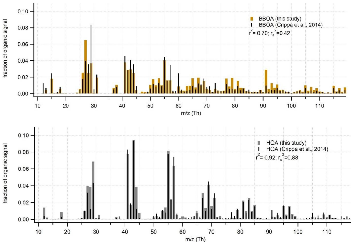
5 Figure 9. Comparison of organic part of spectra with Crippa et al. (2014) for data set II. The r-CMB model results from this study are shown in colour, and the Crippa et al. spectra in black. For comparability, the Crippa et al. spectra were corrected for a difference in fragmentation tables used (included m/z 28 Th, updated to modern calculation of m/z 16, 17 and 18 Th organic signals) and total signal subsequently re-normalised to unity. Spectra similarity is evaluated using Pearson's squared correlation coefficients; unscaled ( r^2 ) and with mass scaling ( r_s^2 ).
