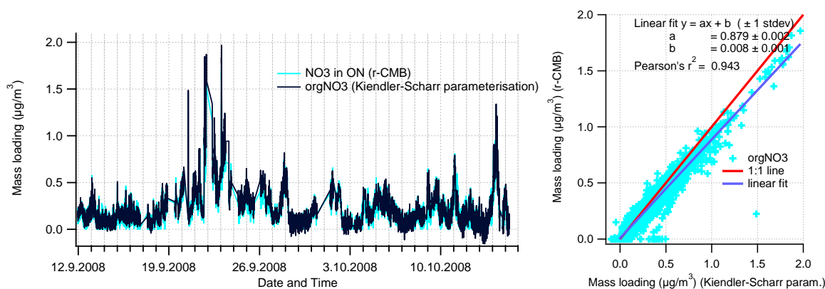
Figure 11. Comparison of Kiendler-Scharr parametrization (Kiendler-Scharr et al., 2016; black line; moving median filter for 11 points window applied; R_{\text{calib}} = 0.42 , R_{\text{orgNO}_3} = 0.1 ) for organonitrate with NO 3 ion species in ON factor from our r-CMB model (in colour).
