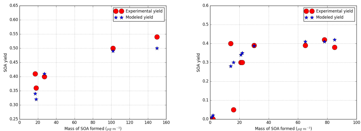
Figure 4. SOA experimental and modeled yield data from smog chamber for guaiacol under low- \text{NO}_x conditions (left panel) (experimental data from Chhabra et al. (2011); Yee et al. (2013) and under high- \text{NO}_x conditions (right panel) (experimental data from Yee et al. (2013); Lauraguais et al. (2012))
