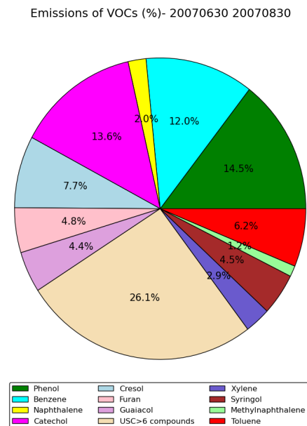
Figure 7. Emissions of the OA_{tot} precursors from wildfires for the different sensitivity simulations (left panel) and percentage of emissions for each VOC (right panel) over the subregion during the summer 2007.
