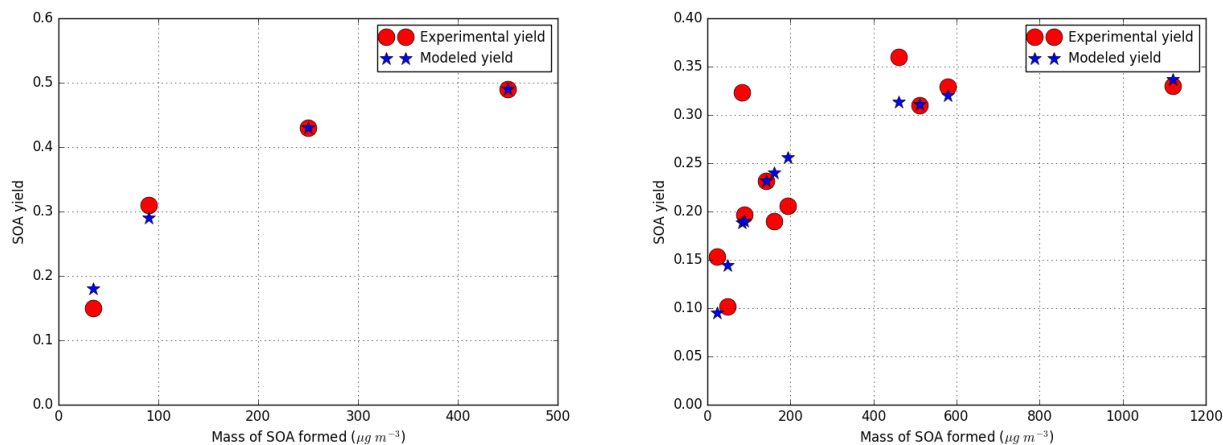
Figure 3. SOA experimental and modeled yield data from smog chamber for syringol under low- \text{NO}_x conditions (left panel) (experimental data from Chhabra et al. (2011); Yee et al. (2013) and under high- \text{NO}_x conditions (right panel) (experimental data from Yee et al. (2013); Lauraguais et al. (2012))
