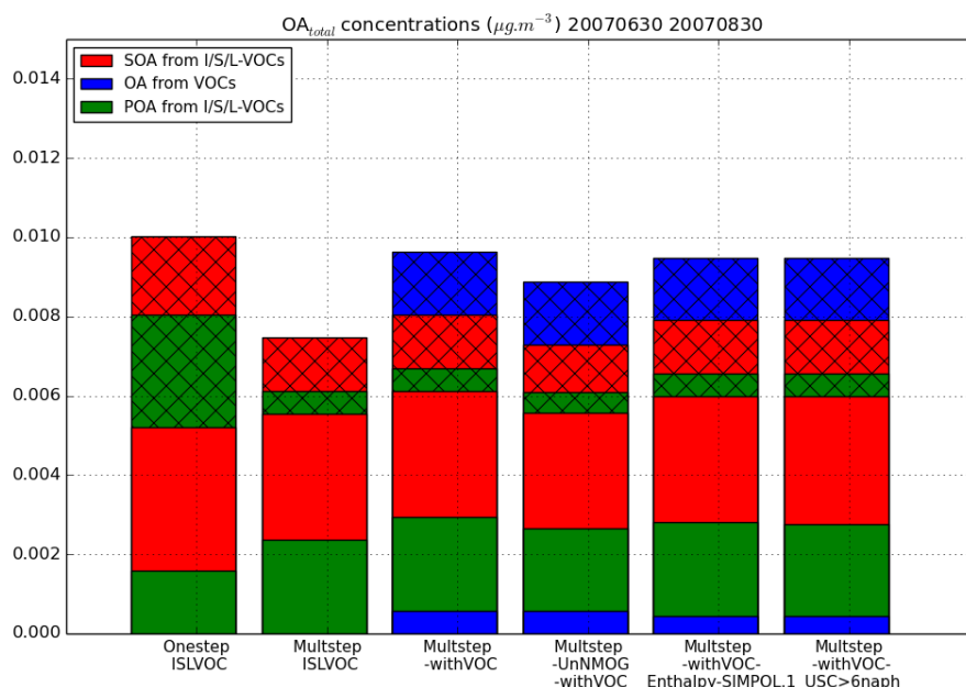
Figure 10. Mean surface \text{OA}_{tot} concentrations from different \text{OA}_{tot} precursors over the subregion for each sensitivity simulation.
