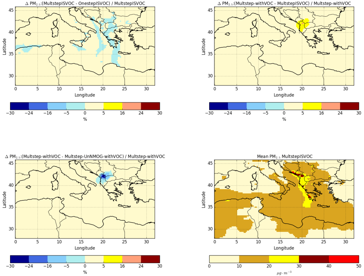
Figure 13. Sensitivity of surface PM_{2.5} concentrations to the gaseous I/S/L-VOCs ageing scheme (upper left panel), the SOA from the selected VOC (upper right panel), the SOA from gaseous I/S/L-VOCs emissions estimated from NMOG (lower left panel) and daily mean PM_{2.5} concentrations from the Multistep - withVOC simulation (lower right panel) during the summer 2007 (from 30 June to 30 August 2007).
