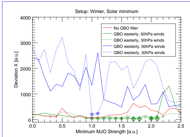
Figure S15: As Fig. 6 in the manuscript, but including results for which the QBO filtering was based on the 30 hPa winds instead of the 50 hPa winds. It is obvious that the choice of the pressure level, at which the wind data is evaluated to define the QBO state, does qualitatively not influence the conclusions.
