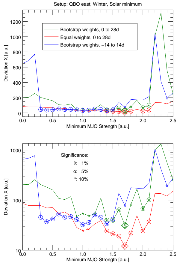
Figure 5. Calculated deviations X between indicating the empirical time lags to strength of the statistical connection between the solar trigger, at which 27-day cycle and the individual MJO phases occur maximally, and phase evolution; a fitted sawtooth function lower X indicates a stronger connection. The same data is shown in linear scaling (upper panel) for an overall visual impression and in logarithmic scaling (lower panel) for inspection of the smaller variations. According to our analysis approach, a lower deviation represents a stronger statistical connection between the solar 27-day cycle and the MJO phase evolution. Focus of this experiment is the dependence of the deviation on the MJO strength threshold. The green line shows these results for the standard numerical setup ( epoch time lags from 0 to 28 d and squared weights from the bootstrap approach ). Three levels of significance in the sense of the MC experiment are shown: 10%, 5%, or 1% chance of getting lower deviations with randomly modified solar extremum dates. The other two lines give an impression of the reaction of the results when the numerical setup is changed to, first, a different epoch definition (blue line) or, second, the use of constant weights (red line, see text Sect. 4.2 for details).
