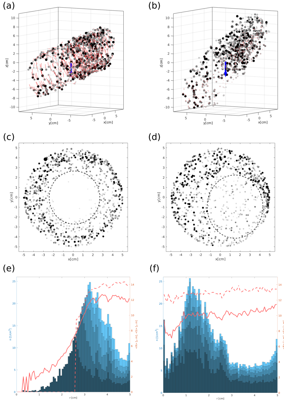
Figure 6. Positions of droplets in simulations 1) (left column) and 2) (right column) as described in Table 5 in perspective view (panels a and b) and in 4 cm-thick central slice projected on a plane perpendicular to the vortex axis (panels c and d). The blue arrow shows the direction of gravity. In panels a-d, droplet size and colour are scaled respectively to the rules described in Sec.5. The red tracks behind the particles in panels a and b reflect the last \Delta t = 0.0055 s of the droplet trajectory (for clarity every 10th droplet is drawn). The dashed circles in panels c and d reflect the approximate shape and size of the visible void in the droplet field. Panels e and f present: the number concentration of droplets n with different blue shading colors representing the contribution from different size groups - left axis, droplet mean real radius (solid red line) and mean visible radius (dashed red line) - right axis, all with respect to the distance from the vortex axis r .
